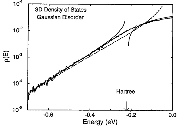
FIG. 1. Density of states (in \text{eV}^{-1} ) for a tight-binding model on a cubic lattice in the presence of a random potential with Gaussian statistics. Histogram: data from the numerical simulation. Full curves: instanton after Hartree resummation (left part), Hartree summation inside the band (right part). Dashed curve: bare instanton theory. The effect of the resummation can be clearly seen. No fitting was done.
