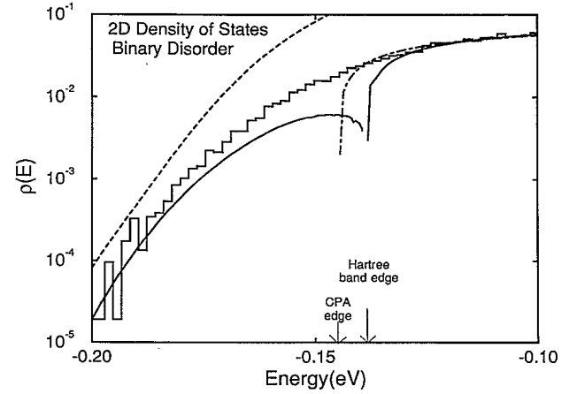
FIG. 3. Density of states (in \text{eV}^{-1} ) for a tight-binding model on a square lattice with binary disorder. Histogram: data from the numerical simulation. Dashed curve: bare instanton theory. Full curves: instanton after Hartree resummation (left part), Hartree summation inside the band (right part). Dotted-dashed curve: CPA prediction, only present in the band.
