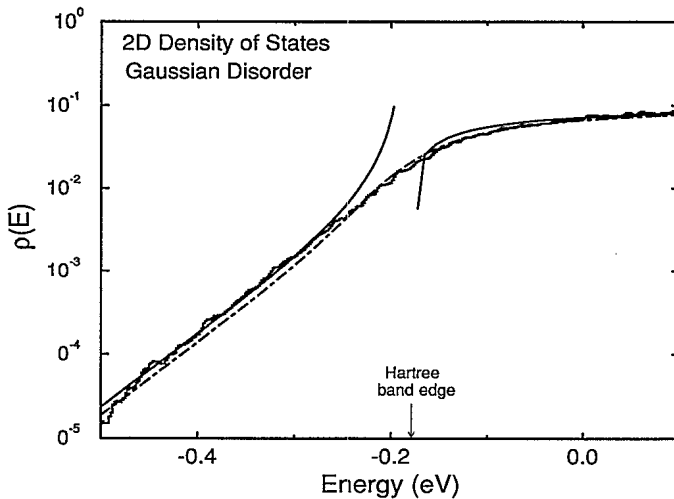
FIG. 2. Density of states (in \text{eV}^{-1} ) for a tight-binding model on a square lattice in the presence of a random potential with Gaussian statistics. Histogram: data from the numerical simulation. Full curves: instanton after Hartree resummation (left part), Hartree summation inside the band (right part). Dotted-dashed line: CPA prediction. The CPA performs very well in the case of Gaussian disorder.
