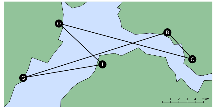
Fig. 1. The six over-water links in the Tegola network.
