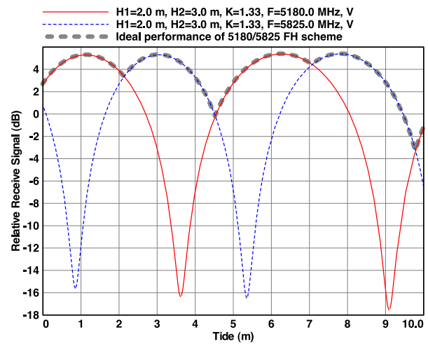
Fig. 8. Modelling of tidal fading when operating at 5180MHz and 5825MHz for the Ornsay-Corran link. The fading that would be experienced by a slow frequency hopping system using these two frequencies is also shown.
