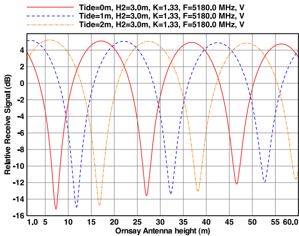
Fig. 7. Path loss simulated using CTE Pathloss 4.0 for varying height of the Ornsay antenna on the Ornsay-Corran link. The graph shows that nulls occur approximately every 20 m.
