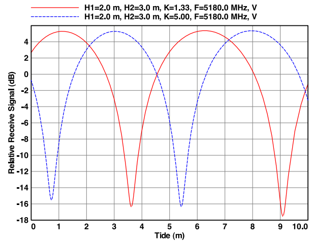
Fig. 6. Signal strength against tide height for the Ornsay–Corran link, simulated using CTE Pathloss 4.0. H1 and H2 refer to the heights of the antennas above land height, as determined by the link profile — the antenna heights can be very low as they are positioned on the sides of hills.
