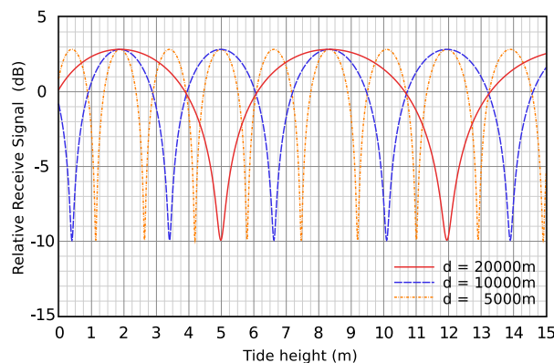
Fig. 4. Relative received signal strength vs. tidal height for links with both antennas 50m above sea level calculated using the geometric model with three link lengths. The reflection coefficient is 0.9. The frequency of operation is 5.180GHz (at 2.4GHz the null spacing would approximately double). Atmospheric effects and earth curvature are neglected.
