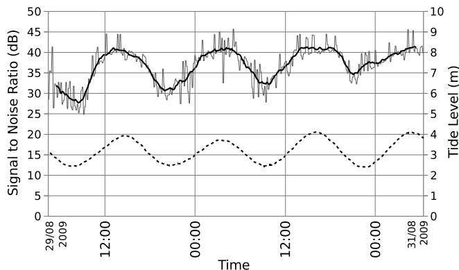
Fig. 2. Signal strength data collected from the Ormsay–Corran link in the Tegola network — the thin (thick) line corresponds to measured signal strength (two hour box-car average). The dashed line shows the tide height data as recorded at a nearby location (Ullapool) for the same time period.
