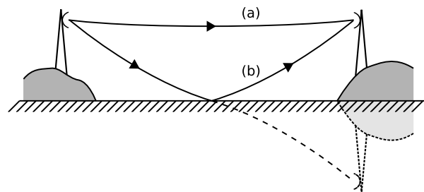
Fig. 3. The two ray model, showing (a) the direct path and (b) the indirect path reflected off the water plane. The reflected path is longer, and so may interfere destructively with the direct path. Refraction is neglected in this diagram. The ray paths are curved due to the flat-earth representation used to clarify the reflection.
