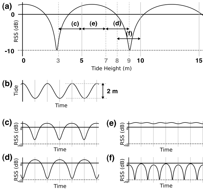
Fig. 5. Modelling the effect of the tide-RSS transfer function on four tidal variations of 2 m. (a) A typical transfer function. (b) The simulated tidal variation. (c) A “positive” response, where increase in tidal height results in increased signal strength. (d) A “negative” response, where increase in tidal height results in decreased signal strength. (e) A “flat” response, where the signal strength is stable to within approximately 2 dB throughout the tidal cycle. (f) A “cross-null” response, which has two minima for every tidal period.
