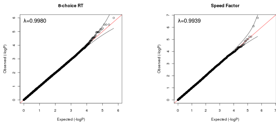
Supplementary Figure 1. Q-Q plots (and their 95% confidence intervals) and Lambda ( \lambda ) Values for the Reported Measures: Digit Symbol, Symbol Search, Inspection Time, Simple RT, Choice RT Measures and the Speed Factor.
