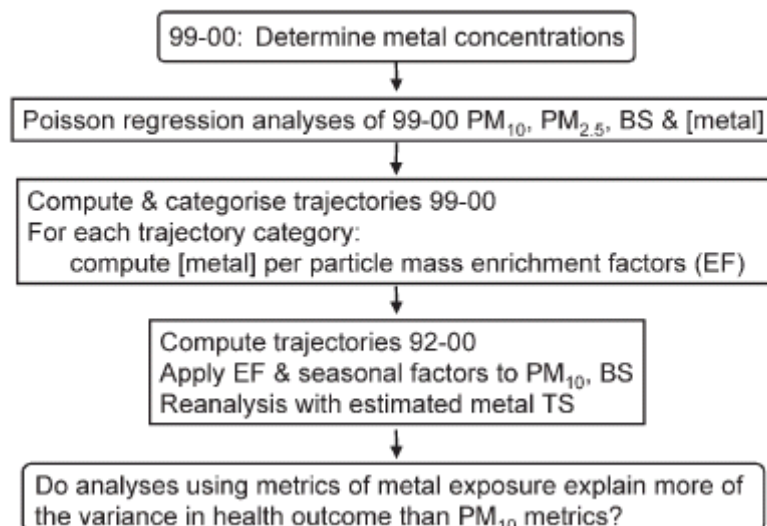
Fig. 1. Conceptual overview of the project to apply chemical exposure data to epidemiological time series analyses of population health outcome. The prior hypothesis was that metal enrichment factors (EF) would be significantly different for some air mass
