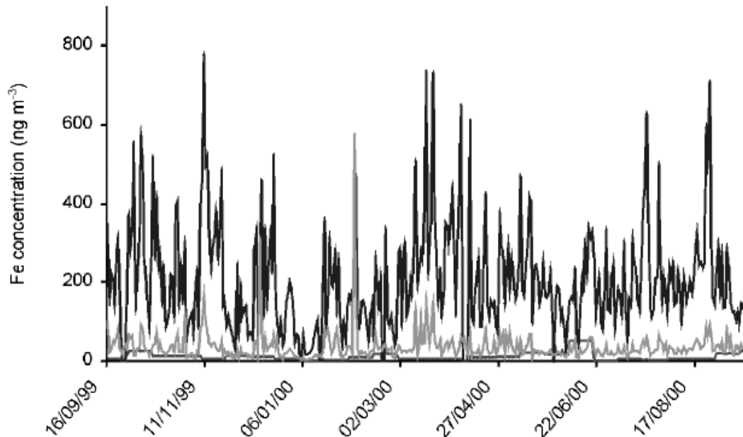
Fig. 2. Example time series of metal concentration. Three hundred and sixty-five daily measurements are illustrated for PM 10 (upper time series), PM 2.5 (middle time series) and limit of detection for analysis (lower time series).
