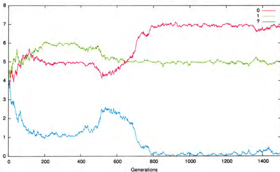
Figure 9.5: Replication of Kirby & Hurford -1500 Generations
