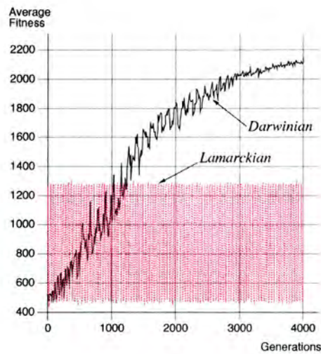
Figure 2.6: Experiment 1 –The average fitness of 0–4000 Generations
