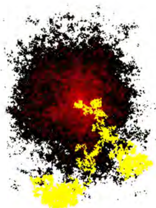
Figure A.2: 2D-Random Walk
