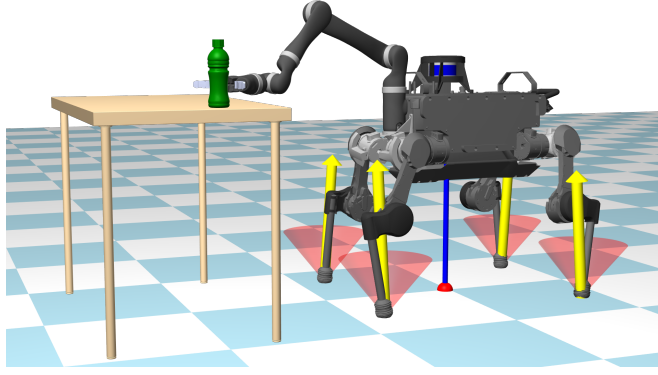
Figure 17: The figure shows the robot at the beginning of a pick-and-place task. The ground-foot contact forces are shown in yellow and the friction cones are shown in red. The blue line represents the CoM projection.
