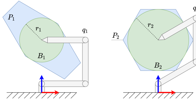
Figure 6: Two valid configurations for reaching the same end-effector target. The blue polygons P_1 and P_2 are the force polytopes of configurations q_1 and q_2 , respectively. The green circles B_1 and B_2 are the largest balls centred at the end-effector that can be inscribed inside those polytopes. The radius of B_1 and B_2 are denoted by r_1 and r_2 , and here r_2 > r_1 .
