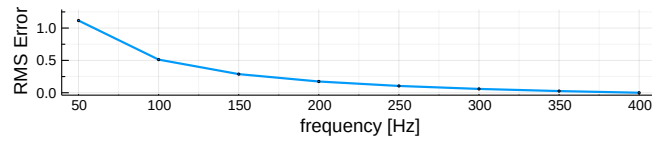
Figure 22: Root-mean-square error (RMSE) in newtons of the SUF given different discretisations, for a 400 Hz baseline.
