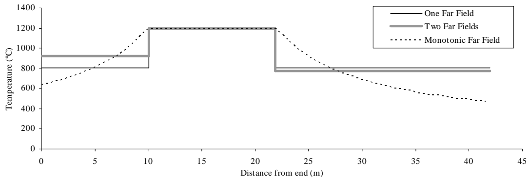
Figure 10. Example range of far field temperature definitions.
