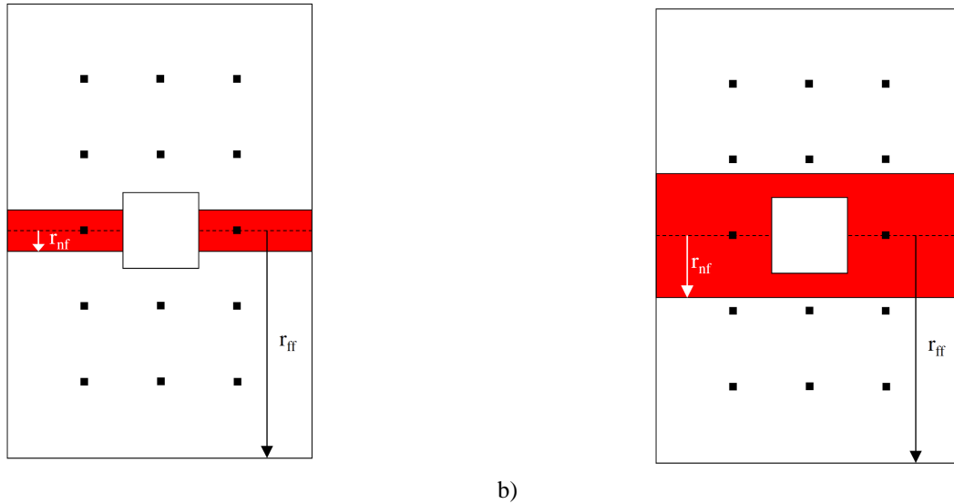
Figure 5. The measurement of r_{ff} and r_{nf} for two different indicative fire sizes (a) small; and (b) large.
