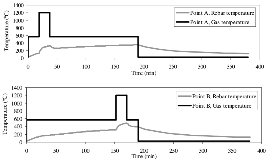
Figure 6. (a) Gas temperature and corresponding rebar temperature at point A; (b) gas temperature and corresponding rebar temperature at point B for a 10% linearly traveling fire.
