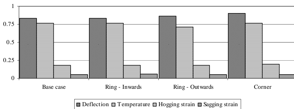
Fig. 13. Influence of path on failure metrics.
