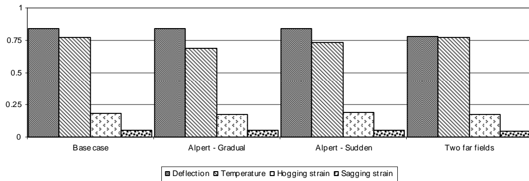
Figure 11. Effect of far field definition on each metric.
