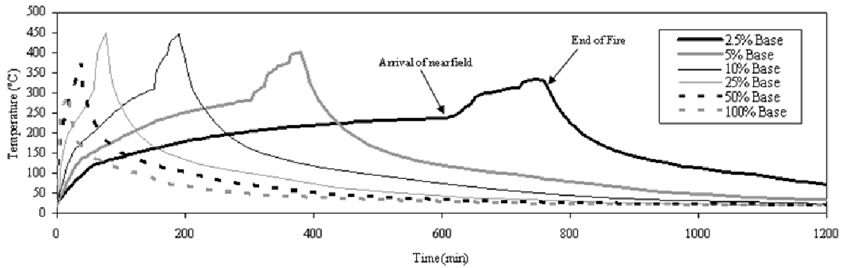
Figure 8. Temperature profiles for the average rebar in the final bay to be heated during the base case fires.
