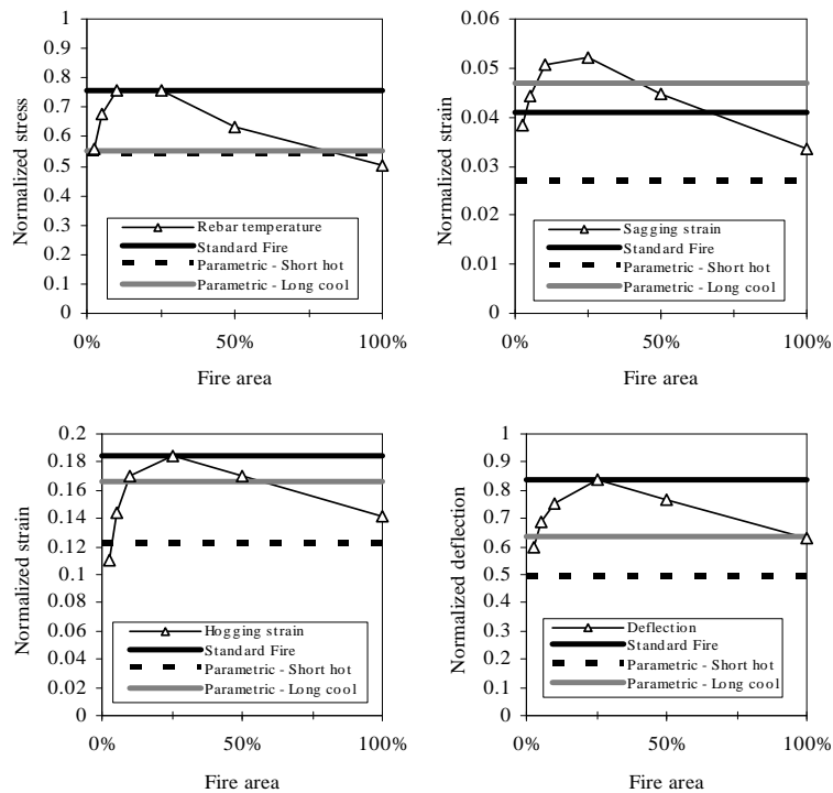
Figure 9. Change in structural distress with near field area: (top left) rebar temperature, Standard Fire equivalent is 1 h 37 min; (top right) sagging tensile strain, value for Standard Fire given after 3 h; (bottom left) hogging tensile strain, Standard Fire equivalent is 1 h 18 min; and (bottom right) deflection, Standard Fire equivalent is 1 h 54 min.
