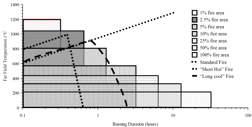
Figure 3. Far field temperatures vs. total burning durations for different fire sizes. Standard and two (“short hot” and “long cool”) parametric Eurocode fire curves are also shown for reference.
