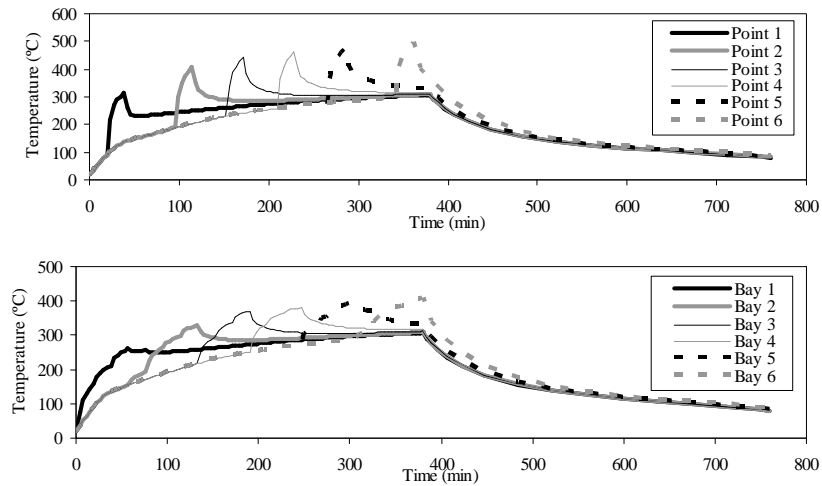
Figure 7. (a) Single point rebar temperature at the centre of bays 1–6 during the 5% base case fire; (b) average rebar temperatures for the whole of bays 1–6 for the 5% base case fire.
