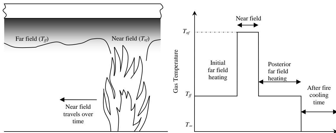
Figure 1. (a) Near field and far field temperatures induced by localized travelling fire; (b) far field and near field exposure durations at an arbitrary point within the fire compartment.
