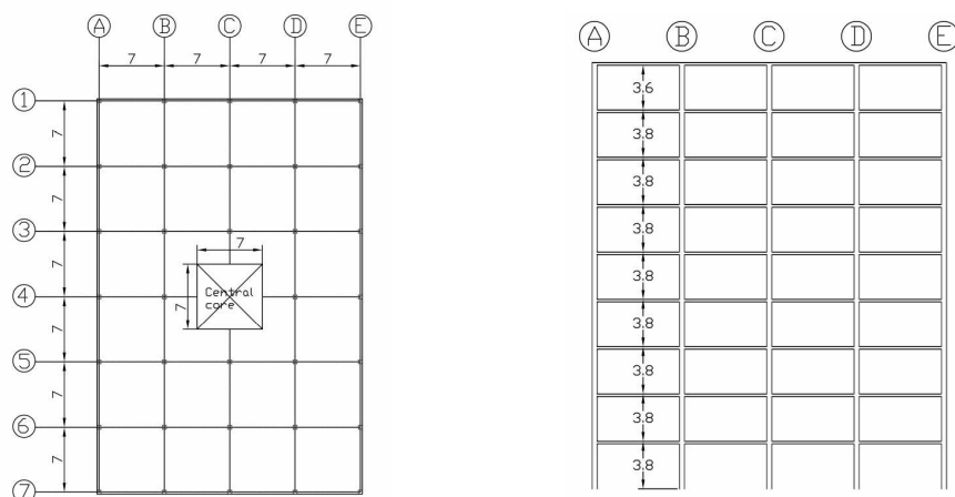
Figure 2. Plan and elevation of concrete structure, dimensions in metres.
