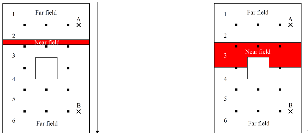
Figure 4. (a) Progression of the 2.5% fire across the floor plate; (b) Progression of the 25% fire across the floor plate. Bay numbers are indicated in both figures.
