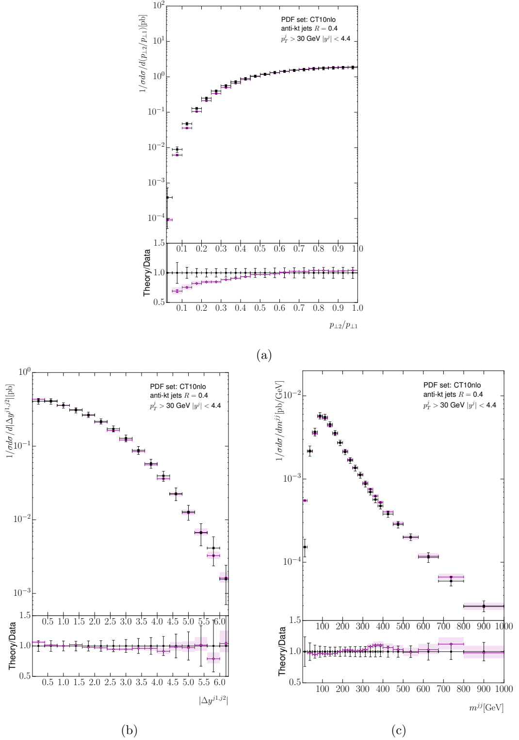
Figure 4.14: The predictions of figs. (4.13a), (4.12a) and (4.11a) normalised to the total cross-section, with scale variation consistently applied to numerator and denominator.
