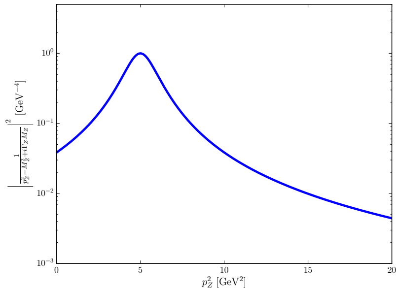
Figure 2.7: The absolute value squared of the Z^0 propagator for a range of values of the invariant mass squared of the Z^0 , p_Z^2 . We see that, as expected, it is strongly peaked at the Z^0 mass and, as such, is an ideal candidate for using importance sampling.
