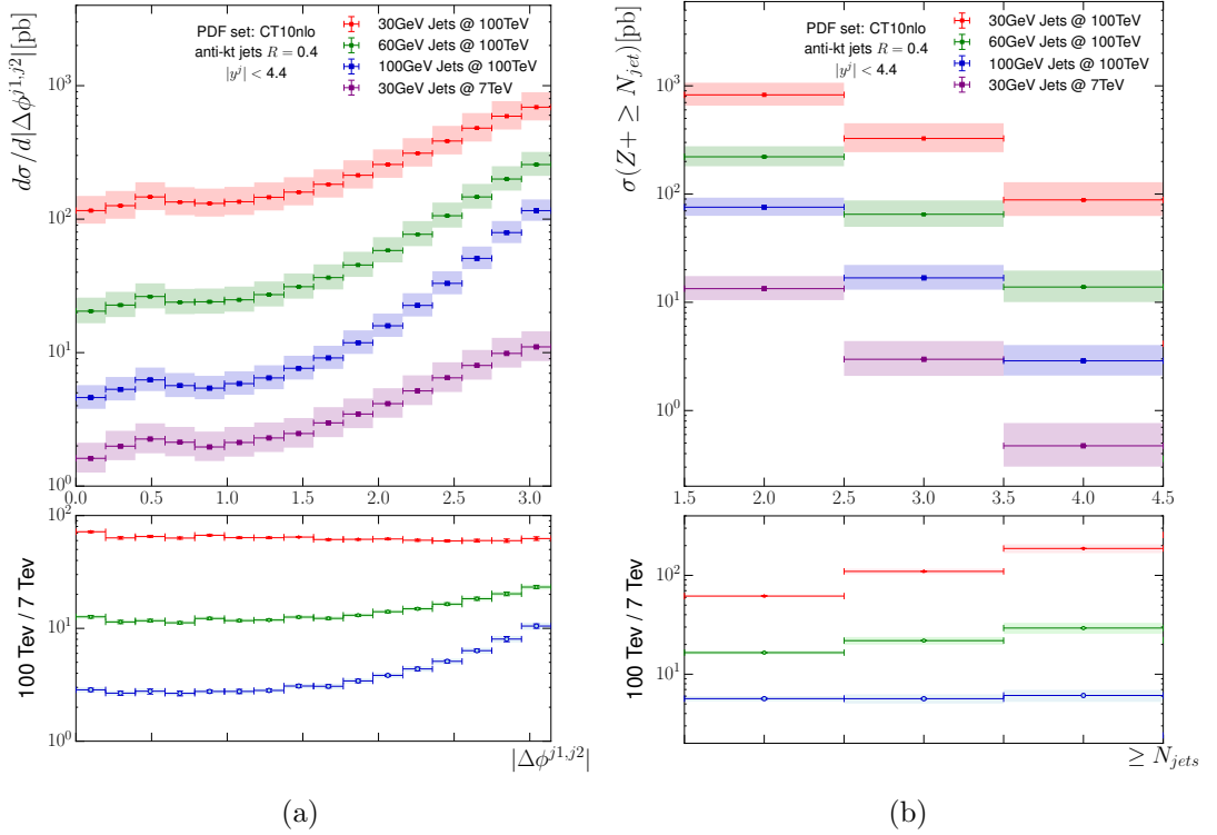
Figure 6.1: Fig. (6.1a) - The differential cross-section for Z/\gamma^* plus inclusive dijets as a function of the azimuthal separation of the dijet system. Fig. (6.1b) - The cross-section for Z/\gamma^* plus inclusive dijets as a function of the number of jets, N_{jets} .
