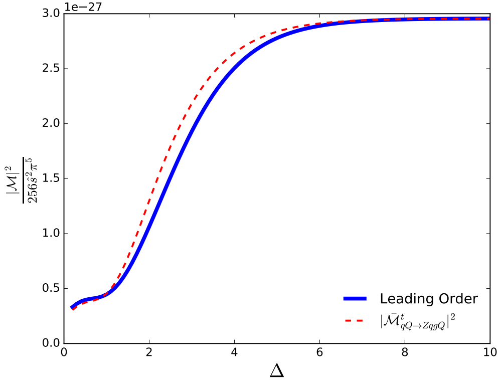
Figure 4.5: A slice through phase space for the Z/\gamma^* + 3 jet final state. The slice defined is akin to that described for the 2 jet case in fig. (4.2) where as \Delta increases we pull apart all three jets and the leptonic decay products are emitted increasingly far into the forward direction.
