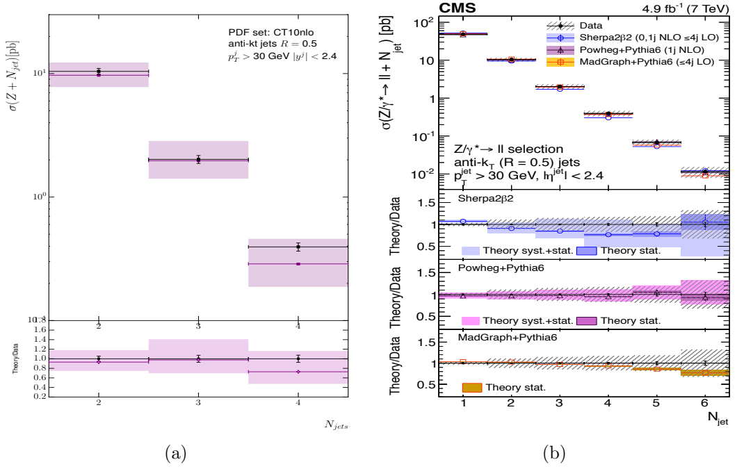
Figure 4.15: The inclusive jet rates as given by (a) the HEJ description and (b) by other theoretical descriptions, both plots compared to the CMS data in [59].
