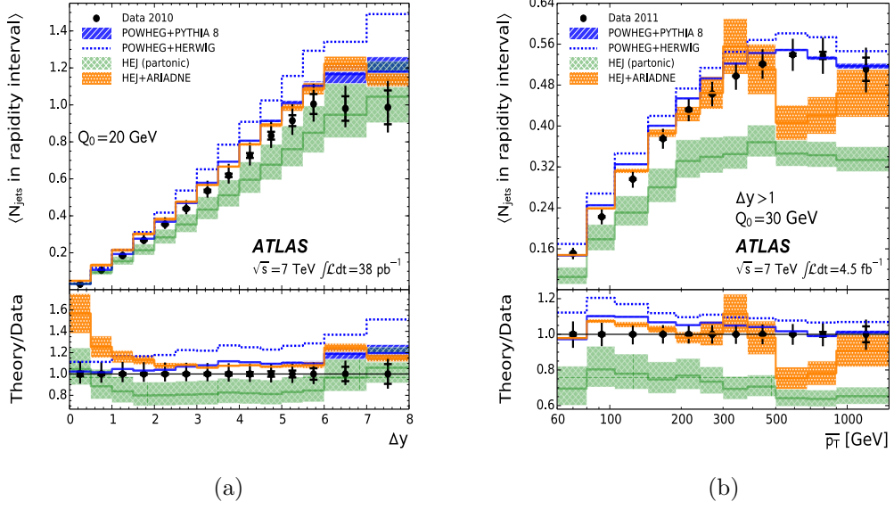
Figure 5.2: The average number of jets, \langle N_{\text{jets}} \text{ in the rapidity interval} \rangle , in the rapidity gap bounded by the dijet system, as a function of (a) the rapidity gap, \Delta y , and (b) the average p_T , \overline{p_T} , of the dijet system.
