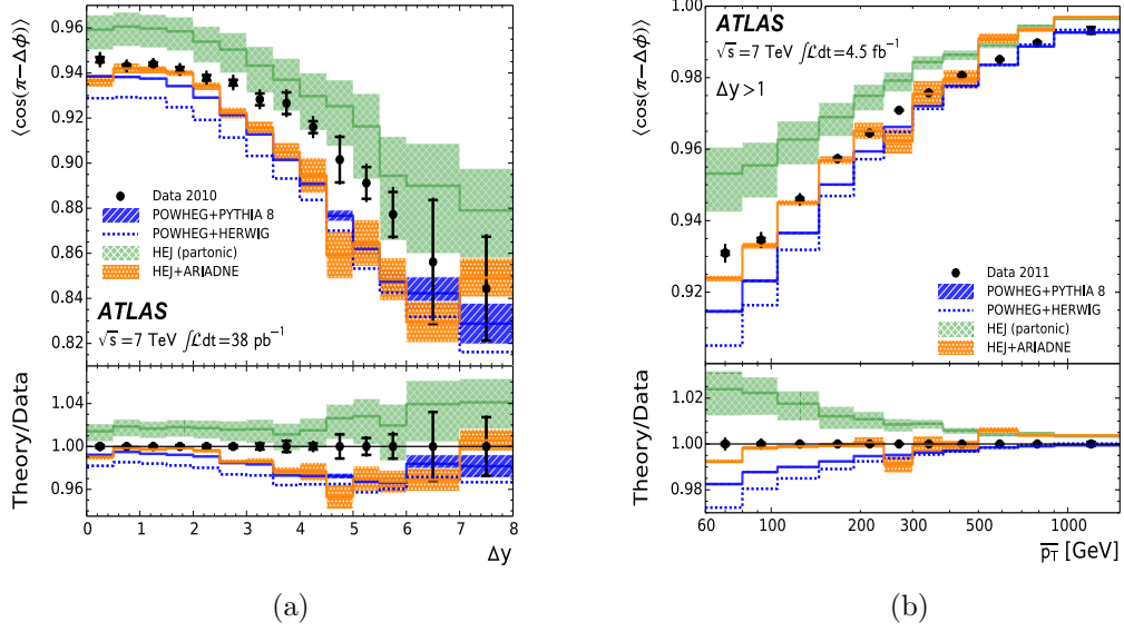
Figure 5.3: The first azimuthal angular moment, \langle \cos(\pi - \Delta\phi) \rangle , as a function of (a) the rapidity gap, \Delta y and (b) the average p_T , \bar{p}_T , of the dijet system.
