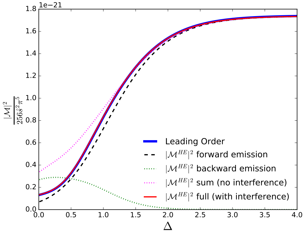
Figure 4.3: The matrix-element squared divided by the square of the partonic centre-of-mass energy for qQ \rightarrow ZqQ with the Z^0 decaying to an electron-positron pair for the phase space slice described in eqn. (4.5). Increasing values of \Delta represent increasing rapidity separation between the jets. The different lines show the contributions from different terms in the calculation: only emission from the forward or the backward quark line (black, dashed and green, dotted), their sum without the interference term (magenta, dotted) and their sum including interference (red, solid) which is seen to agree exactly with the LO result (blue, thick solid).
