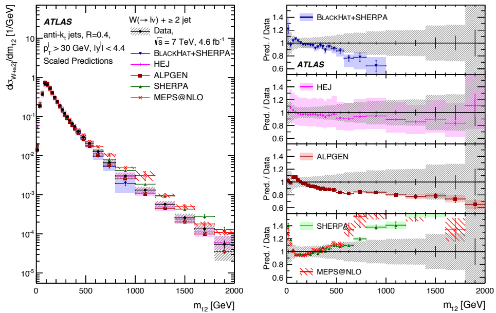
Figure 3.8: The distribution of W^\pm plus inclusive dijets with at least 2 jets differential in the invariant mass of the leading dijets in p_\perp , m_{12} . Fig. from [5].
