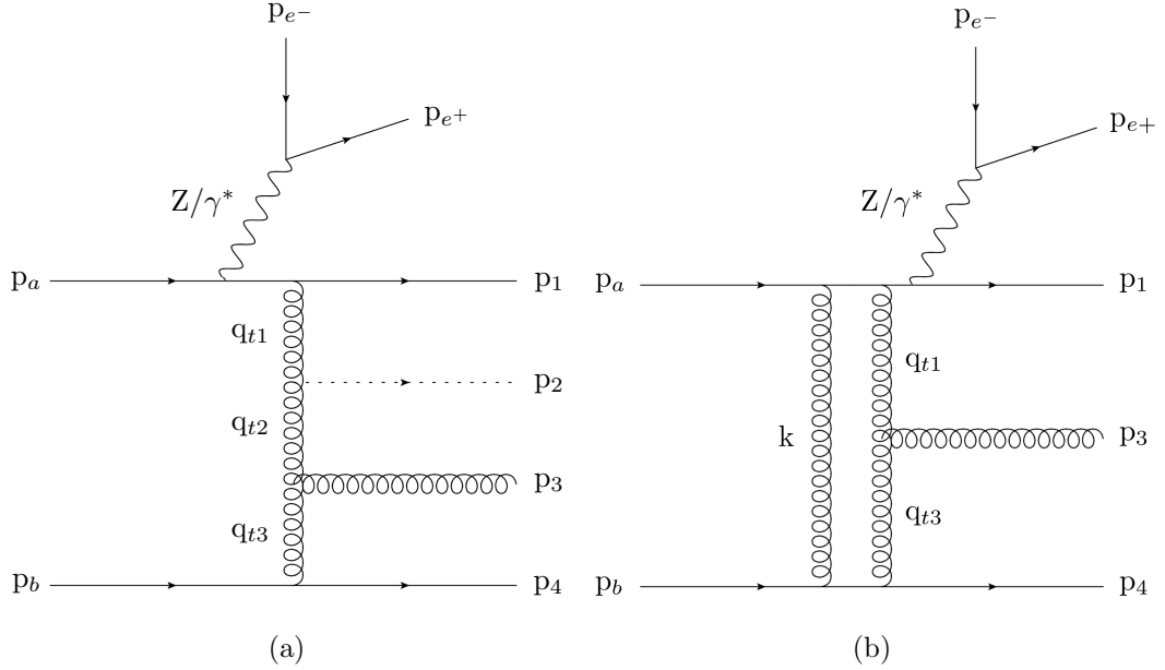
Figure 4.7: Examples of both real and virtual diagrams contributing to 2 \rightarrow 3 scattering. In fig. (4.7a) the p_2 has been drawn with a dashed line to denote it is not resolvable. In fig. (4.7b) the final state momenta have been labelled in a seemingly strange way - this was done to make clear the cancellation when working through the algebra.
