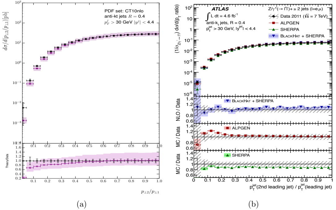
Figure 4.13: These plots show the differential cross section in the ratio of the leading and second leading jet in p_T from (a) HEJ and (b) other theory descriptions and data [2].
