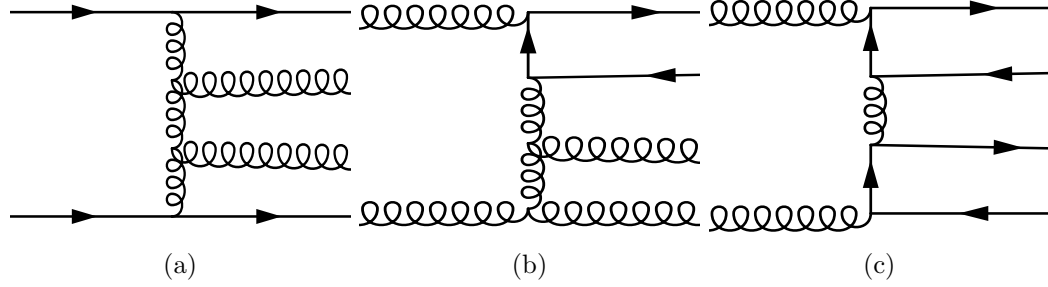
Figure 3.4: Three processes contributing to exclusive four jet production. (a) has the maximum number of gluons exchanged in the t -channels (three) and will dominate in the High Energy limit, (b) and (c) only have two and one gluon which can reggeise. As such as we move from (a) to (c) we will lose powers of large logarithms but maintain the same power of \alpha_s and therefore we can reasonably approximate quad-jet production by neglecting (b) and (c) in the High Energy limit.
