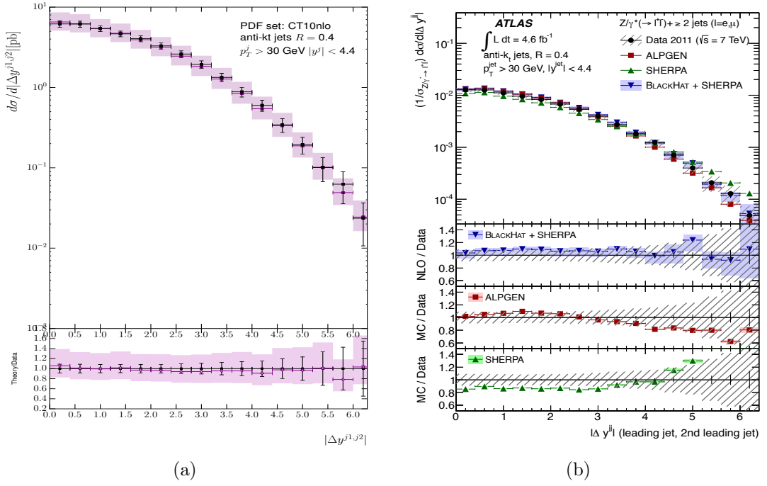
Figure 4.12: The comparison of (a) HEJ and (b) other theoretical descriptions and data [2] to the distribution of the absolute rapidity different between the two leading jets. HEJ and Blackhat+Sherpa give the best description.
