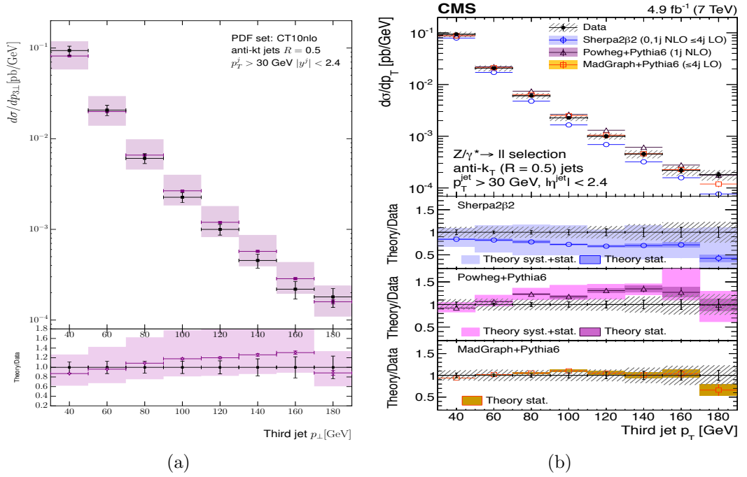
Figure 4.17: The transverse momentum distribution of the third hardest jet in inclusive dijet events in [59], compared to (a) the predictions from HEJ and (b) the predictions from other theory descriptions.
