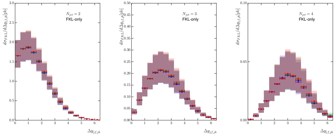
Figure 4.9: The effect of varying \lambda_{cut} on the differential distribution in the rapidity gap between the two extremal jets in rapidity, \Delta y_{jf,jb} , with the N_{jet} = 2, 3, 4 exclusive selections shown from left to right. \lambda_{cut} = 0.2 (red), 0.5 (blue), 1.0 (green), 2.0 (purple). The bands represent the scale variation described in the text.
