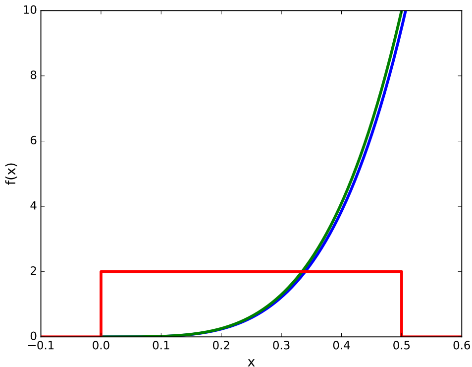
Figure 2.6: A simple importance sampling example (see eqn. (2.90)). The integrand, f(x) , is shown in blue, the importance sampling distribution is shown in green and, for comparison, the uniform probability density function used in the naïve case of no importance sampling is also shown (in red).
