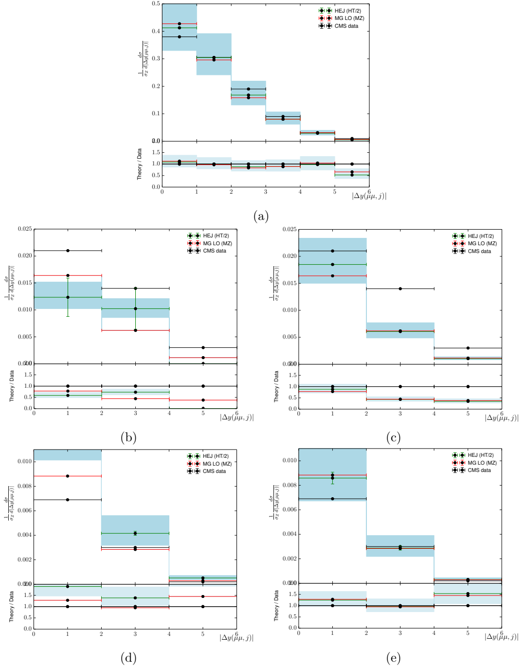
Figure 4.18: Comparisons of HEJ and MadGraph_aMC@NLO to data from a CMS study of double-differential Drell-Yan production. Fig. (4.18a) shows the mass range focussed on the Z^0 peak (60-120 GeV), figs. (4.18b) and (4.18c) show the di-lepton invariant mass range from 30-60 GeV and lastly figs. (4.18d) and (4.18e) show the mass range from 120-1500 GeV. For figs. (2.9b-e) which probe regions away from the Breit-Wigner peak two HEJ lines are shown - figs. (4.18b) and (4.18d) use the naïve Breit-Wigner sampling while figs. (4.18c) and (4.18e) use a modified importance sampling scheme.
