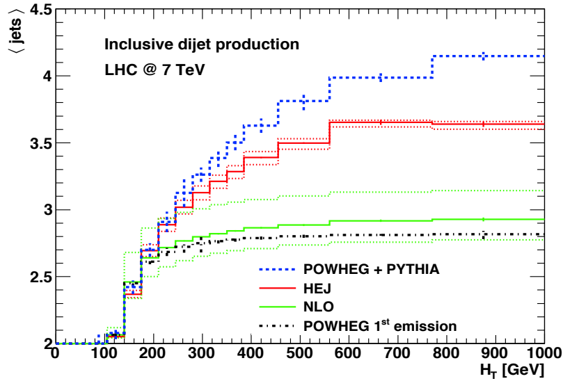
Figure 2.2: Predictions for the average number of jets as a function of the sum of the transverse momenta in the event, H_T , for inclusive dijets at a 7 TeV LHC. Figure from [9].
