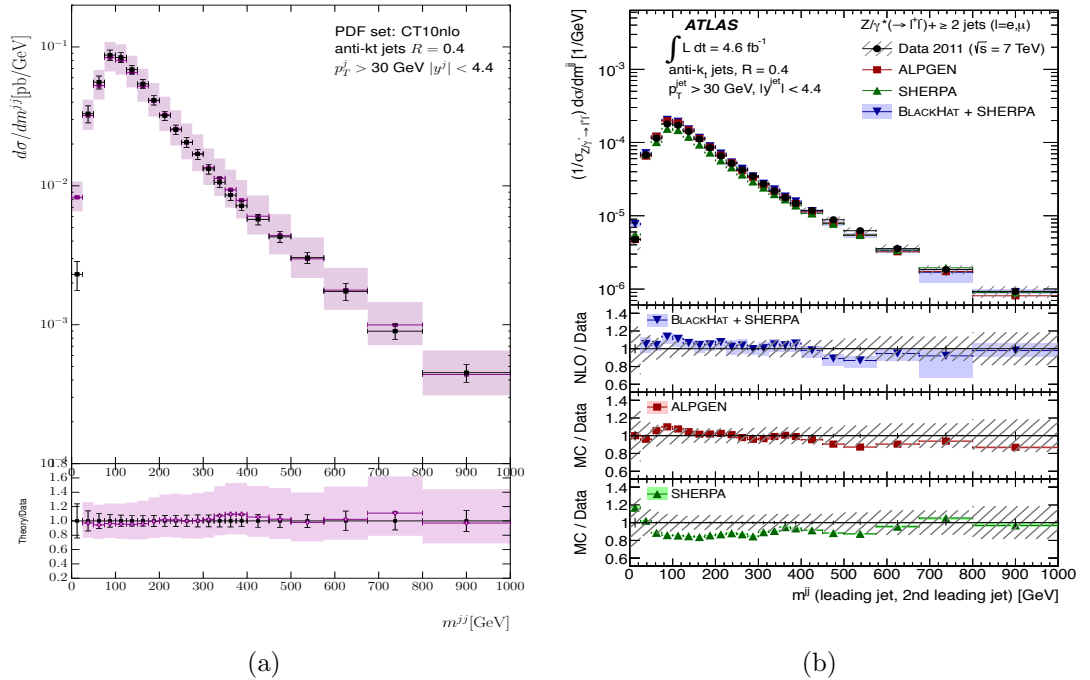
Figure 4.11: These plots show the invariant mass between the leading and second-leading jet in p_T . As in Fig. (4.10), predictions are shown from (a) HEJ and (b) other theory descriptions and data [2]. These studies will inform Higgs plus dijets analyses, where cuts are usually applied to select events with large m_{12} .
