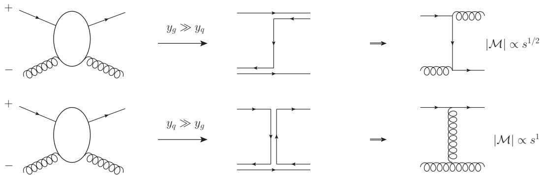
Figure 3.5: The limiting behaviour of gg \rightarrow qq in the regions of phase space where either y_g \gg y_q or y_q \gg y_g . The intermediate diagrams indicate the flow of colour through the process.
