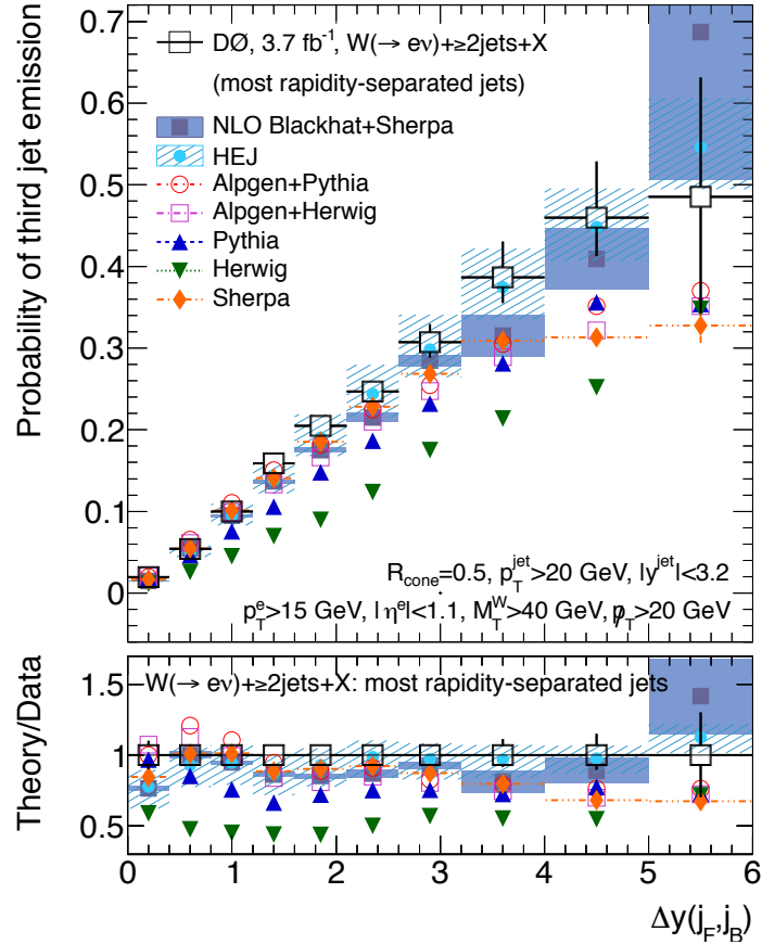
Figure 2.5: The probability of a third jet emission in W^\pm plus inclusive dijets as a function of the rapidity gap between the two leading jets in rapidity at the D0 experiment at the Tevatron experiment. The data are compared to a number of fixed-order generators plus the leading logarithmic accurate HEJ and the NLO accurate Blackhat+Sherpa.
