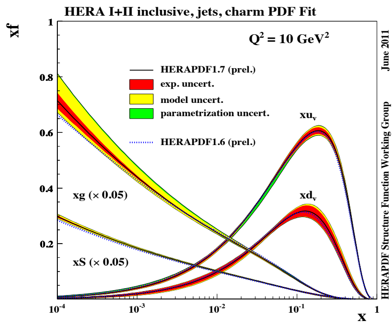
Figure 2.8: Recent parton distribution function fits from the HERA experiment. The observed variation in f(x_{a/b}, Q^2) , especially at high x_{a/b} , can be used to reduce the variance of a Monte Carlo approach to computing eqn (2.41) by using an importance sampling approach
