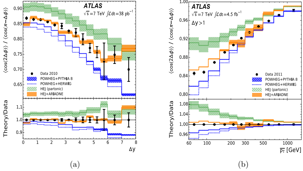
Figure 5.4: The ratio of the second azimuthal angular moment, \langle \cos(2\Delta\phi) \rangle , to the first azimuthal angular moment, \langle \cos(\pi - \Delta\phi) \rangle , as a function of (a) the rapidity gap, \Delta y , and (b) the average p_T , \overline{p_T} , of the dijet system.
