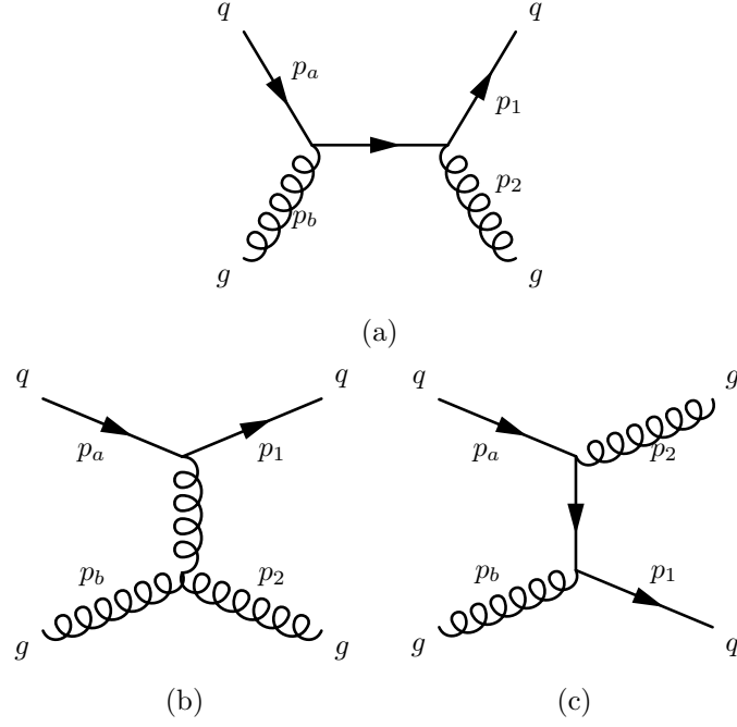
Figure 3.2: The s , t and u channel diagrams contributing to q^-g^+ \rightarrow q^-g^+ at leading order in \alpha_s in figs. (3.2a), (3.2b) and (3.2c) respectively.
