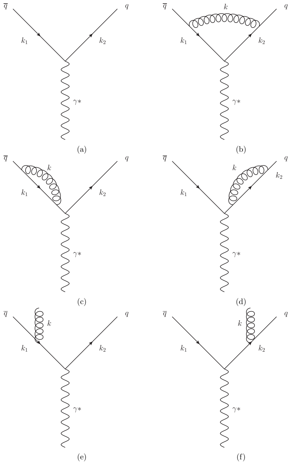
Figure 2.3: Feynman diagrams for calculating the O(\alpha_s) correction to \gamma^* \rightarrow q\bar{q} . Fig. (2.3a) is the leading order contribution, \mathcal{A}_0 . Figs. (2.3b)–(2.3d) are the virtual corrections \mathcal{A}_v , \mathcal{A}_{se1} and \mathcal{A}_{se2} respectively and figs. (2.3e)–(2.3f) are the real emission contributions \mathcal{A}_{r1} and \mathcal{A}_{r2} respectively.
