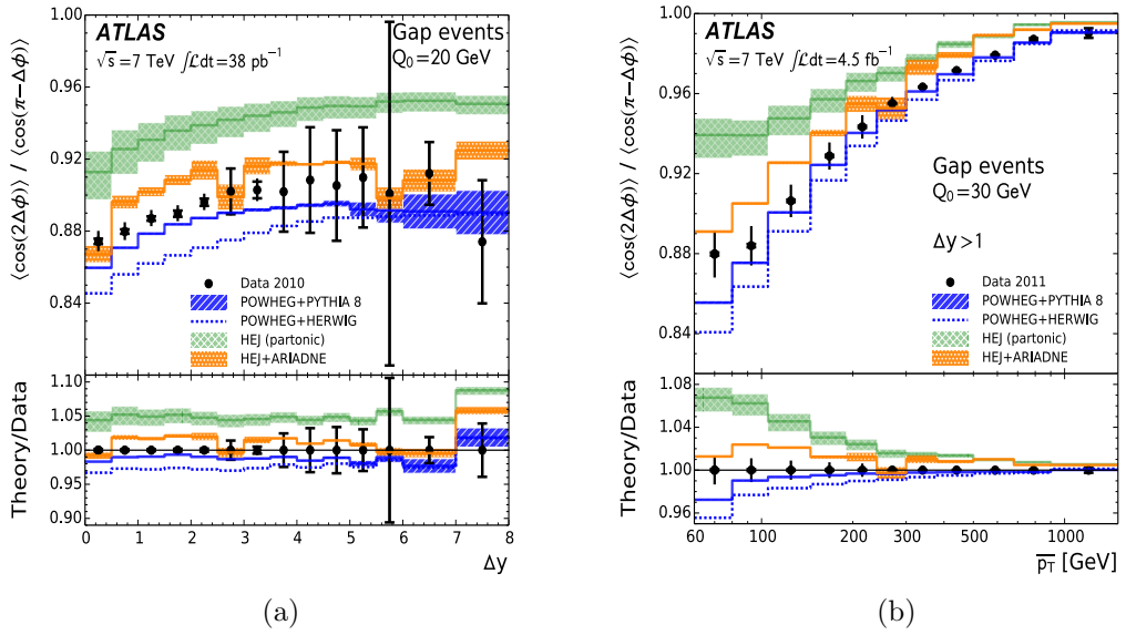
Figure 5.6: The ratio of the second azimuthal angular moment, \langle \cos(2\Delta\phi) \rangle , to the first azimuthal angular moment, \langle \cos(\pi - \Delta\phi) \rangle , as a function of (a) the rapidity gap, \Delta y , and (b) the average p_T , \bar{p}_T , of the dijet system. A veto of Q_0 = 20\text{GeV} , for (a), and Q_0 = 30\text{GeV} , for (b), is applied on activity in the rapidity gap is applied.
