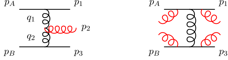
Figure 3.6: The 5 possible emission sites of extra QCD radiation in qQ \rightarrow qQ . Fig. from [19].
