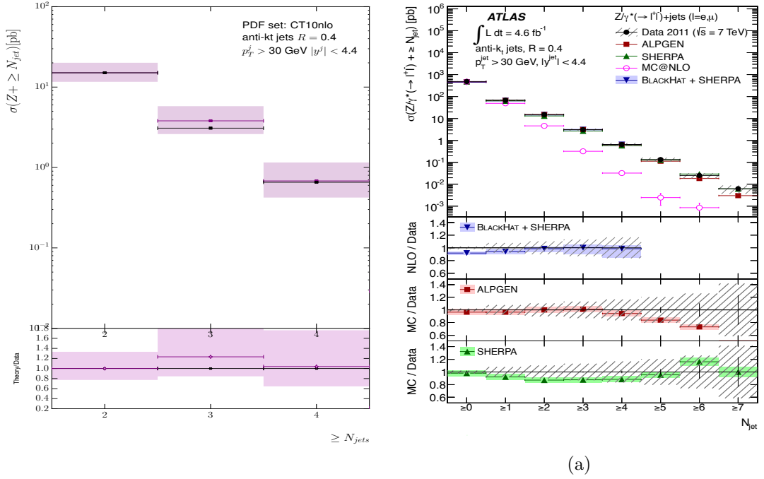
Figure 4.10: These plots show the inclusive jet rates from (a) HEJ and (b) other theory descriptions and data [2]. HEJ events all contain at least two jets and do not contain matching for 5 jets and above, so these bins are not shown.
