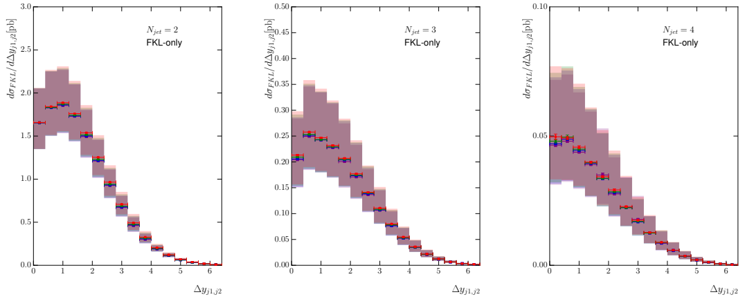
Figure 4.8: The effect of varying \lambda_{cut} on the differential distribution in the rapidity gap between the two leading jets in p_{\perp} , \Delta y_{j1,j2} , with the N_{jet} = 2, 3, 4 exclusive selections shown from left to right. \lambda_{cut} = 0.2 (red), 0.5 (blue), 1.0 (green), 2.0 (purple). The bands represent the scale variation described in the text.
