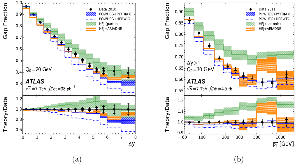
Figure 5.1: The gap fraction, f(Q_0) , as a function of (a) the rapidity gap, \Delta y in the 2010 data, and (b) the average p_T , \overline{p_T} , of the dijet system in the 2011 data.
