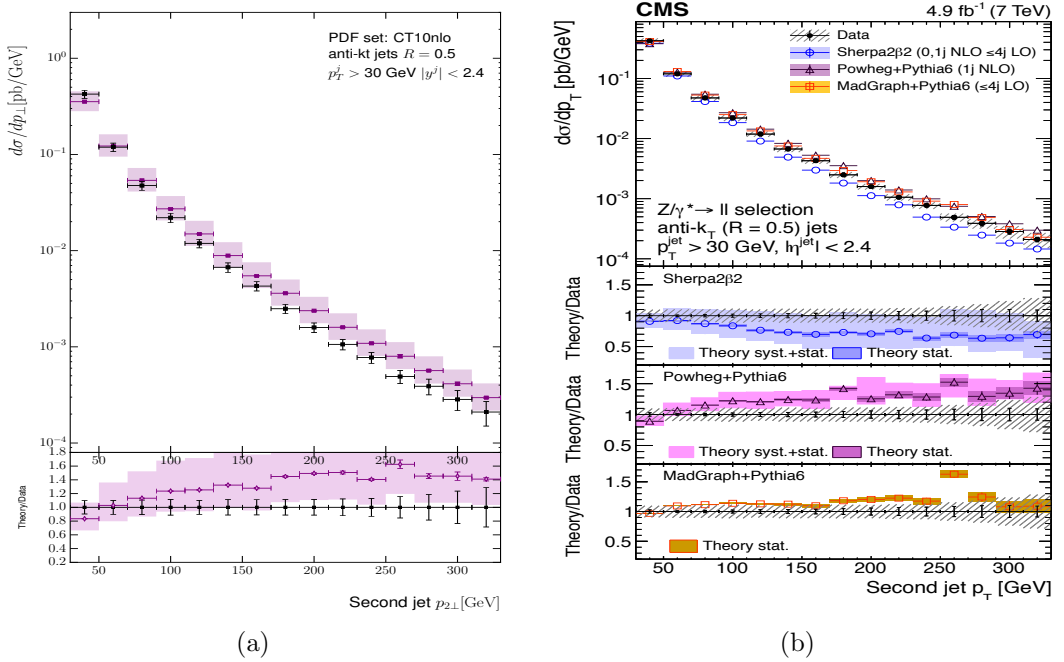
Figure 4.16: The transverse momentum distribution of the second hardest jet in inclusive dijet events in [59], compared to (a) the predictions from HEJ and (b) the predictions from other theory descriptions.
