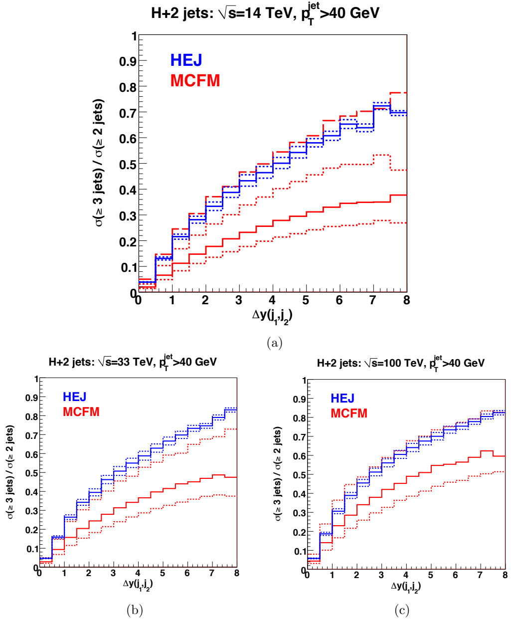
Figure 2.4: The ratio of the inclusive Higgs plus three jet cross-section to inclusive Higgs plus two jet cross-section shown for centre-of-mass energies of 14TeV (similar to the current LHC), 33TeV and 100TeV (possible energy scales for a hadronic future circular collider).
