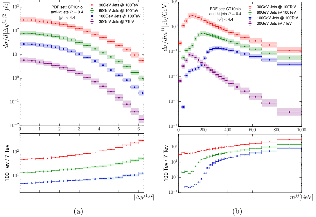
Figure 6.2: Fig. (6.2a) - The differential cross-section for Z/\gamma^* plus inclusive dijets as a function of the absolute value of the rapidity gap between the dijets, |\Delta y^{j1,j2}| . Fig. (6.2b) - The differential cross-section for Z/\gamma^* plus inclusive dijets as a function of the invariant mass of the dijets, m^{jj} .
