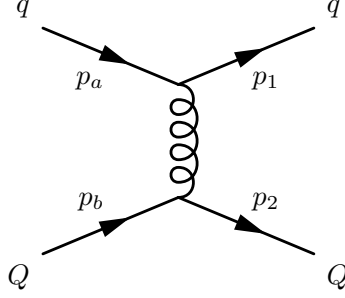
Figure 3.1: The only diagram which contributes to qQ \rightarrow qQ at leading order in \alpha_s .
