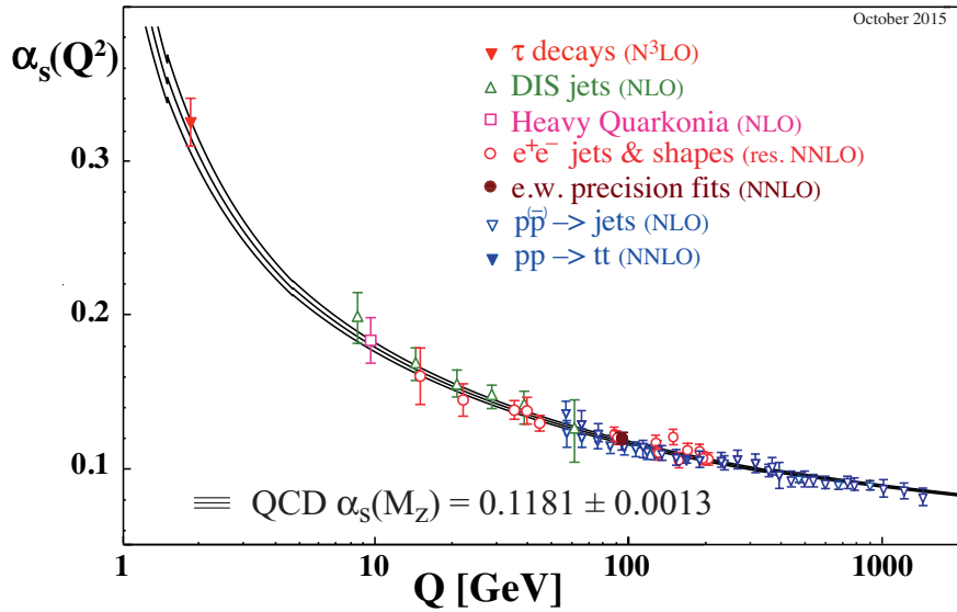
Figure 2.1: The evolution of \alpha_s over several orders of magnitude in the scale of the process Q^2 . The data points fitted are of varying degrees of formal accuracy ranging from next-to-leading order in \alpha_s (NLO) to next-to-next-to-next-to-leading order in \alpha_s ( N^3LO ). Fig. from [27].
