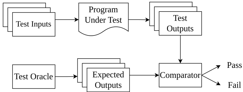
Figure 1.1: Test oracles compute the test inputs’ expected outputs. They identify program correctness by comparing the actual output of a test execution with the expected output.
