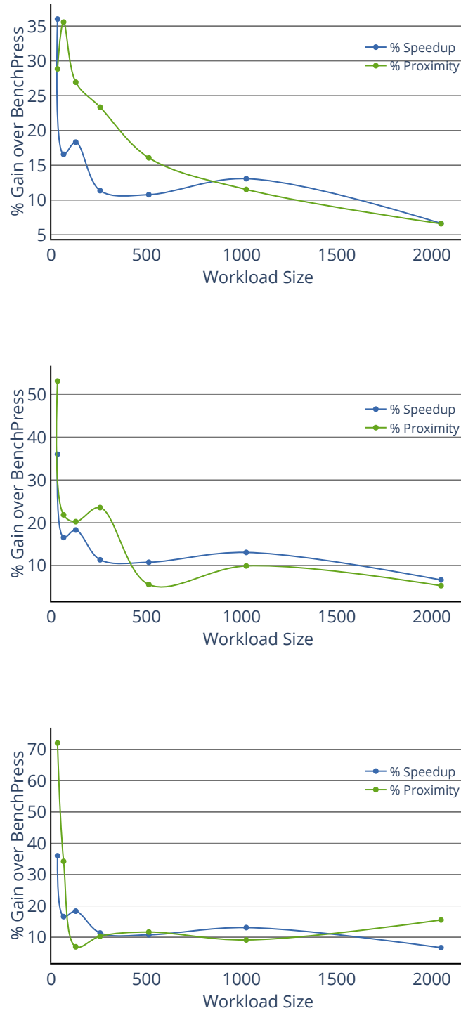
Figure 6.3: BENCHDIRECT's acquired execution time speedup and relative proximity improvement over BENCHPRESS per workload size configuration for (a) Grewe's et al., (b) InstCount and (c) Autophase feature spaces.
