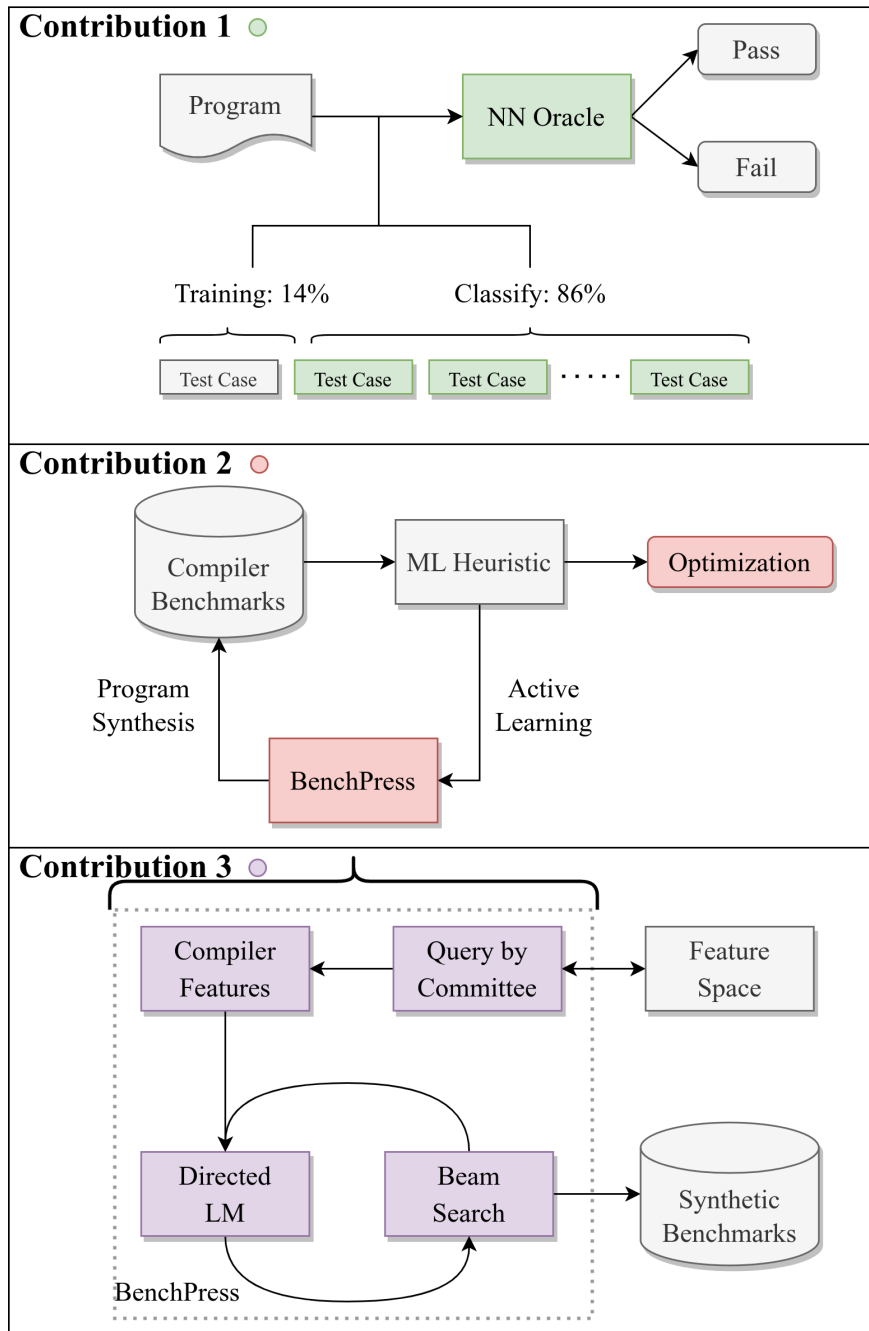
Figure 1.3: Three contributions presented in applying ML to automate software testing and compiler optimisation: (a) We propose an ML oracle, which allows developer to label only 14% of test cases with the remaining being classified automatically. (b) We present BENCHPRESS, a steerable program generator that uses active learning to improve the training data of predictive models for compilers. (c) We develop BENCHDIRECT, the first directed language model for targeted compiler benchmark generation. This contribution targets benchmarks written by compiler experts up to 36% more accurately and up to 72% faster compared to BENCHPRESS.
