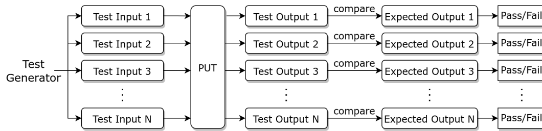
Figure 2.1: An overview of the software testing process.
