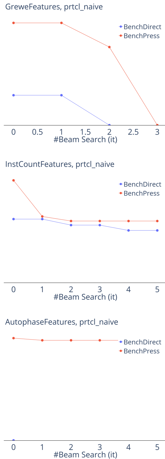
Figure 6.9: A comparative visualization of the minimum distance achieved (y-axis) from particle_naive target benchmark over the course of six beam search iterations (x-axis) for all three feature spaces.
