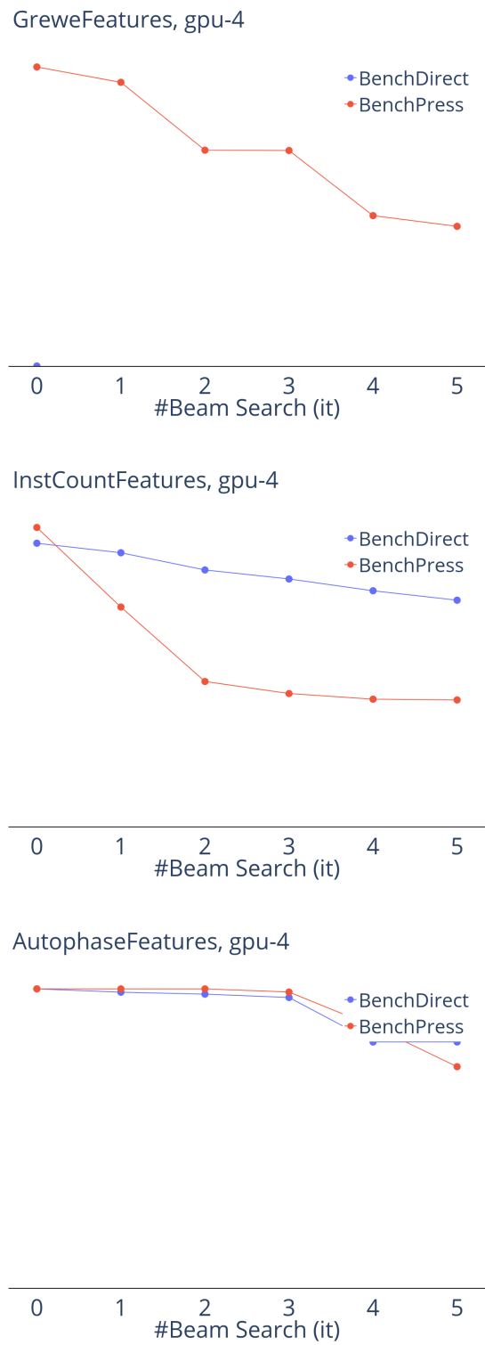
Figure 6.8: A comparative visualization of the minimum distance achieved (y-axis) from gpu-4 target benchmark over the course of six beam search iterations (x-axis) for all three feature spaces.
