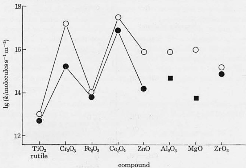
FIGURE 2. Comparison of the activities of the oxides for hydrogen-deuterium equilibration and ethylene-deuterium reactions. The temperatures used to measure either (●) C 2 H 4 -D 2 (addition) or (■) C 2 H 4 -D 2 (exchange) were 298 K for MgO and as given in table 3 for the other oxides. The H 2 -D 2 equilibration rates (O) were determined as follows: Al 2 O 3 at 273 K (Van Cauwelaert & Hall 1970); MgO at 273 K (Eley & Zammitt 1971); ZrO 2 at 298 K (Hughes et al. ); other oxides all at 297 K (Pearce et al. 1969).
