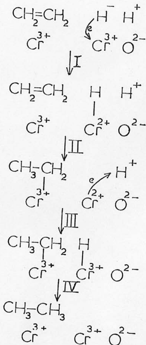
FIGURE 4.5 : Scheme for adsorption and reaction of ethylene and hydrogen on chromia.
