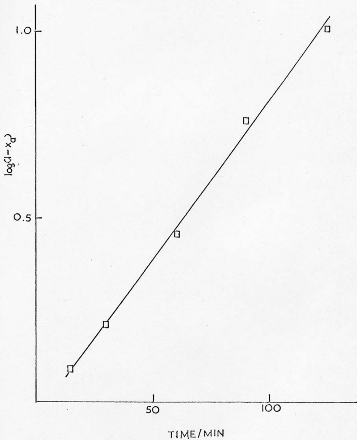
FIGURE 4.3 : Rate Plot for the Addition Reaction of Ethylene and Deuterium on Zinc Oxide at 273K.
