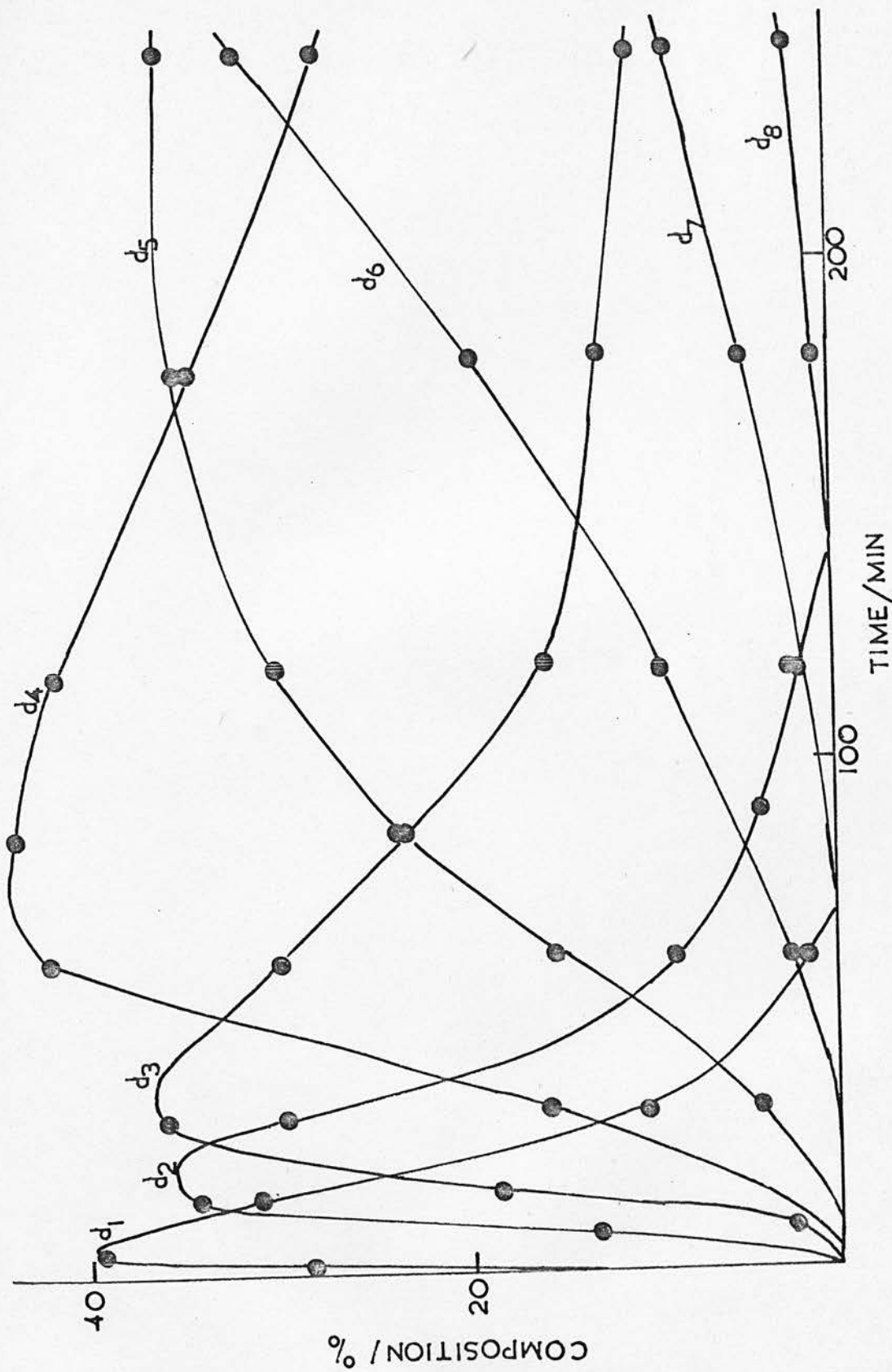
FIGURE 3.1 : Calculated isotopic distributions during reaction with k_B = 0.6 D atoms/ 100 molecules \text{min}^{-1} and k_A/k_B = 20 .
