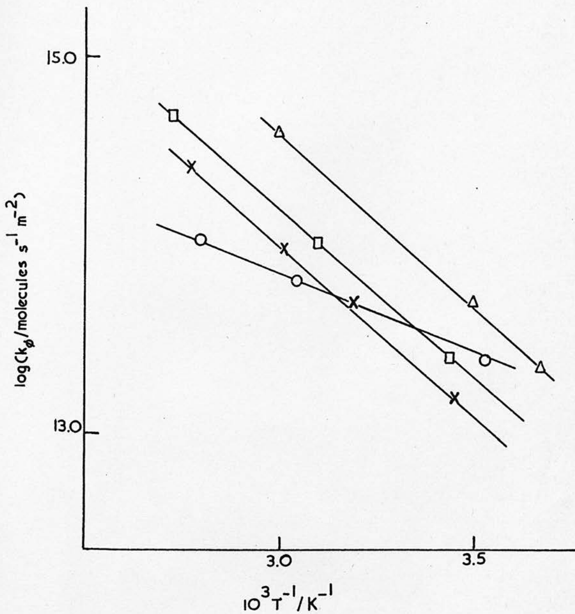
FIGURE 5.2 : Arrhenius plots for the exchange reactions of acyclic alkanes on alumina.
