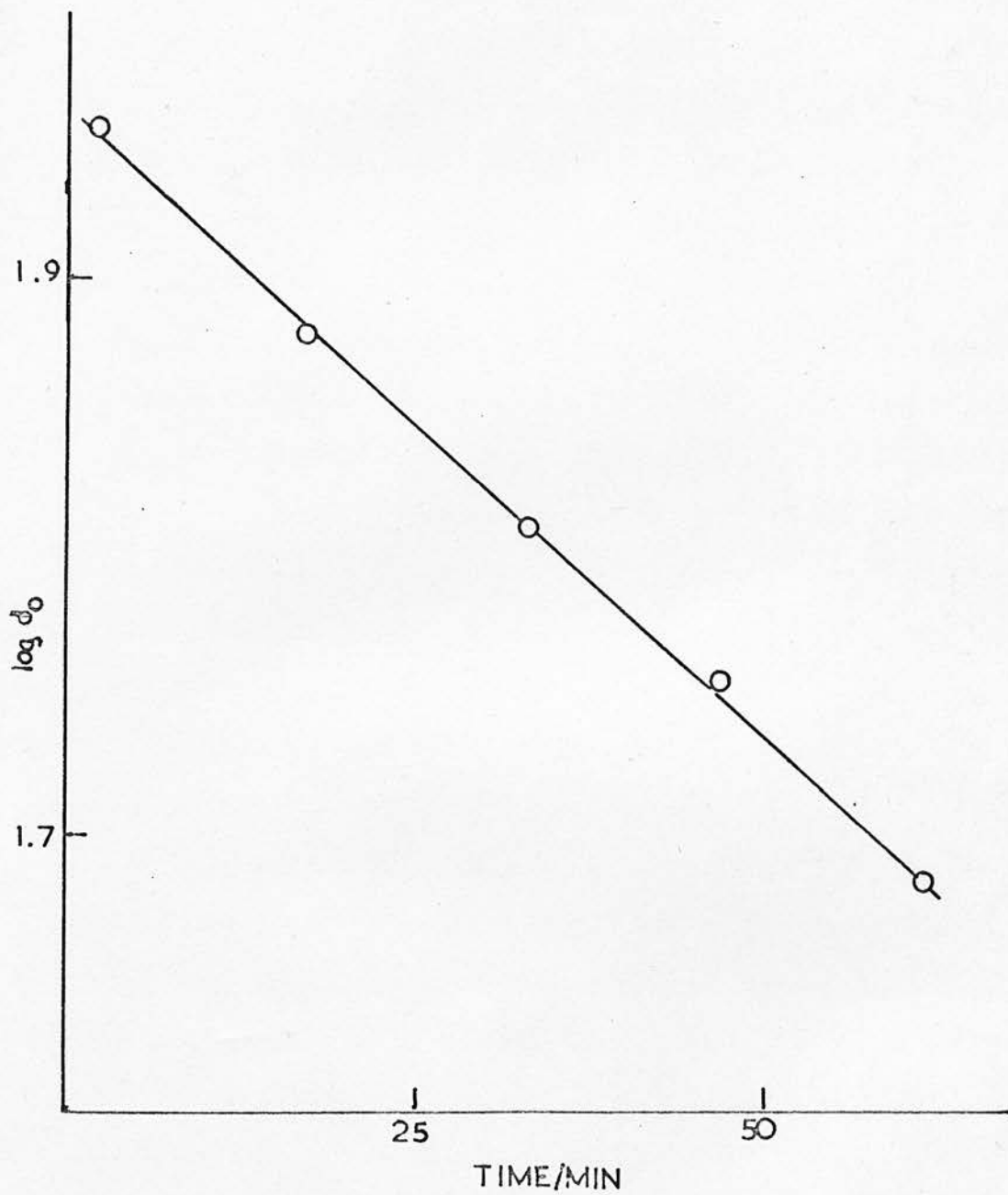
FIGURE 4.2 : Rate Plot for the Exchange of Ethylene with Deuterium on Magnesium Oxide at 298K.
