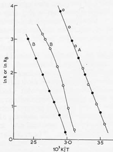
Fig. 5. Arrhenius plots for the estimated rates of exchange from temperature-programmed results with values of \bar{k}/\bar{k}_B of 6 (○) and 21 (●); A represents \bar{k} , the total rate of exchange, and B the rate of the slower group, \bar{k}_B .
