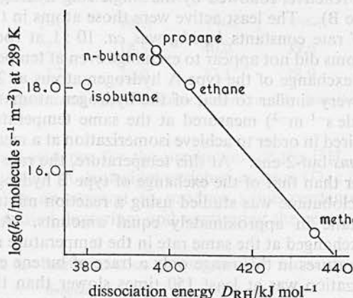
FIG. 1.—Alkane exchange reactions over tungsten; \log k_0 at 289 K as a function of the dissociation energy 15 of the C—H bond for methane, 10 ethane, 10 propane, 10 isobutane 13 and n -butane. 14
