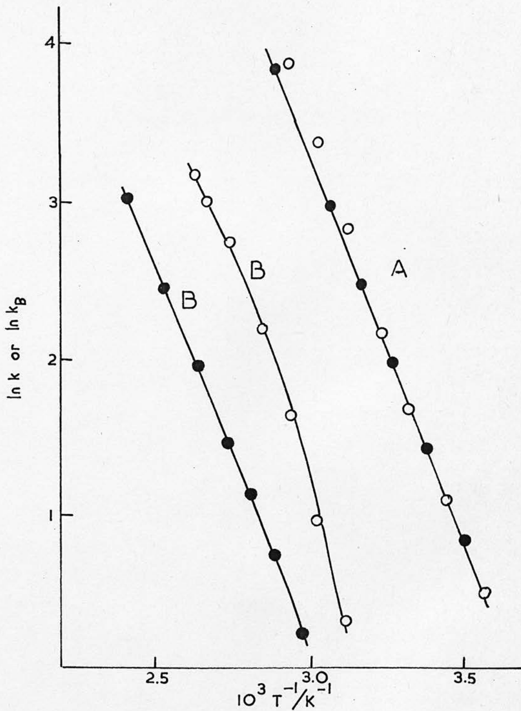
FIGURE 3.5 : Arrhenius plots for the estimated rates of exchange from temperature-programmed results with values of k/k_B of 6 (O) and 21 (●); A represents k , the total rate of exchange and B the rate of the slower group, k_B .
