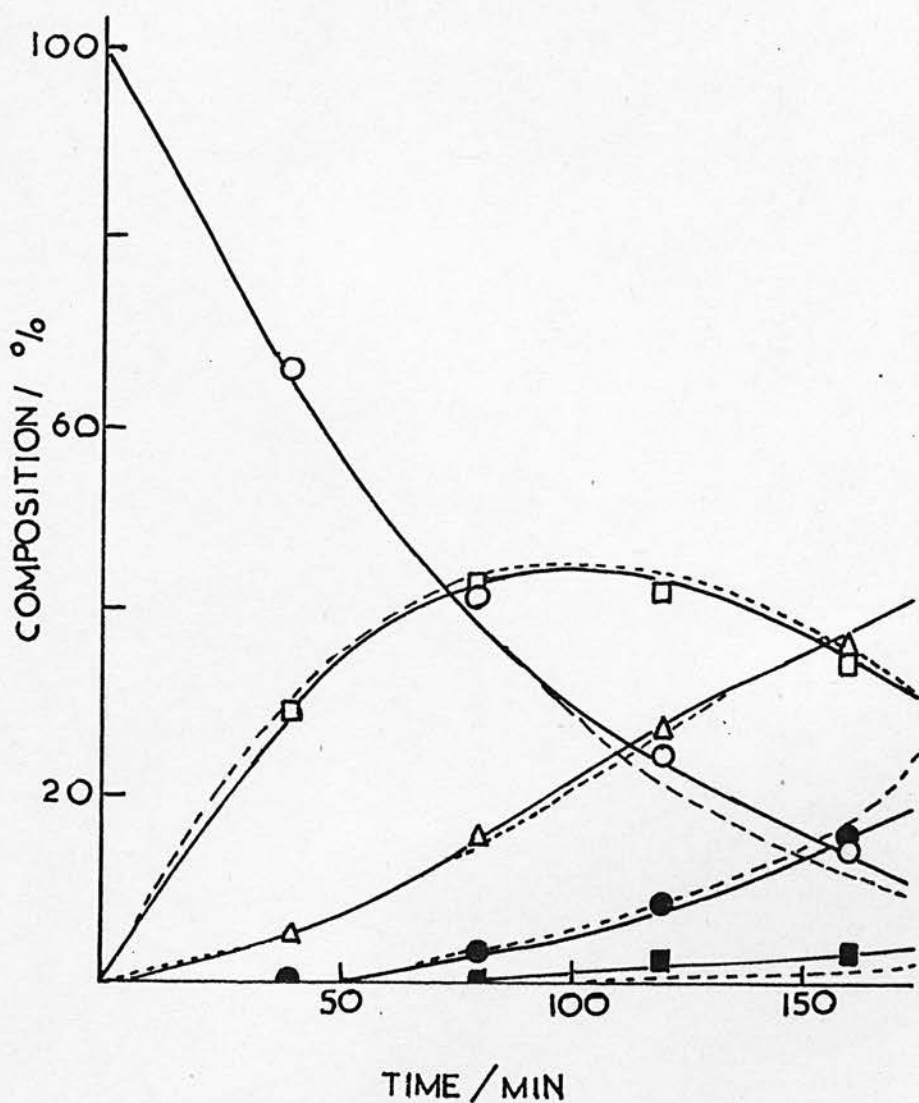
FIGURE 2.3 : Comparison of isotopic distributions obtained for the exchange of ethylene with deuterium on magnesium oxide at 298 and 373K. —, data from PDP11; - - , data from photographic paper; also shown are calculated binomial distributions: ○, ethylene -d_0 ; □, -d_1 ; Δ, -d_2 ; ●, -d_3 ; ■, -d_4 . The parameter \phi represents 100 times the mean number of deuterium atoms present per molecule of hydrocarbon.
