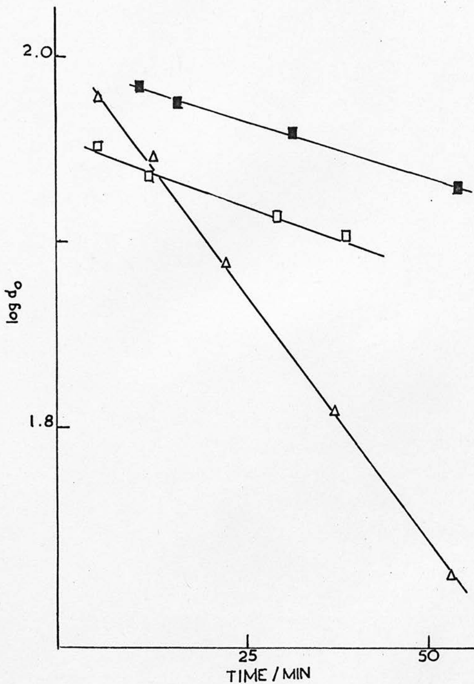
FIGURE 6.3 : Rate plots for the exchange reactions of olefins with deuterium on magnesium oxide.
