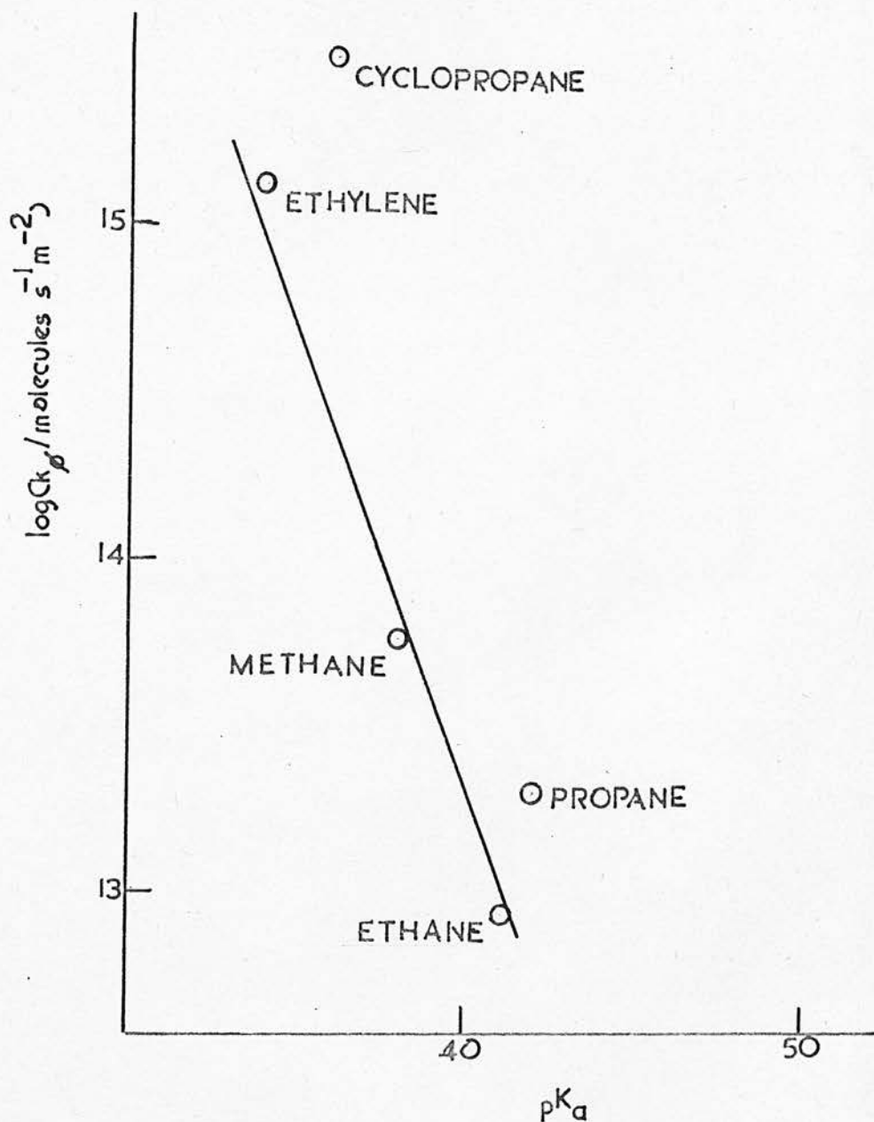
FIGURE 6.5 : Alkane exchange reactions over magnesium oxide; rate of deuterium exchange at 627K as a function of the pK_a of the hydrocarbon. Values of pK_a are from same sources as those in chapter 5.
