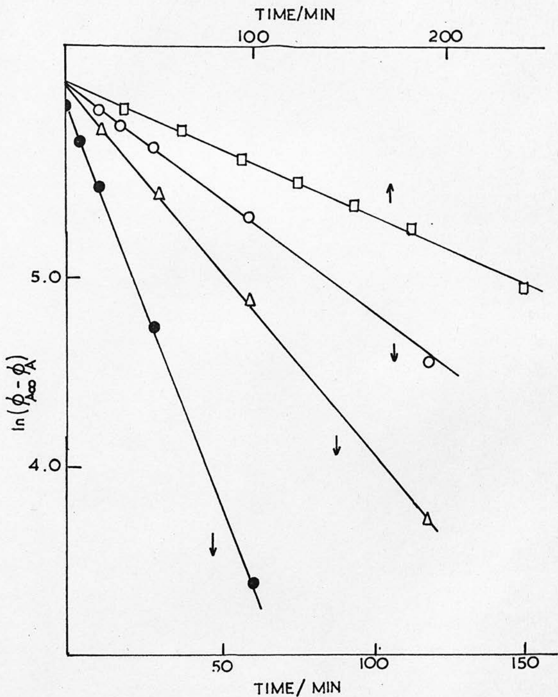
FIGURE 3.3 : Appropriate plots of \phi_A to determine k with values of k_A/k_B of 1 ( \square ), 5 ( \circ ), 10 ( \Delta ) and 20 ( \bullet ).
