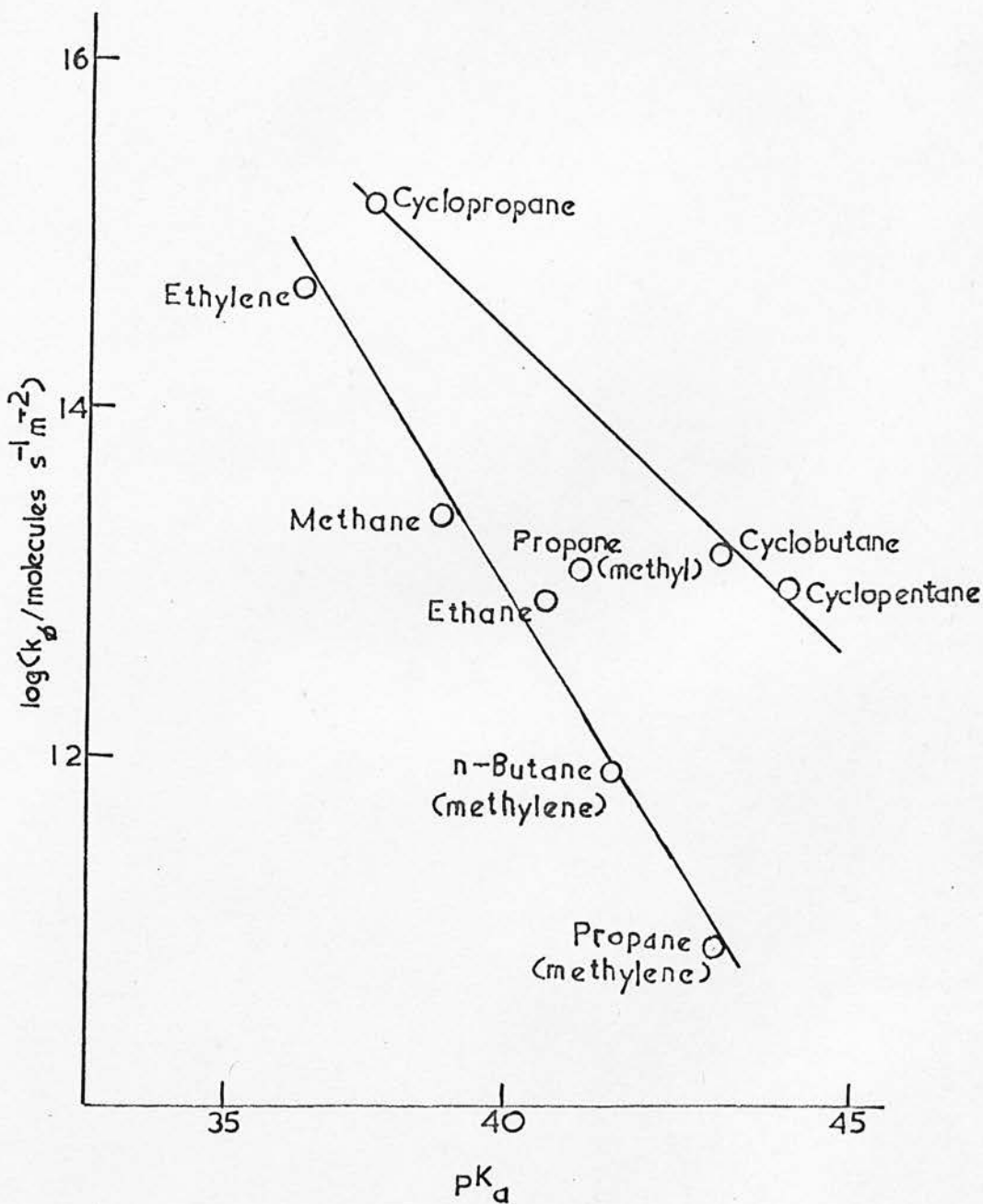
FIGURE 5.5 : Alkane exchange reactions over alumina; \log k_\phi at 289K as a function of the pK_a of the hydrocarbon. The values of pK_a are given to the nearest half-integer for ethane and n-butane and to the nearest integer for the other compounds (15,16) .
