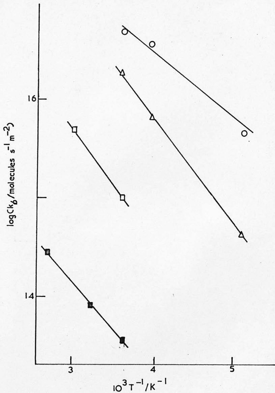
FIGURE 6.4 : Arrhenius plots for the exchange reactions of olefins on magnesium oxide.
