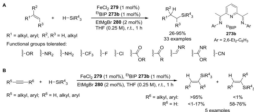
Scheme 2.40. Iron-catalysed hydrosilylation of alkenes and alkynes using in situ reduction of an iron(II) pre-catalyst with ethylmagnesium bromide.
