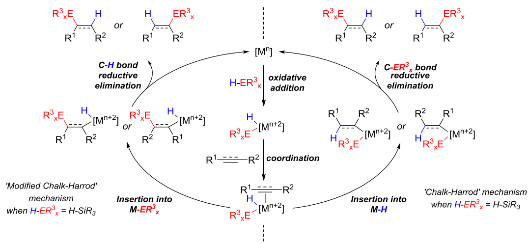
Scheme 1.03. Hydrofunctionalisation of alkenes and alkynes through oxidative addition of a transition-metal catalyst into the hydrogen-heteroatom bond of a hydrofunctionalisation reagent ( H-ER^3_x ).
