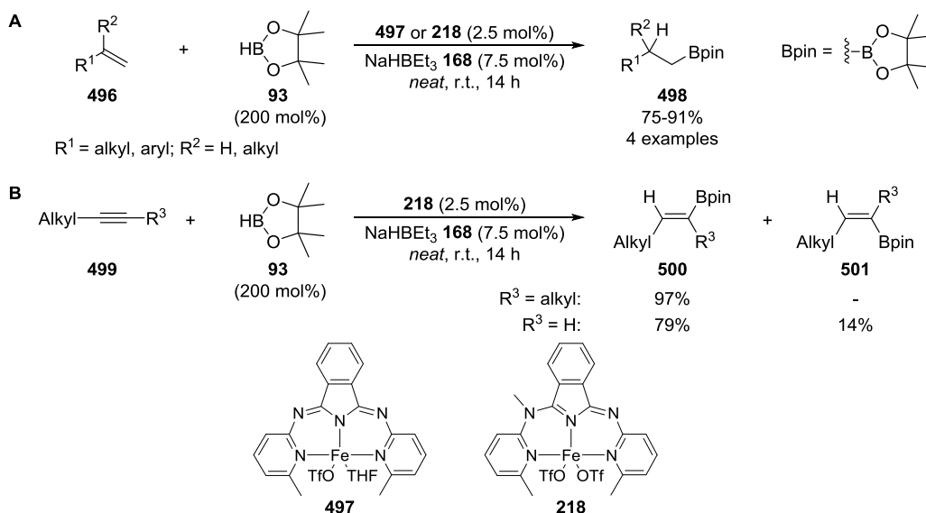
Scheme 3.05. Hydroboration of terminal and 1,2-disubstituted alkenes and alkynes using N,N,N -bMepi iron complexes 497 and 218 , reduced in situ using sodium triethylborohydride.
