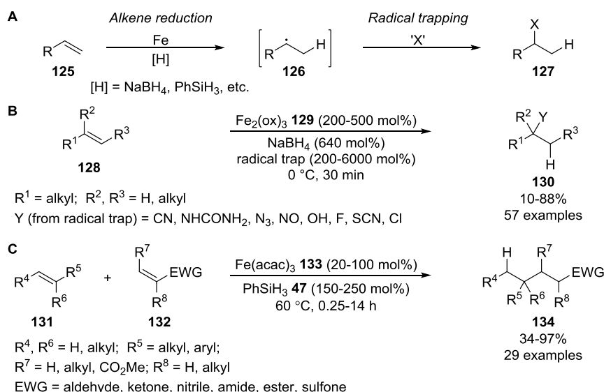
Scheme 1.20. Iron-catalysed, radical-mediated hydrofunctionalisation of alkenes. A General scheme; B Broad-scope hydrofunctionalisation using a range of radical traps; C Reductive cross-coupling of alkenes.
