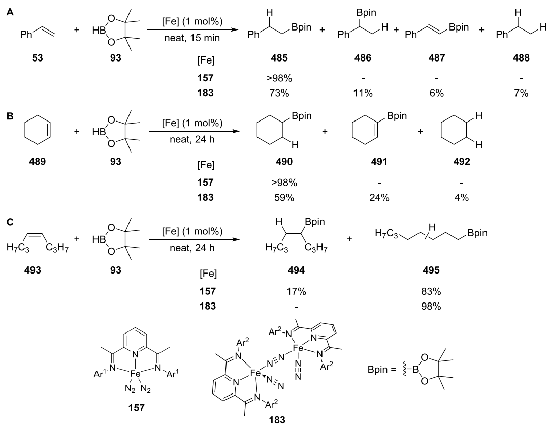
Scheme 3.04. Selectivity differences in the hydroboration of styrene and 1,2-disubstituted alkenes using bis(imino)pyridine iron bis(dinitrogen) complexes 157 and 183 .
