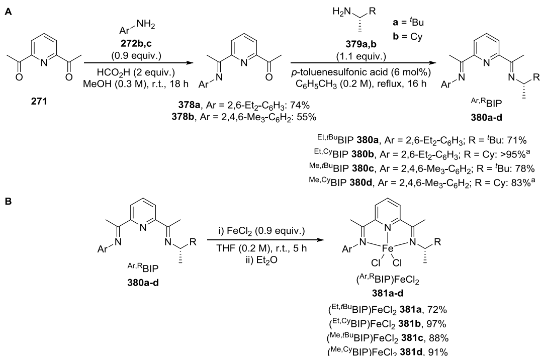
Scheme 2.19. Synthesis of enantiopure bis(imino)pyridine iron(II) chloride complexes 381a-d .
