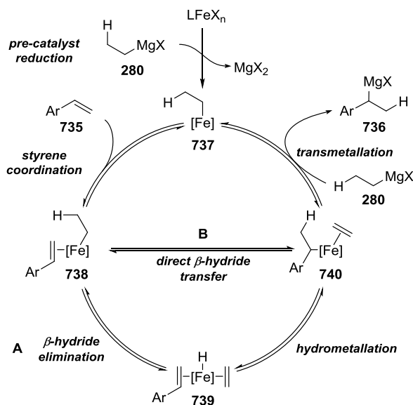
Scheme 4.21. Proposed mechanism of iron-catalysed hydromagnesiation.
