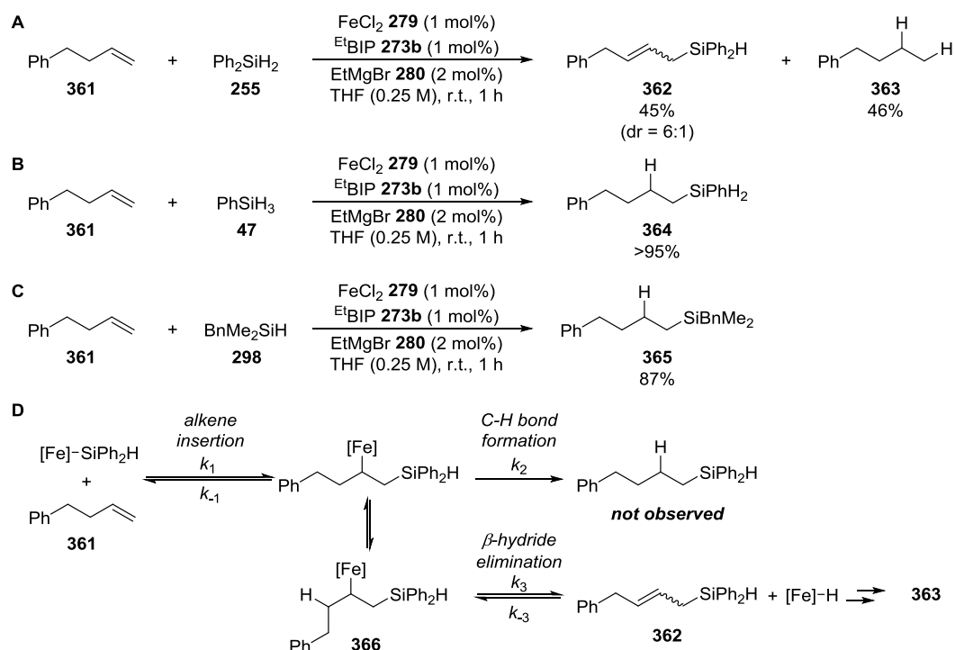
Scheme 2.16. Hydrosilylation of 4-phenylbutene 361 using primary, secondary and tertiary silanes.
