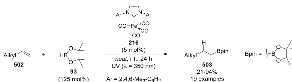
Scheme 3.06. Hydroboration of terminal alkenes using iron carbene tetracarbonyl complex [(\text{IMes})\text{Fe}(\text{CO})_4] 216 , activated using continual near-UV irradiation ( \lambda = 350 \text{ nm} ).
