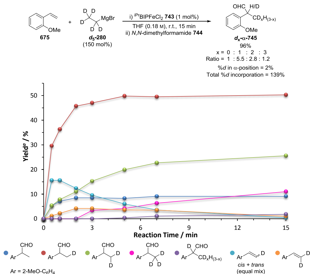
Figure 4.06. Hydromagnesiation of 2-methoxystyrene 675 using d_5 -ethylmagnesium bromide d 5 -280 . a Yield determined by 1 H NMR spectroscopy using 1,3,5-trimethoxybenzene as an internal standard.
