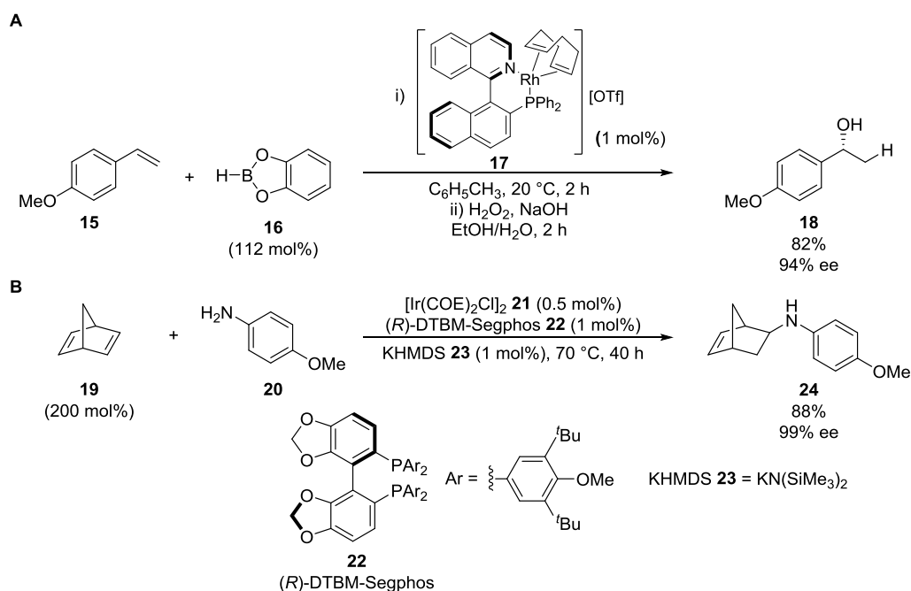
Scheme 1.06. Asymmetric hydrofunctionalisation reactions with potential application in fine chemical synthesis: A Rhodium-catalysed hydroboration-oxidation of aryl alkenes; B Iridium-catalysed hydroamination of norbornadiene.
