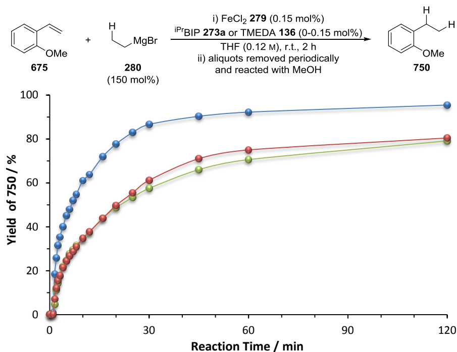
Figure 4.15. Hydromagnesiation of 2-methoxystyrene 675 using different iron pre-catalysts ([Fe] = 1.8 \times 10^{-3} M). ● = FeCl 2 279 + i PrBIP 273a (0.15 mol%); ● = FeCl 2 279 ; ● = FeCl 2 279 + TMEDA 136 (0.15 mol%).
