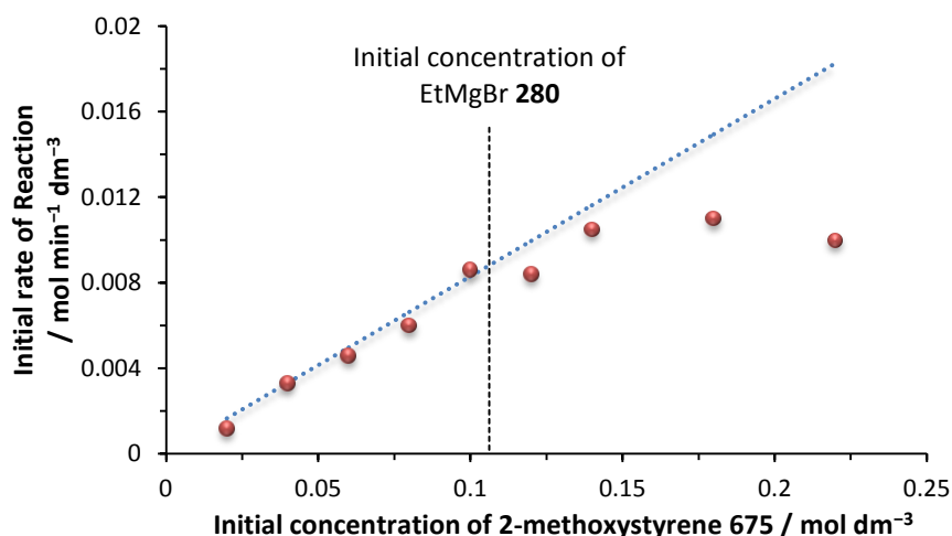
Figure 4.12. Initial rate of reaction dependence on concentration of 2-methoxystyrene 675 .
