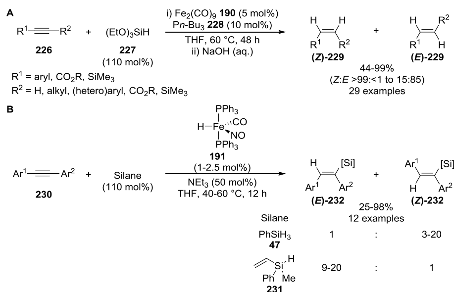
Scheme 2.02. Hydrosilylation of alkynes using iron carbonyl complexes as pre-catalysts. A Using a catalyst combination of \text{Fe}_2(\text{CO})_9 190 and tributylphosphine 228 ; B Using (nitroso)iron hydride complex [\text{FeH}(\text{CO})\text{NO}(\text{PPh}_3)_2] 191 as pre-catalyst.
