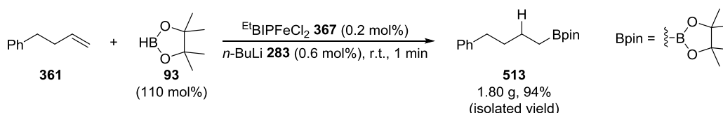
Scheme 3.12. Gram-scale hydroboration of 4-phenylbutene 361 under ‘solvent-free’ conditions.
