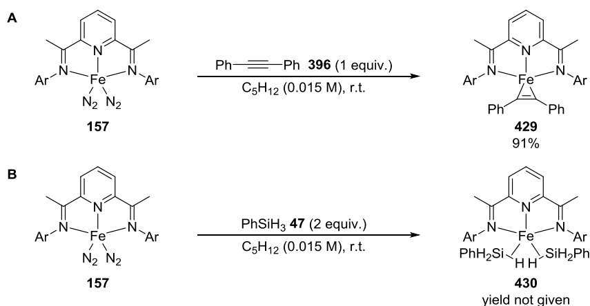
Scheme 2.30. Stoichiometric reactions of bis(imino)pyridine iron bis(dinitrogen) complex 157 with phenylacetylene 396 and phenylsilane 47 to give iron complexes 429 and 430 , respectively.
