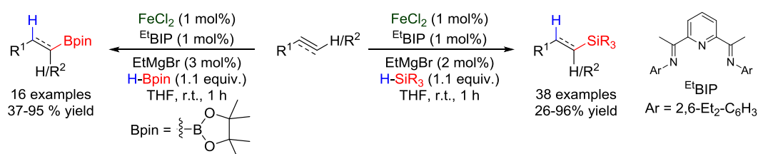
Scheme A1. Iron-catalysed hydrosilylation and hydroboration of alkenes and alkynes
