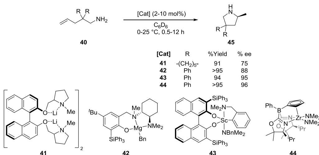
Scheme 1.09. Enantioselective intramolecular hydroamination using a selection of catalysts based upon metals from groups 1-4 bearing enantiopure nitrogen and oxygen-based ligands.
