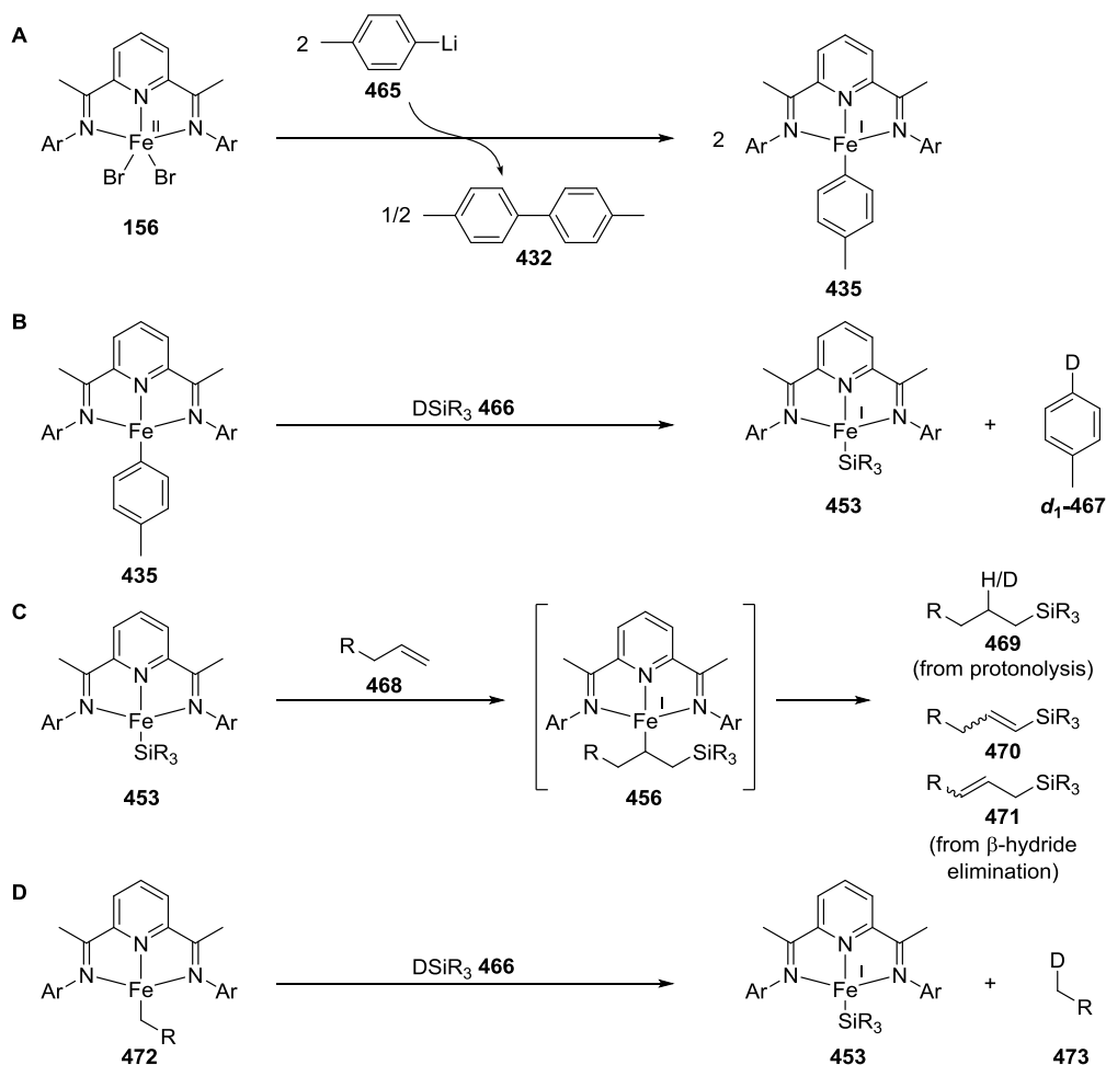
Scheme 2.39. Proposed stoichiometric reactions of isolated iron complexes to validate or disprove each step of the proposed catalytic cycle.
