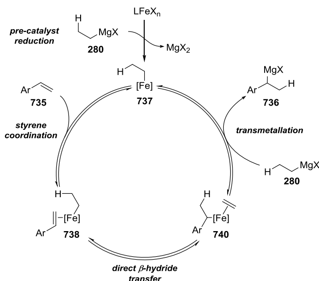
Scheme 4.32. Proposed mechanism for the iron-catalysed hydromagnesiation of styrene derivatives 735 using ethylmagnesium bromide 280 .
