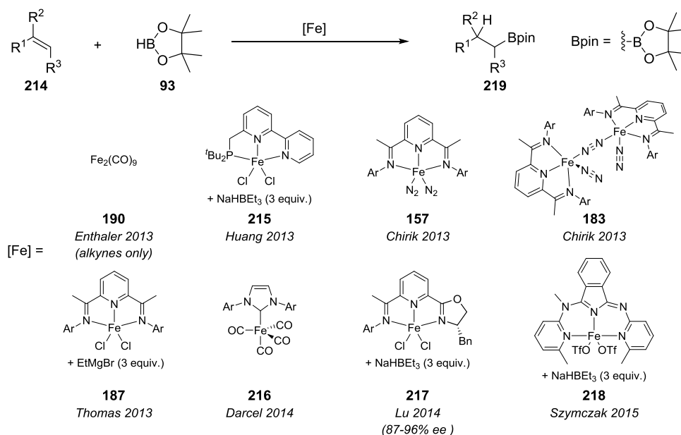
Scheme 1.28. Iron catalysts reported by different research groups for the iron-catalysed hydroboration of alkenes and alkynes.
