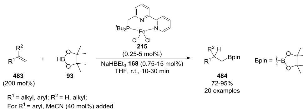
Scheme 3.03. Hydroboration of terminal and 1,1-disubstituted alkenes 483 using a PNN iron(II) pre-catalyst 215 reduced in situ using sodium triethylborohydride 168 .
