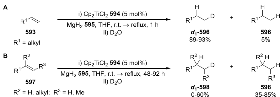
Scheme 4.02. Hydromagnesiation of terminal alkenes ( A ) and disubstituted alkenes ( B ) using magnesium hydride 595 and bis(cyclopentadienyl)titanium dichloride 594 ( \text{Cp}_2\text{TiCl}_2 ).
