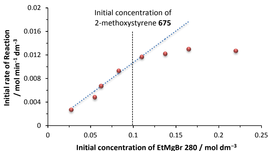
Figure 4.13. Initial rate of reaction dependence on concentration of ethylmagnesium bromide 280 .
