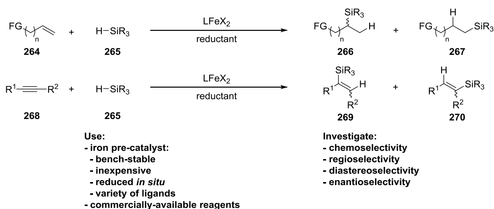
Scheme 2.09. Proposed development of iron-catalysed hydrosilylation methodology.
