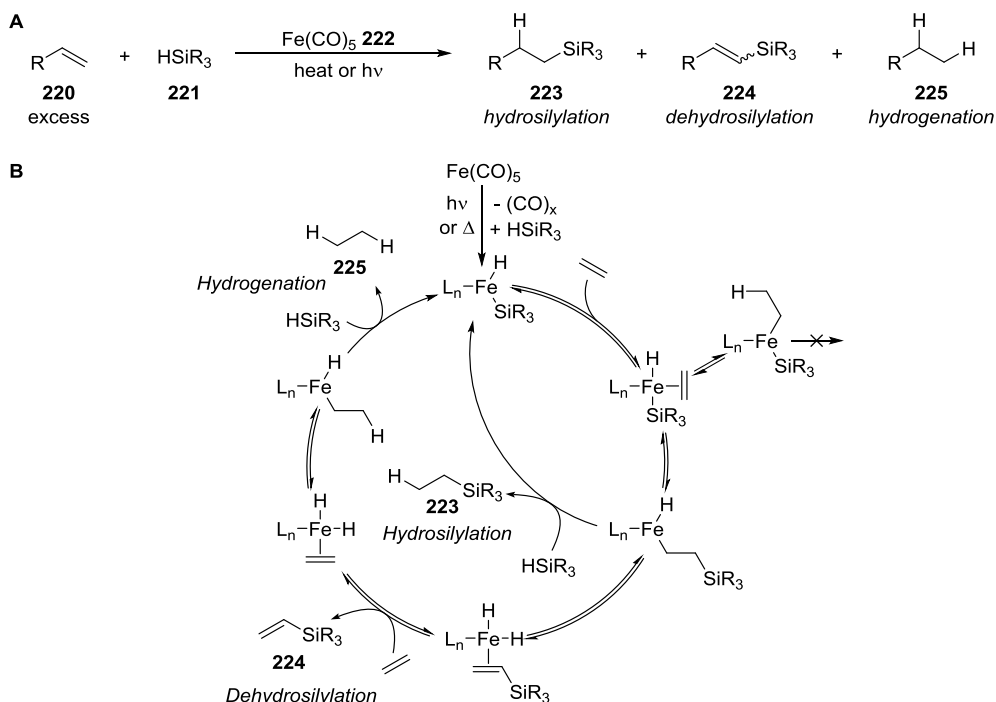
Scheme 2.01. Iron-catalysed hydrosilylation of alkenes using iron pentacarbonyl as a pre-catalyst. A General reaction scheme; B ‘Modified Chalk-Harrod’ mechanism proposed by Wrighton.
