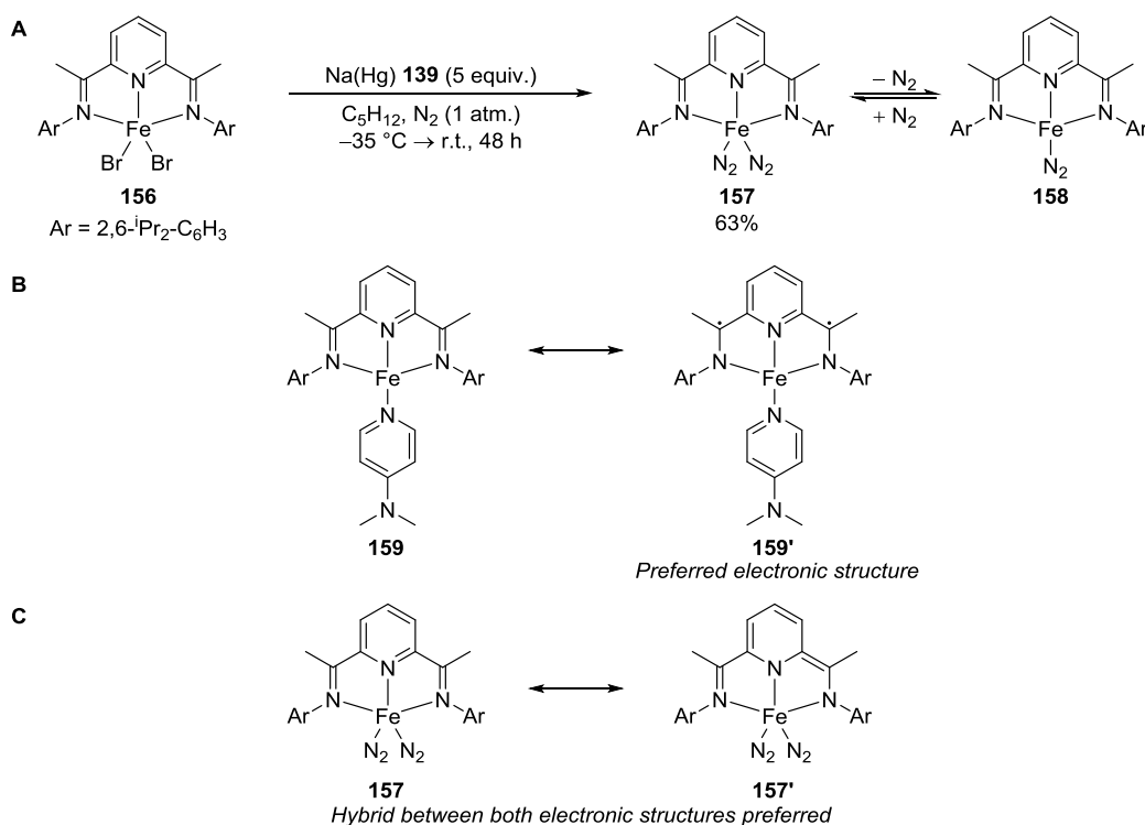
Scheme 1.22. Redox chemistry of bis(imino)pyridine (BIP) complexes. A Sodium amalgam 139 reduction of iron(II) bromide complex 156 to give bis(imino)pyridine iron dinitrogen complexes 157 and 158 ; B Electronic resonance structures of four-coordinate bis(imino)pyridine iron DMAP complex 159 and 159' (DMAP = 4-dimethylaminopyridine); C Electronic resonance structures of bis(imino)pyridine iron bis(dinitrogen) complex 157 and 157' .
