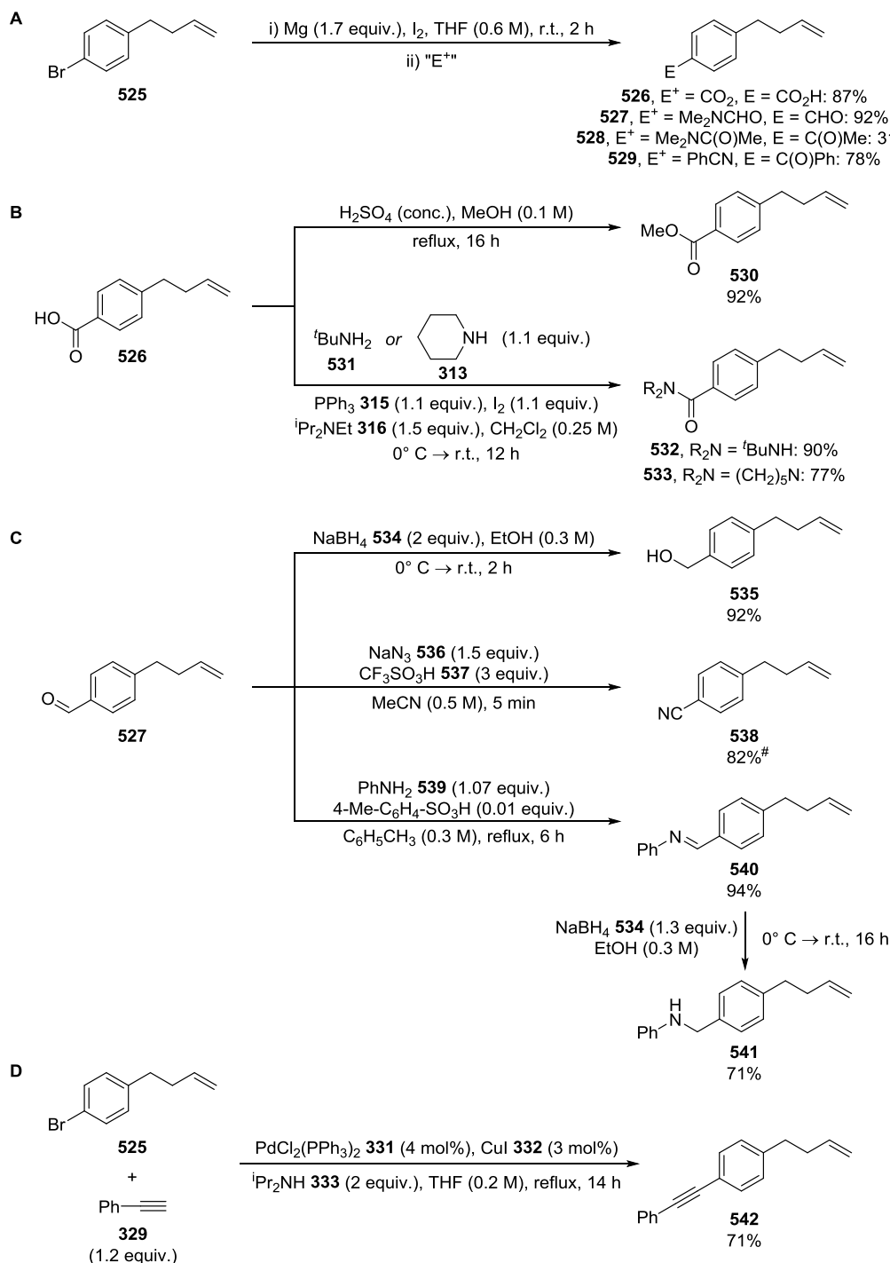
Scheme 3.11. Synthesis of 4-phenylbutene derivatives 526-530 , 532 , 533 , 535 , 538 and 540-542 . # approx. 15% internal alkene isomers also obtained.
