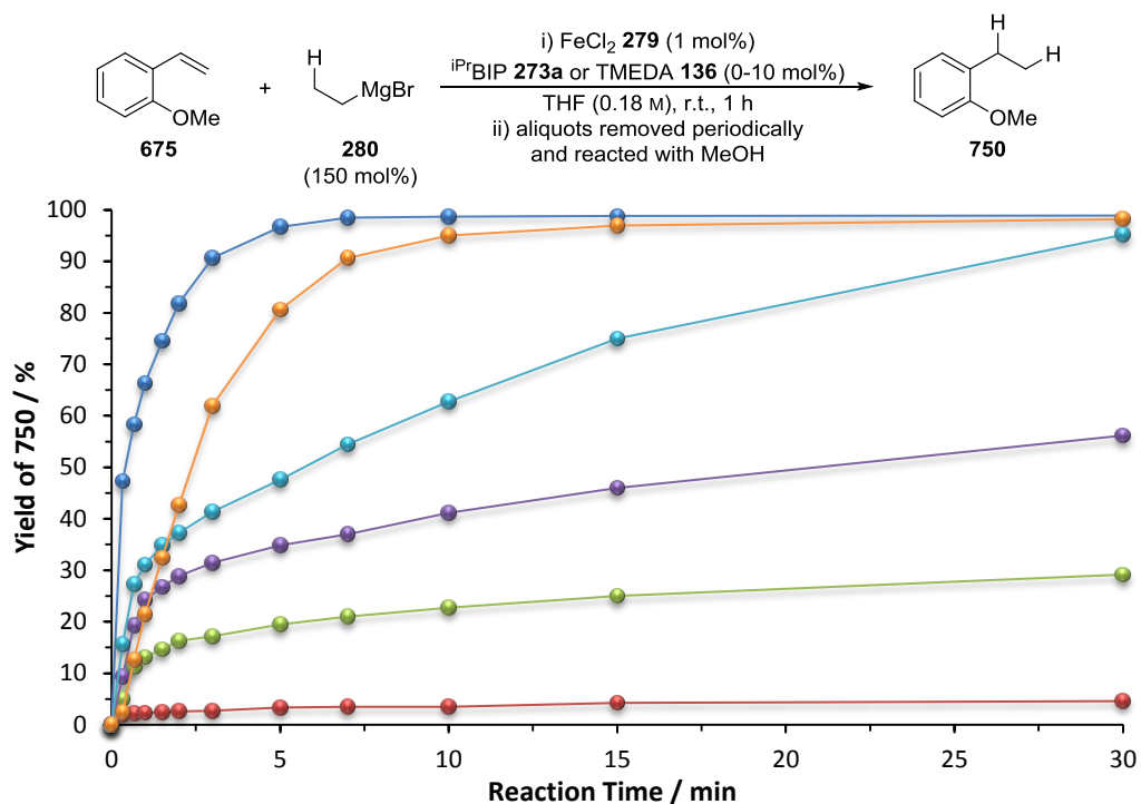
Figure 4.14. Hydromagnesiation of 2-methoxystyrene 675 using different iron pre-catalysts ([Fe] = 1.8 \times 10^{-3} M). ● = FeCl 2 279 + iPrBIP 273a (1 mol%); ● = FeCl 2 279 ; ● = FeCl 2 279 + TMEDA 136 (0.5 mol%); ● = FeCl 2 279 + TMEDA 136 (1 mol%); ● = FeCl 2 279 + TMEDA 136 (2 mol%); ● = FeCl 2 279 + TMEDA 136 (10 mol%).
