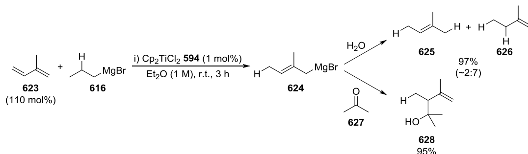
Scheme 4.07. Titanium-catalysed hydromagnesiation of isoprene 623 and subsequent reaction with electrophiles.
