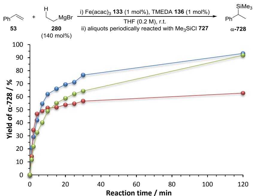
Figure 4.02. Kinetic analysis of the hydromagnesiation of styrene on a preparative scale. Conditions: Fe(acac) 3 133 (1 mol%), TMEDA 136 (1 mol%), styrene 53 (0.7 or 7 mmol), EtMgBr 280 (140 mol%), THF (0.2 M). Key: ● = 0.7 mmol scale; ● = 7 mmol scale; ● = 7 mmol scale, with continual N 2 sparge.
