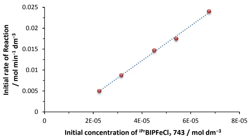
Figure 4.11. Initial rate of reaction dependence on concentration of iron pre-catalyst 743 .
