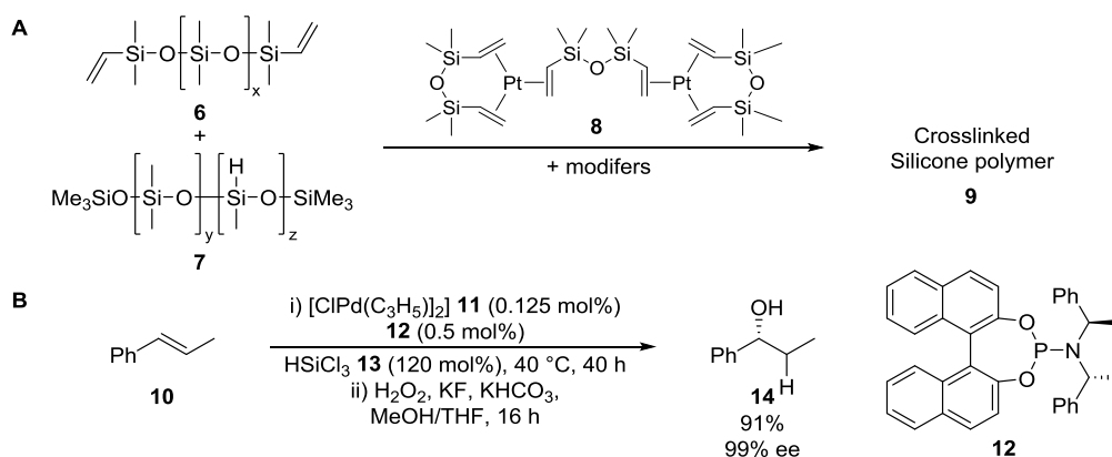
Scheme 1.05. Hydrosilylation of alkenes: A Industrial application of platinum-catalysed hydrosilylation for the synthesis of cross-linked silicone polymers; B Palladium-catalysed enantioselective hydrosilylation-oxidation of aryl alkenes.
