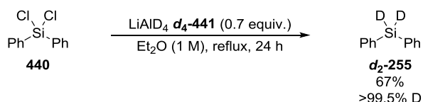
Scheme 2.34. Reduction of dichlorodiphenylsilane 440 with lithium aluminium deuteride d 4 -441 to give diphenyl(silane- d_2 ) d 2 -255 .
