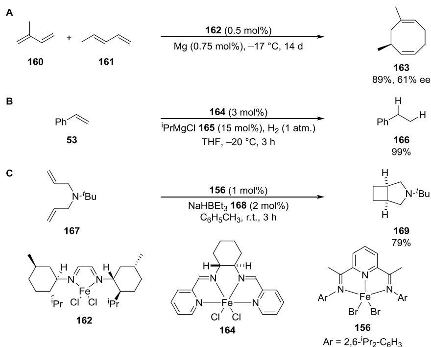
Scheme 1.23. Iron-catalysed reactions in which the active catalyst is formed in situ by reduction of an iron(II) pre-catalyst using: A Activated magnesium (1.5 equiv. with respect to iron); B iso-Propylmagnesium chloride 165 (5 equiv. with respect to iron); C Sodium triethylborohydride 168 (2 equiv. with respect to iron).
