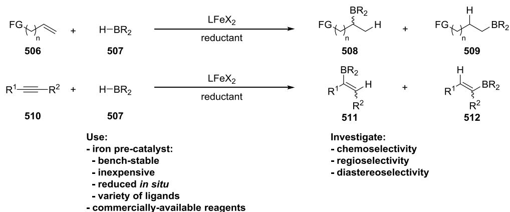
Scheme 3.09. Proposed development of iron-catalysed hydroboration methodology.
