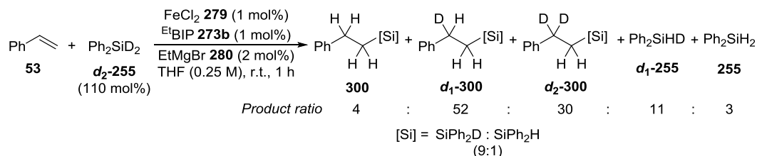
Scheme 2.35. Hydrosilylation of styrene 53 using diphenyl(silane- d_2 ) d 2 -255 .
