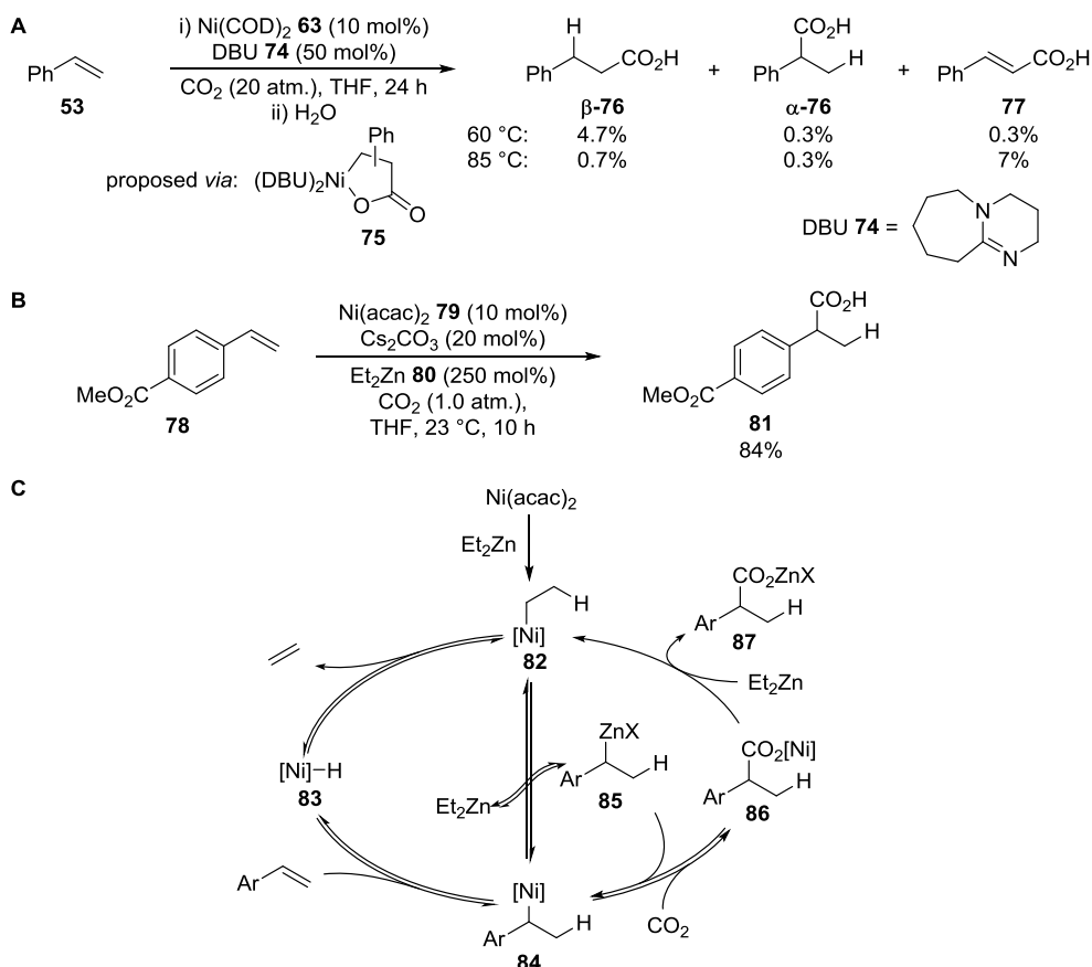
Scheme 1.14. A Nickel-mediated hydrocarboxylation and dehydrocarboxylation of styrene; B Nickel-catalysed hydrocarboxylation of styrene derivatives; C Proposed mechanism for nickel-catalysed hydrocarboxylation of styrene derivatives.
