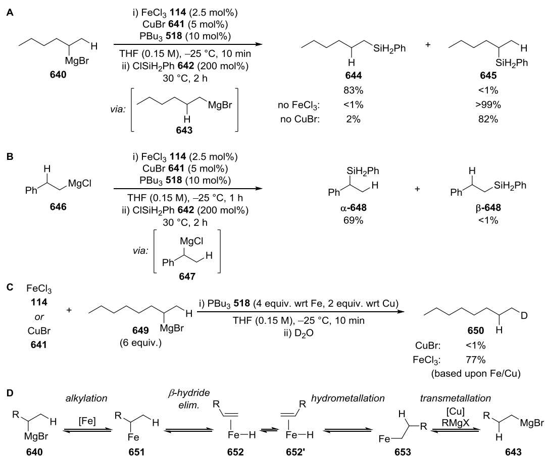
Scheme 4.11. Isomerisation of alkyl Grignard reagents using iron-copper cooperative catalysis. A Isomerisation of a 2-alkyl Grignard reagent 640 to a 1-alkyl Grignard reagent 643 ; B Isomerisation of a homobenzylic Grignard reagent 646 to a benzylic Grignard reagent 647 ; C Stoichiometric reactions of iron and copper salts with 2-octylmagnesium bromide 649 . D Proposed mechanism of alkyl Grignard reagent isomerisation.
