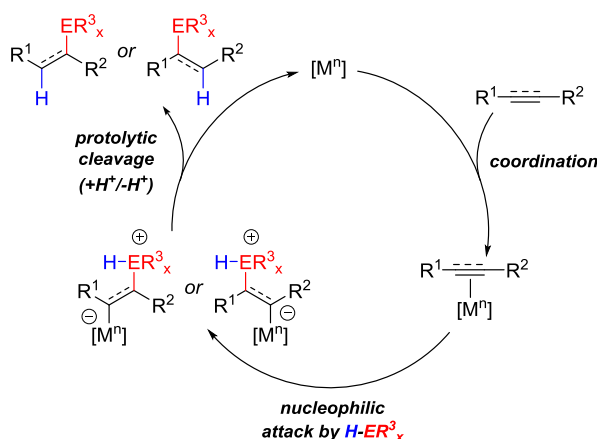
Scheme 1.02. Hydrofunctionalisation of alkenes and alkynes through coordination to a transition-metal catalyst and external attack by a nucleophilic hydrofunctionalisation reagent ( H-ER^3_x ).
