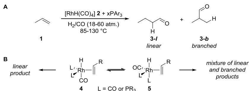
Scheme 1.04. A General conditions used for the hydroformylation of propene; B Isomeric trigonal bipyramidal rhodium complexes leading to linear and branched aldehyde products.
