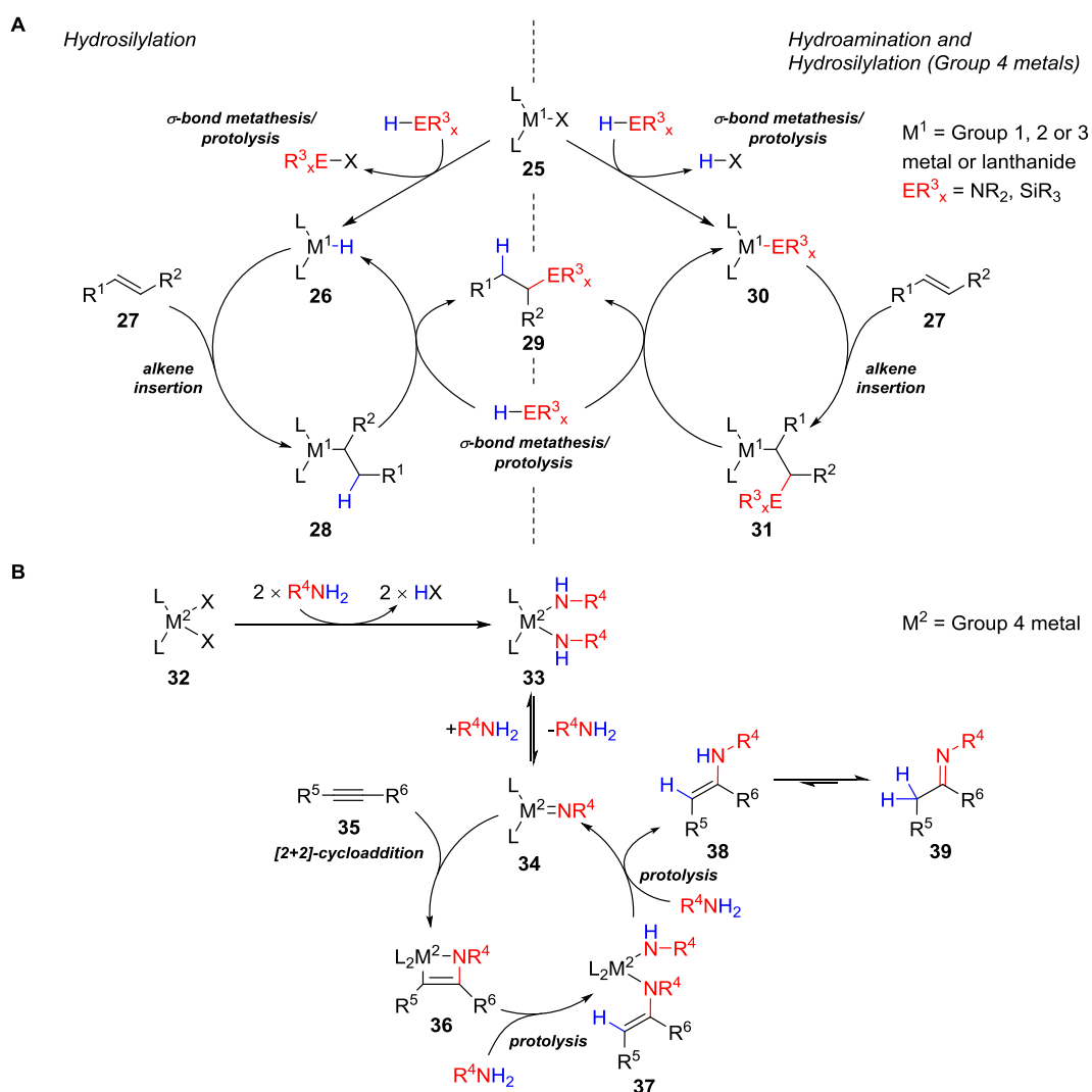
Scheme 1.08. Mechanisms of alkene and alkyne hydrofunctionalisation using metal catalysts with a d^0 electronic configuration. A ‘Alkene insertion mechanism’ proposed for the hydroamination and hydrosilylation of alkenes using groups 1-3, and lanthanide, metal catalysts; B ‘Imido mechanism’ proposed for the hydroamination of alkynes using group 4 metal catalysts.
