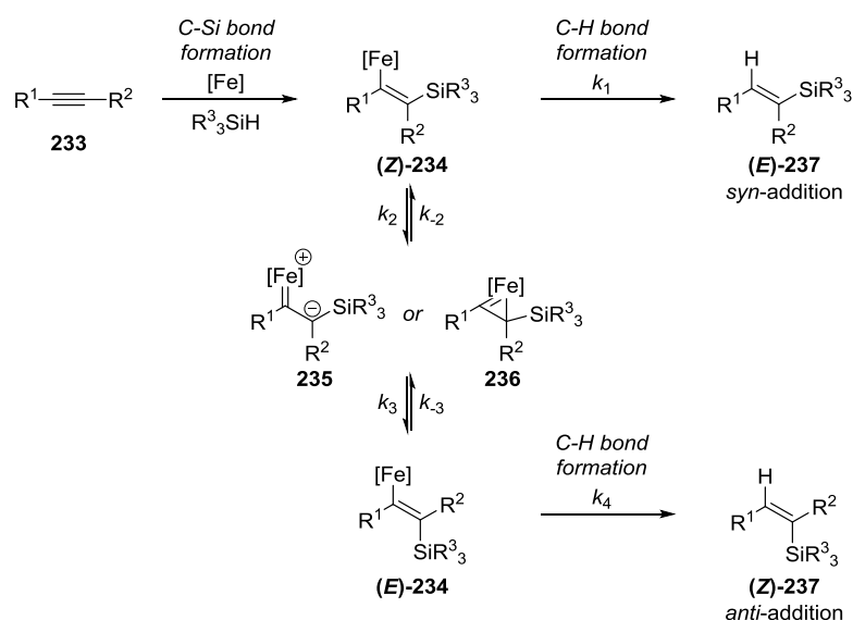
Scheme 2.03. Possible mechanism to explain the stereochemical outcome of iron-catalysed hydrosilylation of alkynes.
