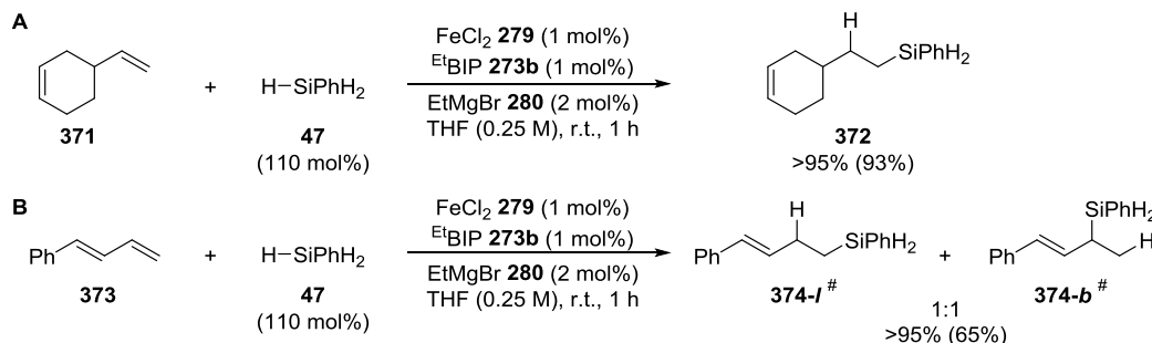
Scheme 2.17. Chemoselective hydrosilylation of the terminal alkene of diene substrates 371 and 373 . # = Result obtained by Dominik Frank
