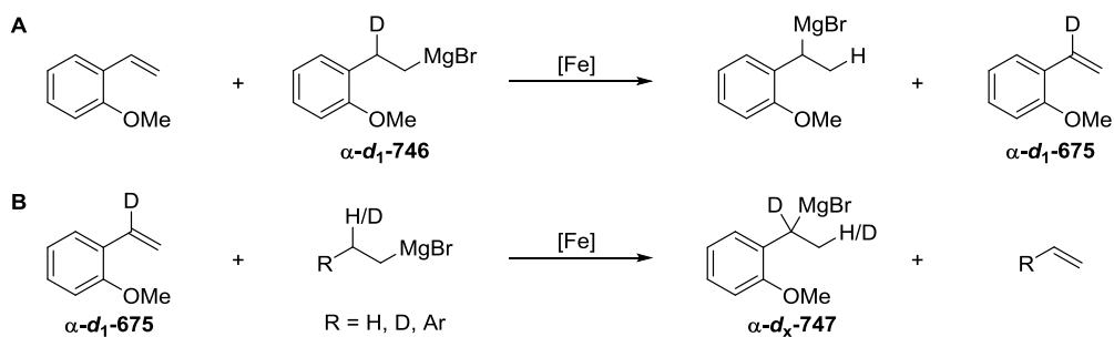
Scheme 4.23. Proposed pathway to explain the formation of an \alpha -aryl Grignard reagent \alpha\text{-d}_x\text{-747} with deuterium incorporation in the \alpha -aryl position.
