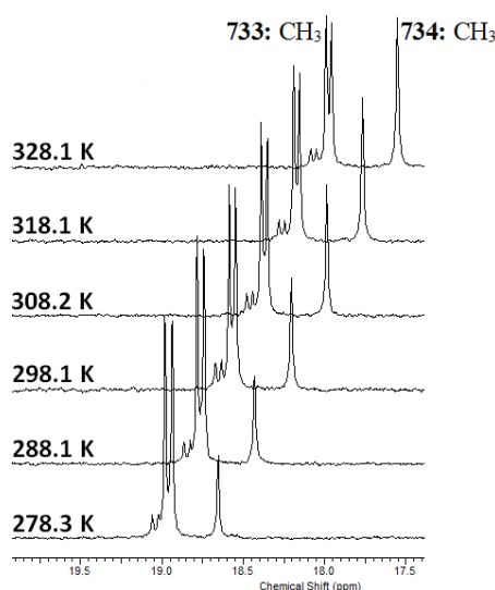
Figure 4.04. Variable temperature ^{13}\text{C} NMR spectra of methyl carbons of benzylic Grignard reagent 734 and dibenzylmagnesium 733 .
