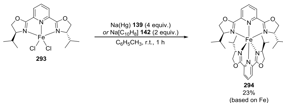
Scheme 2.11. Reduction of i PrPybox iron(II) chloride complex 293 using sodium amalgam 139 or sodium naphthalide 142 to give catalytically-inactive ( i PrPybox) 2 Fe(0) complex 294 .
