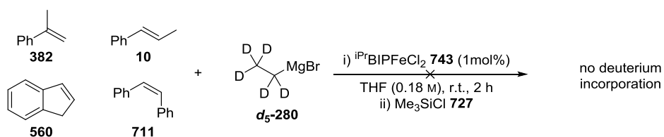
Scheme 4.27. Attempted hydromagnesiation of disubstituted styrene derivatives using deuterated ethylmagnesium bromide d 5 -280 .
