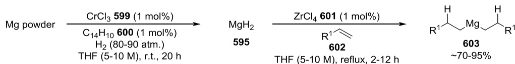
Scheme 4.03. Hydrogenation of magnesium using a mixed pre-catalyst system of chromium(III) chloride 599 and anthracene 600 to give activated magnesium hydride 595 , and subsequent hydromagnesiation of terminal alkenes 602 using zirconium(IV) chloride 601 as a pre-catalyst.
