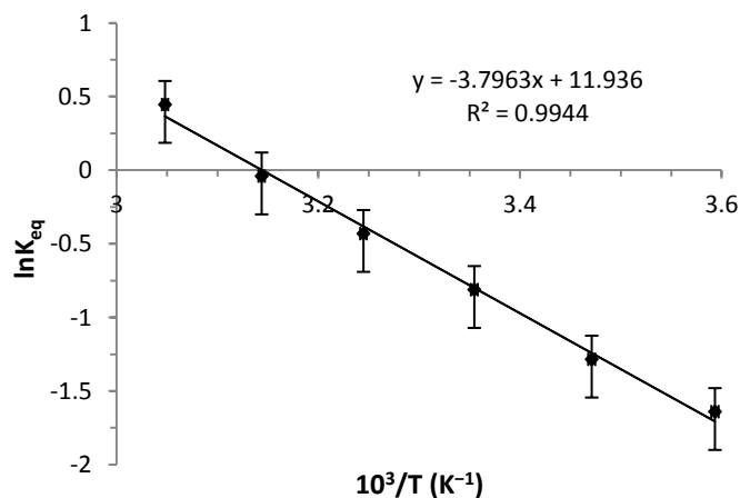
Figure 4.05. van't Hoff plot of \ln K_{eq} vs. 10^3/T for the reaction \text{MgBr}_2 732 + \text{R}_2\text{Mg} 733 \rightleftharpoons 2 \times \text{RMgBr} 734 ( \text{R} = \text{CH}(\text{CH}_3)\text{Ph} ).
