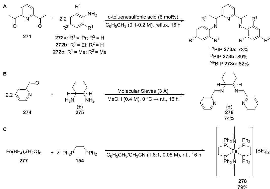
Scheme 2.10. Synthesis of iminopyridine-based ligands 273a-c and 276 through condensation reactions ( A and B ) and iron(II) bis[1,2-bis(diphenylphosphino)ethane] complex 278 ( C ).
