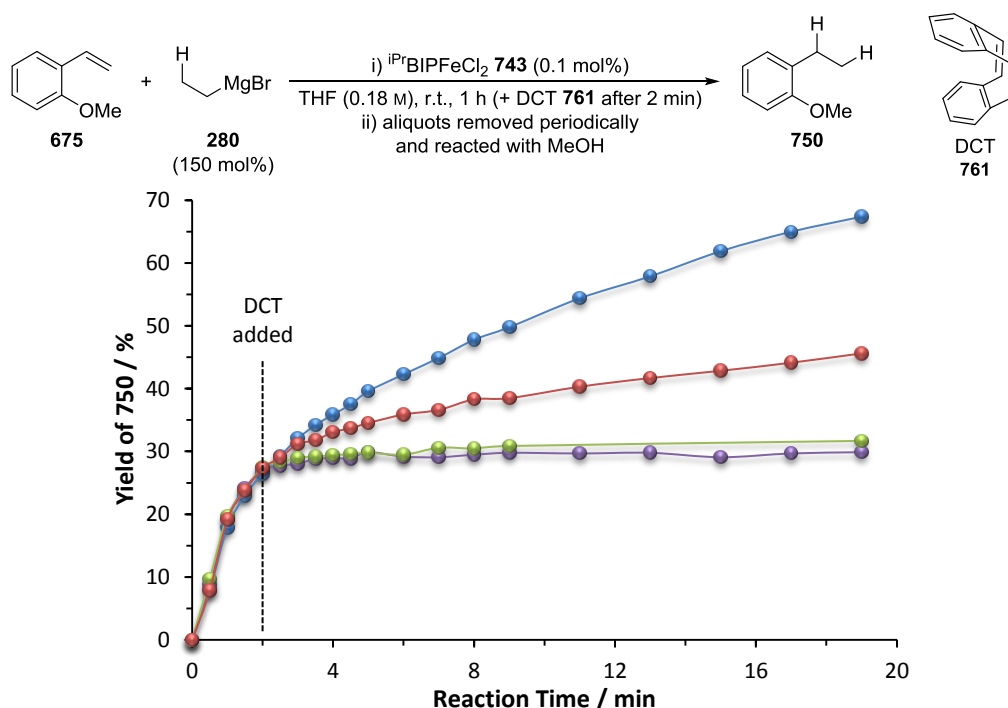
Figure 4.16. Hydromagnesiation of 2-methoxystyrene 675 in the absence and presence of DCT 761 . ● = no DCT 761 added; ● = DCT 761 (0.05 mol%) added after 2 minutes; ● = DCT 761 (0.1 mol%) added after 2 minutes; ● = DCT 761 (0.2 mol%) added after 2 minutes.
