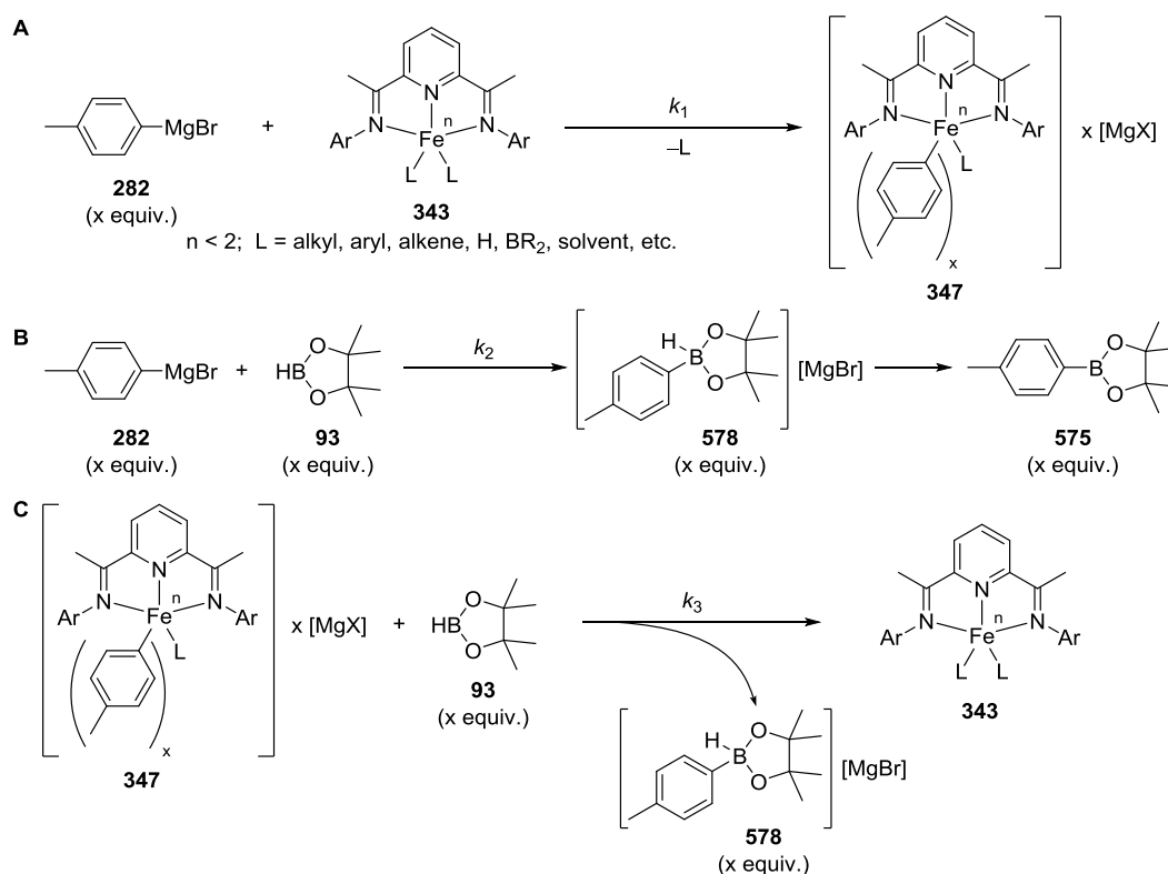
Scheme 3.16. A Formation of proposed catalytically-inactive iron-ate complex 347 in the presence of excess p -tolylmagnesium bromide 282 ; B Reaction of p -tolylmagnesium bromide 282 with pinacol borane 93 ; C Regeneration of ‘active catalyst’ 343 through reaction of iron-ate complex 347 with pinacol borane 93 .
