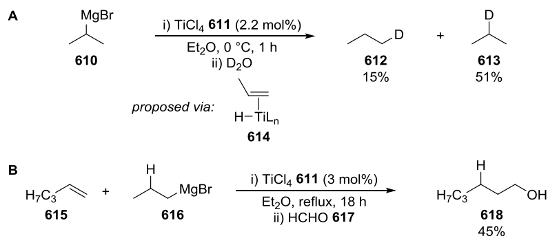
Scheme 4.05. A Titanium-catalysed isomerisation of alkyl Grignard reagents bearing \beta -hydrogen atoms. B Titanium-catalysed hydromagnesiation of 1-pentene 615 using n -propylmagnesium bromide 616 .
