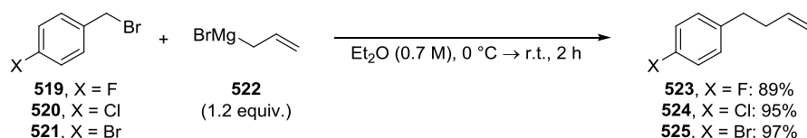
Scheme 3.10. Synthesis of halide-substituted 4-phenylbutene derivatives 523-525 .
