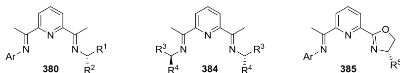
Figure 2.01. Enantiopure C_1 - and C_2 -symmetric iminopyridine-based ligand structures which may be investigated for the development of asymmetric iron-catalysed hydrosilylation.
