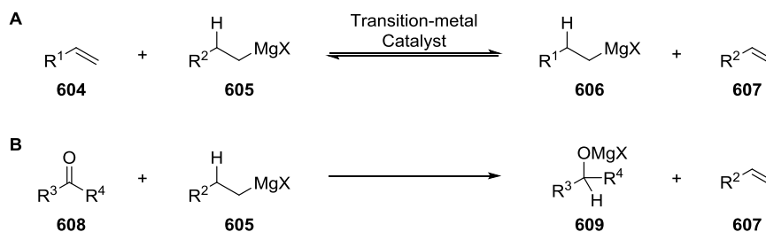
Scheme 4.04. A Transition-metal-catalysed hydromagnesiation of alkenes 604 using a Grignard reagent bearing \beta -hydrogen atoms 605 ; B Meerwein–Ponndorf–Verley-type reduction of ketones 608 using a Grignard reagent bearing \beta -hydrogen atoms 605 .
