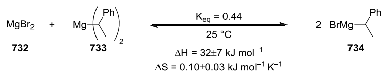
Scheme 4.19. Schlenk equilibrium between dibenzylmagnesium species 733 and magnesium bromide 732 , and benzylic Grignard reagent 734 .
