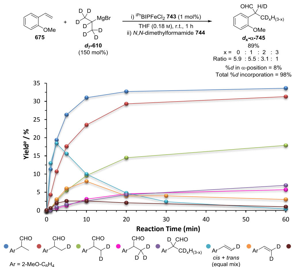
Figure 4.07. Hydromagnesiation of 2-methoxystyrene 675 using d 7 -iso-propylmagnesium bromide d 7 -610 . a Yield determined by 1 H NMR spectroscopy using 1,3,5-trimethoxybenzene as an internal standard.
