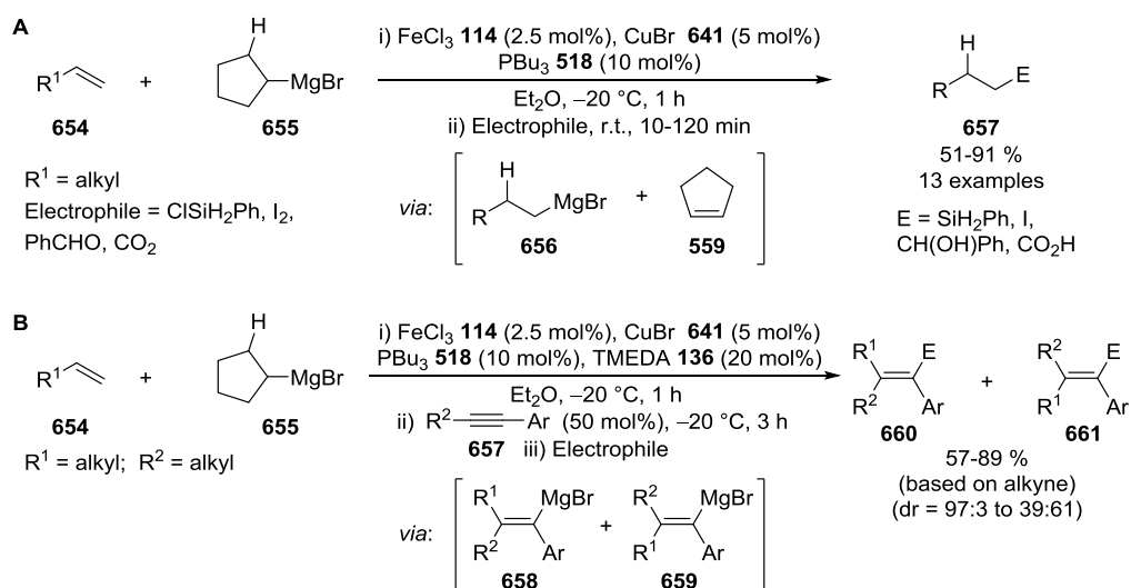
Scheme 4.12. Iron-catalysed hydromagnesiation of terminal alkenes 654 to give primary alkyl Grignard reagents 656 . A Subsequent reaction with electrophiles to give hydrofunctionalised products 657 . B Subsequent iron-catalysed addition to alkynes 657 to give tri- and tetra-substituted alkenes 660 and 661 .
