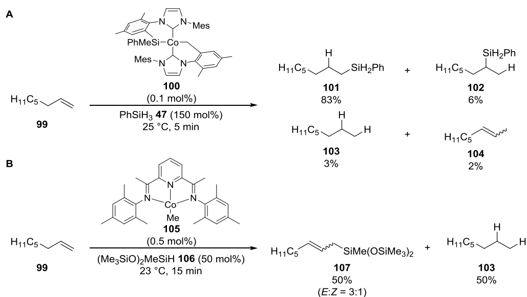
Scheme 1.17. Cobalt-catalysed hydrosilylation and dehydrosilylation of terminal alkenes.
