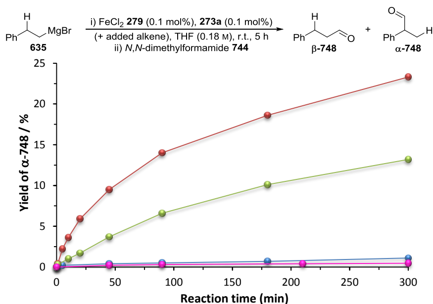
Figure 4.08. Isomerisation of \beta -aryl Grignard reagent 635 in the absence and presence of alkenes. ● = no alkene added (0.5 mol% styrene 53 present in Grignard reagent solution); ● = styrene 53 (10 mol%) added; ● = 1-octene 99 (100 mol%) added. ● = cyclopentene 559 (10 mol%), indene 560 (10 mol%), \alpha -methylstyrene 382 (10 mol%) or \beta -methylstyrene 10 (10 mol%) added. [98]
