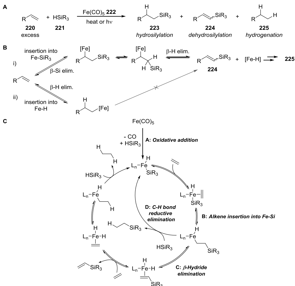
Scheme 2.28. Iron-catalysed hydrosilylation using iron pentacarbonyl as a pre-catalyst. A General reaction scheme. B Significance of alkene insertion into an iron-silicon bond for the formation of dehydrosilylation products. C Proposed hydrosilylation mechanism, with 'key steps' ( A-D ) highlighted
