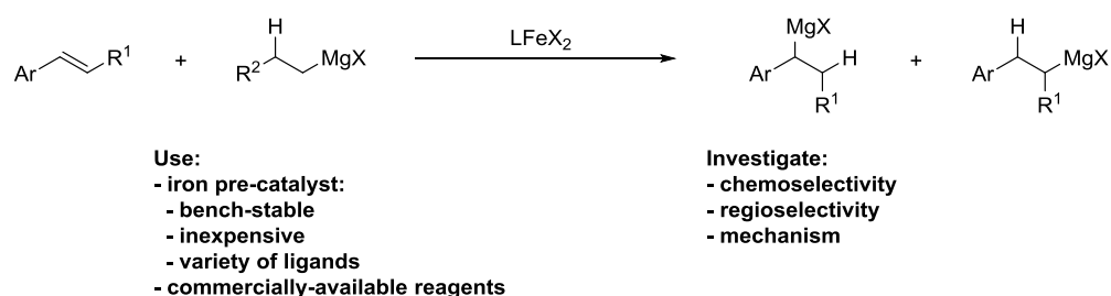
Scheme 4.15. Proposed development of iron-catalysed hydromagnesiation methodology.
