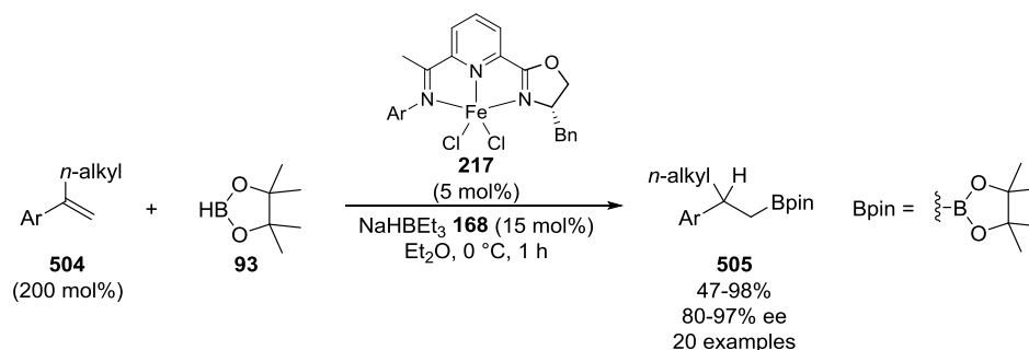
Scheme 3.07. Enantioselective hydroboration 1,1-disubstituted alkenes using an iminopyridine oxazoline iron(II) pre-catalyst 217 reduced in situ using sodium triethylborohydride.
