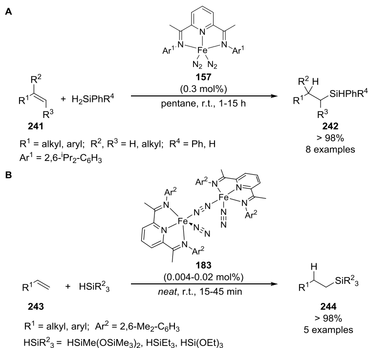
Scheme 2.05. Hydrosilylation of alkenes using bis(imino)pyridine (BIP) iron bis(dinitrogen) complexes. A Hydrosilylation using first-generation pre-catalyst; B Hydrosilylation using second-generation pre-catalyst.
