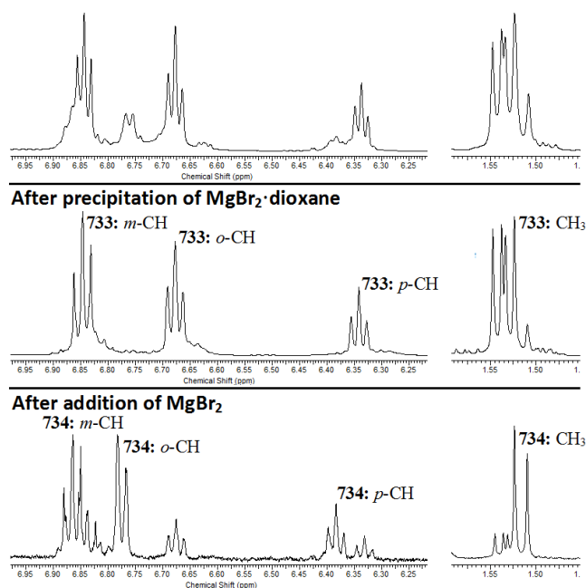
Figure 4.03. ^1\text{H} NMR spectra of benzylic Grignard reagent 734 and dibenzylmagnesium 733 at room temperature.
