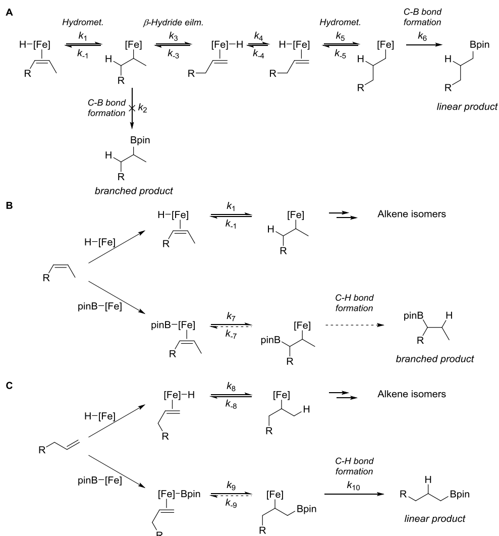
Scheme 3.18. Possible mechanisms to explain the formation of linear boronic ester products from the hydroboration of internal and terminal alkenes. A By alkene insertion into an iron-hydride bond followed by carbon-boron bond formation; B and C By alkene insertion into an iron-boron bond followed by carbon-hydrogen bond formation.
