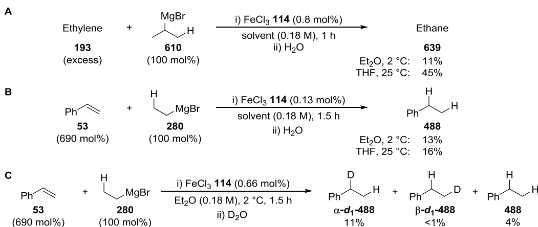
Scheme 4.10. Iron-catalysed hydromagnesiation using iron(III) chloride 114 . A Hydromagnesiation of ethylene 193 using iso-propylmagnesium bromide 610 ; B Hydromagnesiation of styrene 53 using ethylmagnesium bromide 280 ; C Hydromagnesiation of styrene 53 using ethylmagnesium bromide 280 followed by reaction with deuterium oxide.
