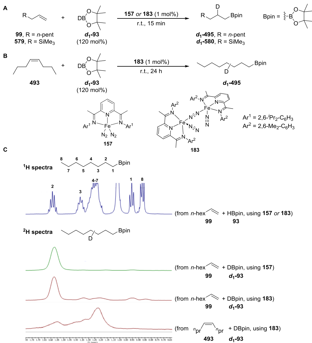
Scheme 3.17. Hydroboration of terminal ( A ) and internal ( B ) alkenes using d_1 -pinacol borane d_1 -93 and bis(imino)pyridine iron pre-catalysts 157 and 183 ; C ^1\text{H} and ^2\text{H} NMR spectra of 1-octyl pinacol boronic ester d_1 -495 from the reaction of 1-octene 99 or 4- cis -octene 493 using pinacol borane 93 or d_1 -pinacol borane d_1 -93 and bis(imino)pyridine iron pre-catalyst 157 or 183 – spectra obtained from supporting information of reference 87c.
