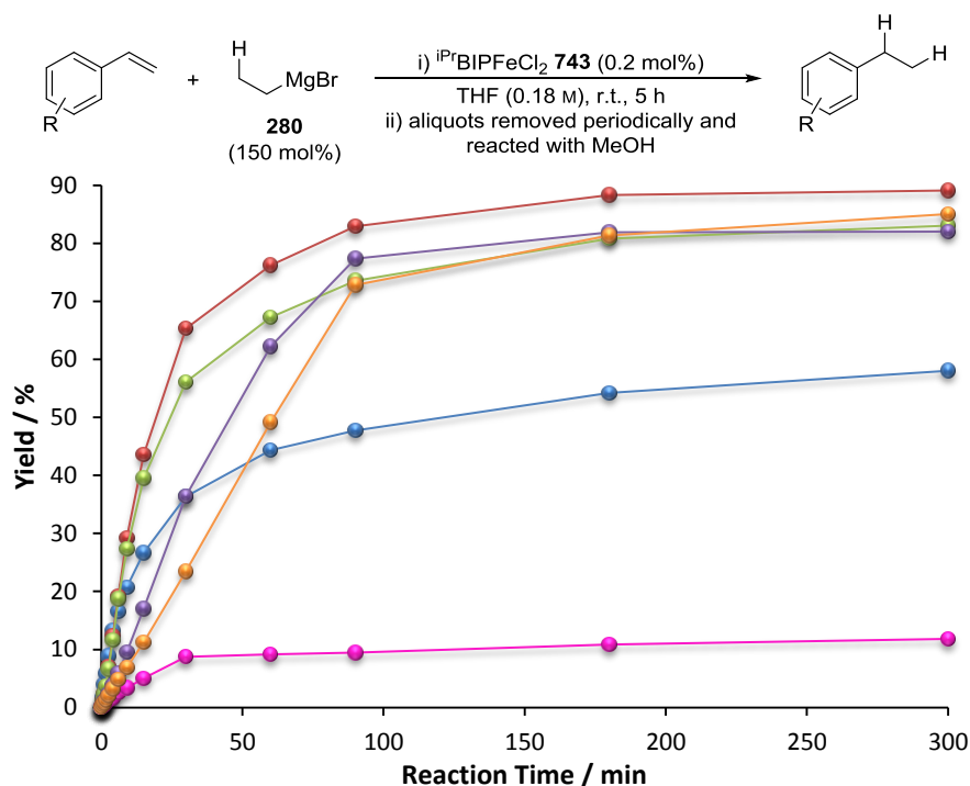
Figure 4.09. Kinetic profiles for the hydromagnesiation of a selection of electronically-differentiated styrene derivatives. ● = 4-Methoxystyrene; ● = 4- tert -butylstyrene; ● = 4-methylstyrene; ● = styrene; ● = 4-fluorostyrene; ● = 3-methoxystyrene.
