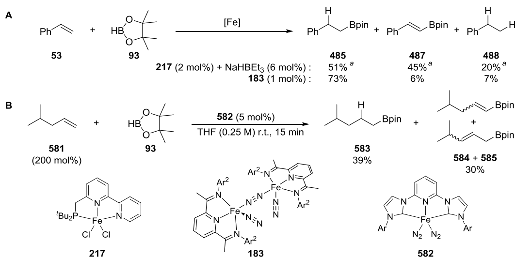
Scheme 3.19. The formation of vinyl boronic ester side-products in iron-catalysed hydroboration of alkenes using a selection of different iron pre-catalysts. a Yield based on styrene 53 (200 mol% used).
