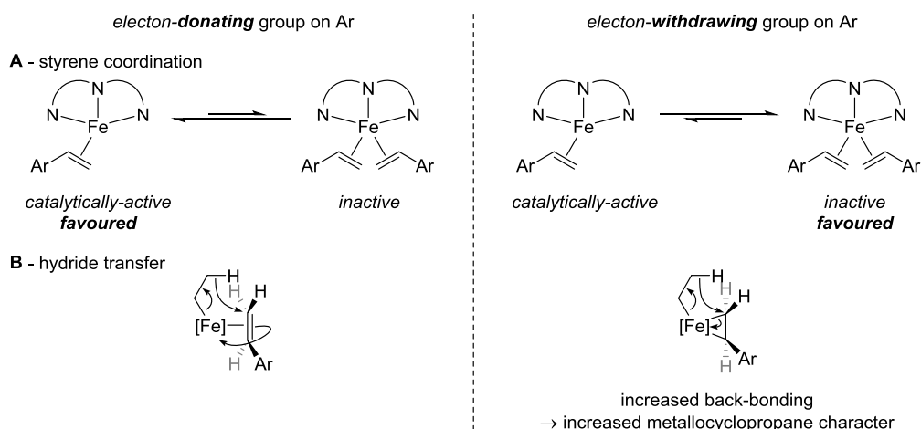
Scheme 4.26. Two possible explanations for the negative \rho value calculated for the hydromagnesiation of electronically-differentiated styrene derivatives.
