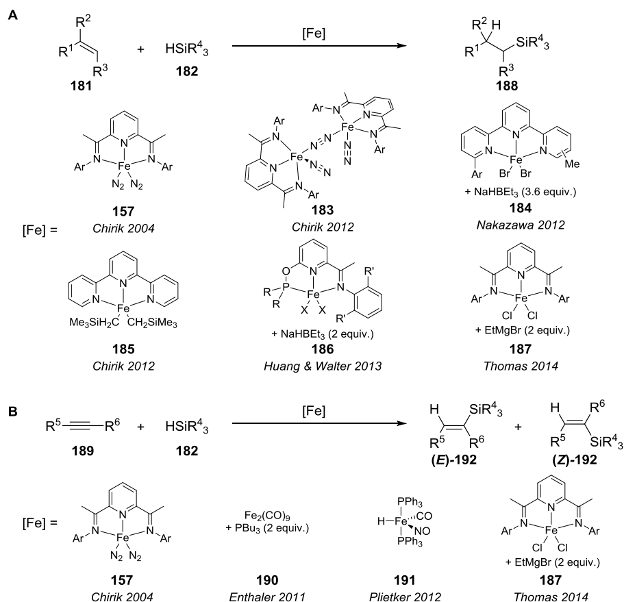
Scheme 1.25. Iron catalysts reported by different research groups for the iron-catalysed hydrosilylation of alkenes (A) and alkynes (B).
