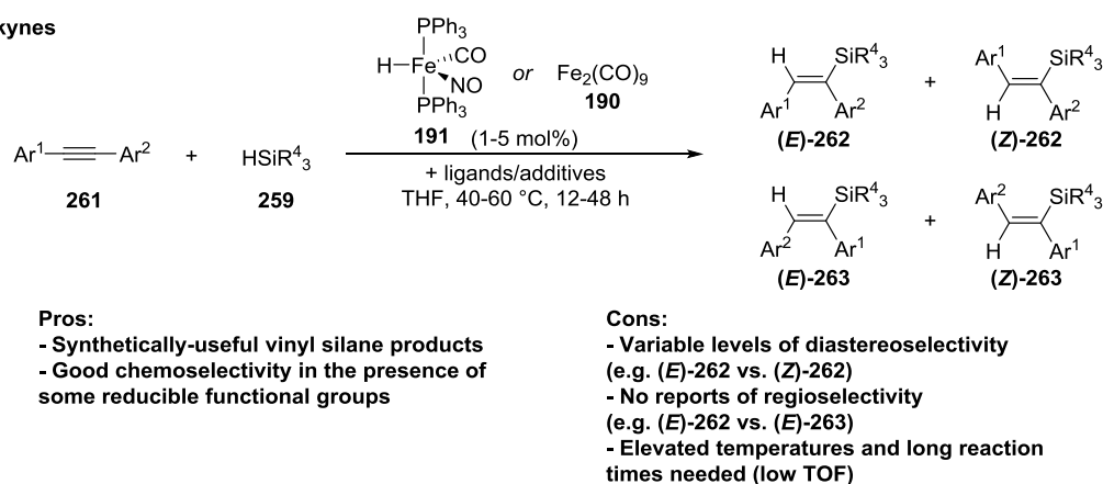
Scheme 2.08. State of the art iron-catalysed hydrosilylation methodologies in early 2012.
