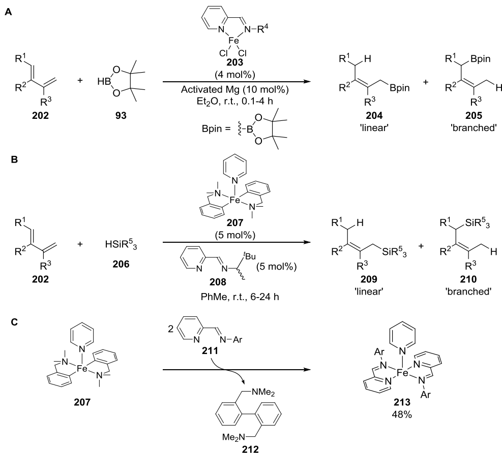
Scheme 1.27. Iron-catalysed 1,4-hydrofunctionalisation of 1,3-dienes using an iminopyridine iron catalyst. A Hydroboration using pinacol borane; B Hydrosilylation using tertiary silanes; C Reduction of iron(II) pre-catalyst 207 through carbon-carbon bond reductive elimination.
