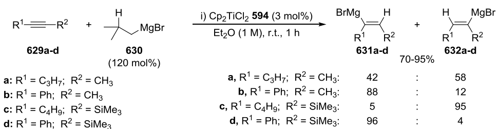
Scheme 4.08. Regioselectivity in the titanium-catalysed hydromagnesiation of unsymmetrically-substituted alkynes 629a-d . Ratio of vinyl Grignard reagents 631a-d and 632a-d inferred by analysis of products formed following reaction with electrophiles (I 2 , D 2 O, CH 3 I).
