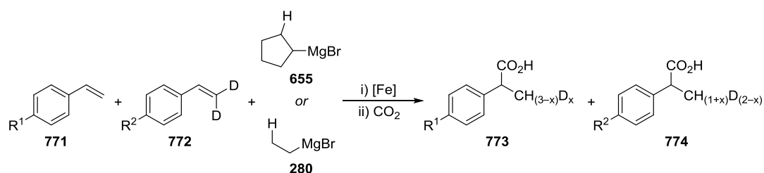
Scheme 4.33. Proposed deuterium scrambling in pseudo isotope/deuterium labelling experiment.
