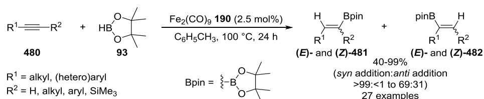
Scheme 3.02. Hydroboration of terminal and internal alkynes 480 using an iron carbonyl cluster pre-catalyst \text{Fe}_2(\text{CO})_9 190 .
