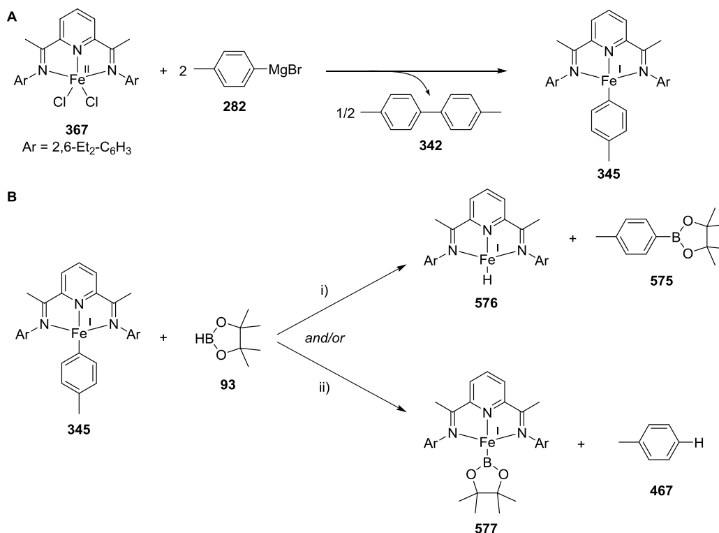
Scheme 3.15. A Reduction of iron(II) pre-catalyst Et BIPFeCl 2 367 using p -tolylmagnesium bromide 282 to give iron(I) aryl complex 345 ; B Possible reaction of iron(I) aryl complex 345 with pinacol borane 93 to give iron(I) hydride or boryl complexes 576 and 577 .
