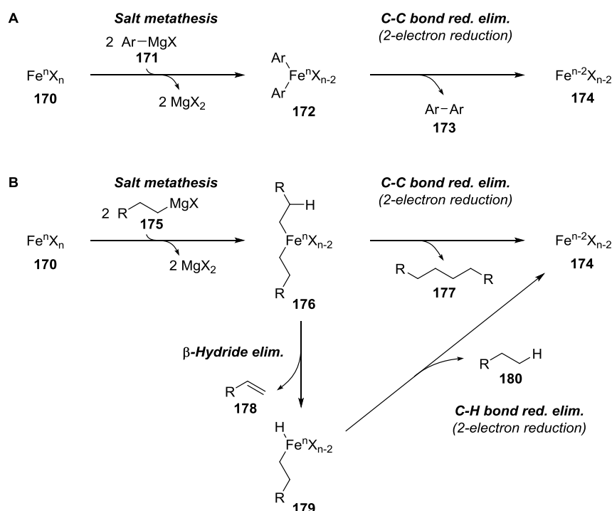
Scheme 1.24. Reduction of iron salts 170 using Grignard reagents: A Reduction pathway using arylmagnesium halides 171 ; B Competing reduction pathways using alkylmagnesium halides bearing \beta -hydrogen atoms 175 .
