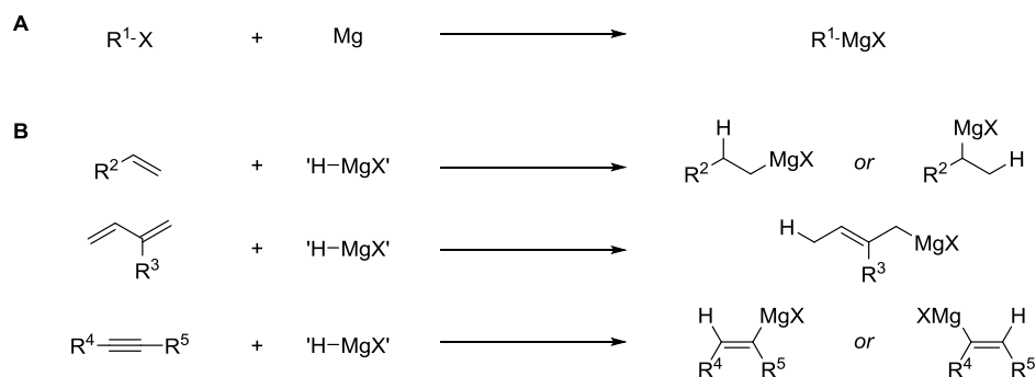
Scheme 4.01. Methods for the synthesis of Grignard reagents. A Insertion of magnesium in a carbon-halide bond; B Hydromagnesiation of alkenes, dienes and alkynes.
