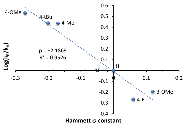
Figure 4.10. Hammett plot using electronically-differentiated 4- and 3-substituted styrene derivatives.
