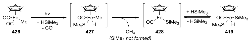
Scheme 2.29. Stoichiometric reactions of pentamethylcyclopentadienyl iron carbonyl complexes to demonstrate each of the 'key steps' (A-D) highlighted in Scheme 2.28 C.
