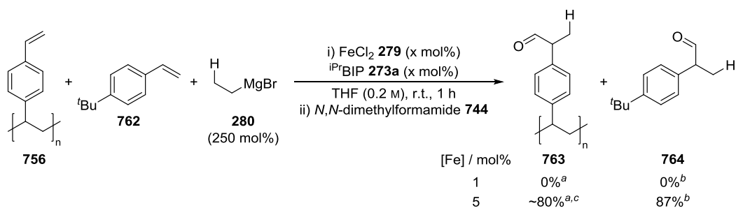
Scheme 4.30. Hydromagnesiation of polymer-bound styrene 756 using ethylmagnesium bromide 280 , in the presence of tert -butylstyrene 762 . a Formation determined by IR spectroscopy; b Yield determined by 1 H NMR spectroscopy using 1,3,5-trimethoxybenzene as an internal standard; c Conversion determined using high resolution magic angle spinning (HRMAS) NMR spectroscopy.
