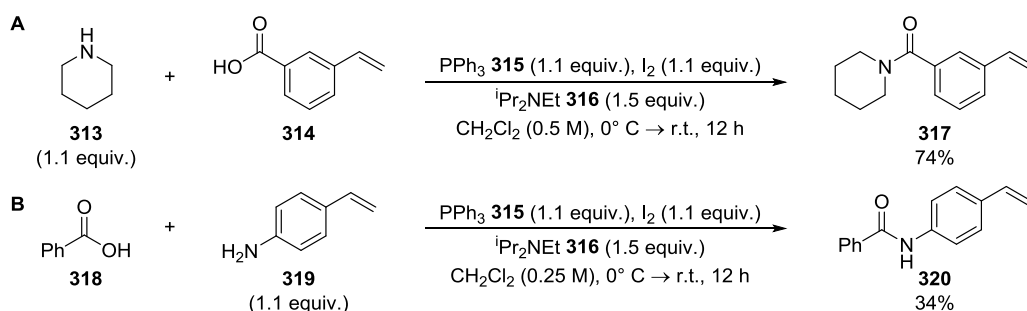
Scheme 2.12. Synthesis of ester and amide-functionalised styrene derivatives.
