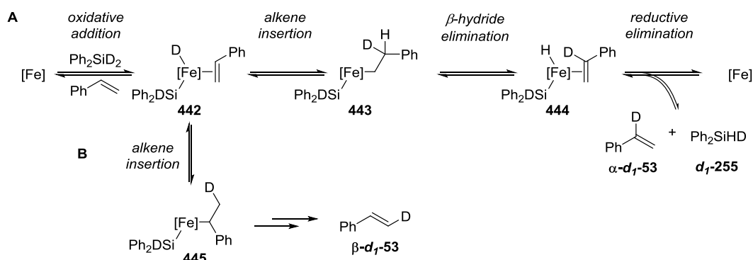
Scheme 2.36. Reversible \beta -hydride elimination mechanism to explain hydrogen-deuterium exchange in the hydrosilylation of styrene using deuterium-labelled silane.
