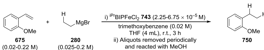
Scheme 4.28. Conditions used for initial rates approach for the hydromagnesiation of 2-methoxystyrene 675 using ethylmagnesium bromide 280 at different initial concentrations of each reagent.
