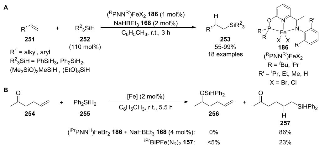
Scheme 2.07. Hydrosilylation of alkenes using a phosphinite-iminopyridine (PNN) iron complex as pre-catalyst. A General reaction scheme; B Comparison of chemoselectivity for alkene and ketone hydrosilylation using iron pre-catalysts 186 and 157 .
