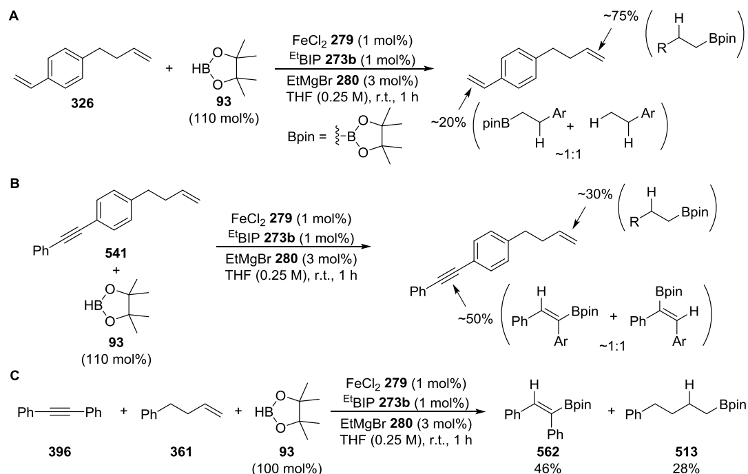
Scheme 3.13. Hydroboration of substrates containing multiple alkene/alkyne functionalities.
