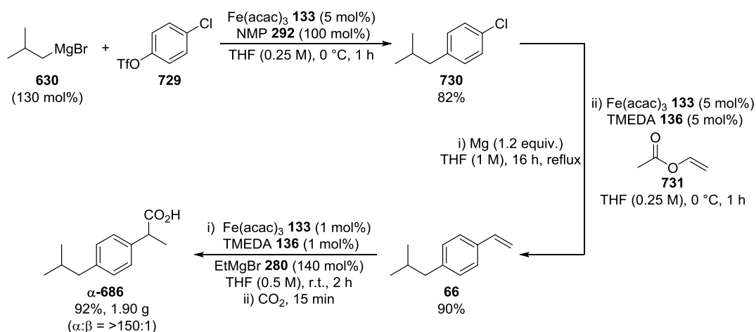
Scheme 4.18. Three-step synthesis of ibuprofen α-686 , using iron-catalysed reactions for each step. In collaboration with Adam Kolodziej and Fern Sinclair.
