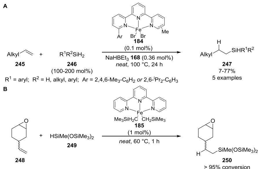
Scheme 2.06. Hydrosilylation of alkenes using iron(II) terpyridine complexes as pre-catalysts. A Using an iron(II) halide complex 184 reduced in situ using NaHBET_3 168 ; B Using an iron(II) dialkyl complex 185 .
