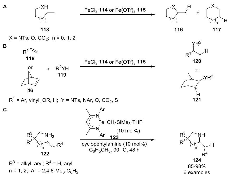
Scheme 1.19. High oxidation-state iron pre-catalysts used for the hydrofunctionalisation of alkenes.
