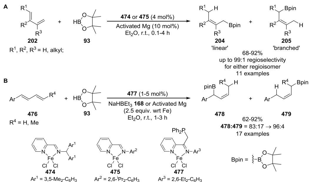
Scheme 3.01. 1,4-Hydroboration of 1,3-dienes using iron(II) iminopyridine pre-catalysts. A Regiodivergent hydroboration of aliphatic 1,3-dienes 202 using iron pre-catalysts 474 and 475 ; B Regioselective hydroboration of 1-aryl-1,3-dienes 476 using iron pre-catalyst 477 .
