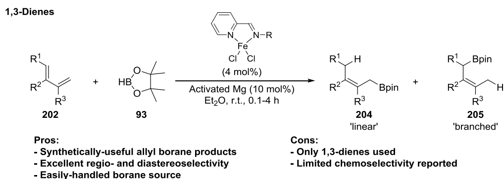
Scheme 3.08. State of the art iron-catalysed hydroboration in early 2012.
