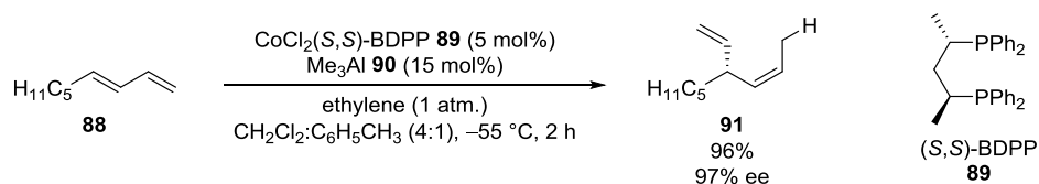
Scheme 1.15. Cobalt-catalysed asymmetric 1,4-hydrovinylation of 1,3-nonadiene 88 .
