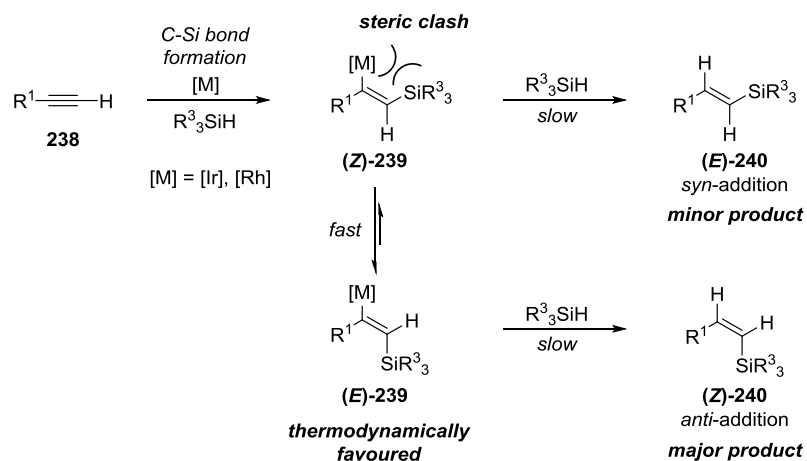
Scheme 2.04. Proposed mechanism to explain the stereochemical outcome of iridium- and rhodium-catalysed hydrosilylation of terminal alkynes.
