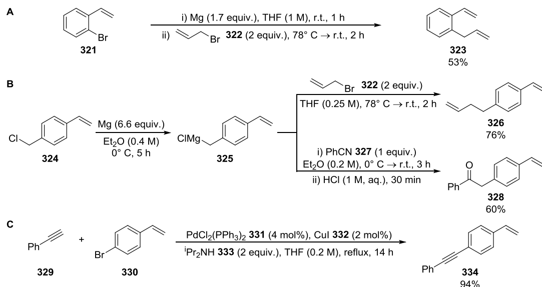
Scheme 2.13. Synthesis of allyl-, homoallyl-, keto- and alkynyl-substituted styrene derivatives by carbon-halogen bond functionalisation reactions.
