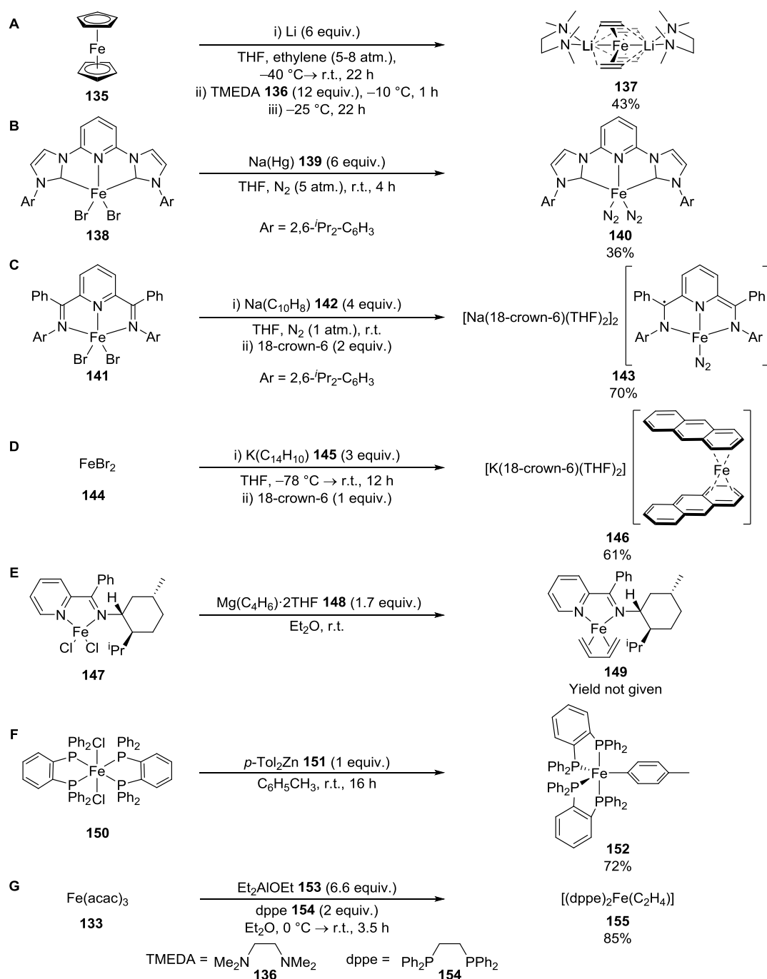
Scheme 1.21. The reduction of iron(II)/(III) species using inorganic and organometallic reductants.
