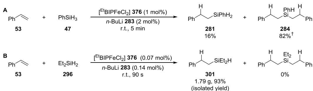
Scheme 2.21. Gram-scale hydrosilylation of styrene 53 under ‘solvent-free’ conditions. † Yield based on phenylsilane 47 .
