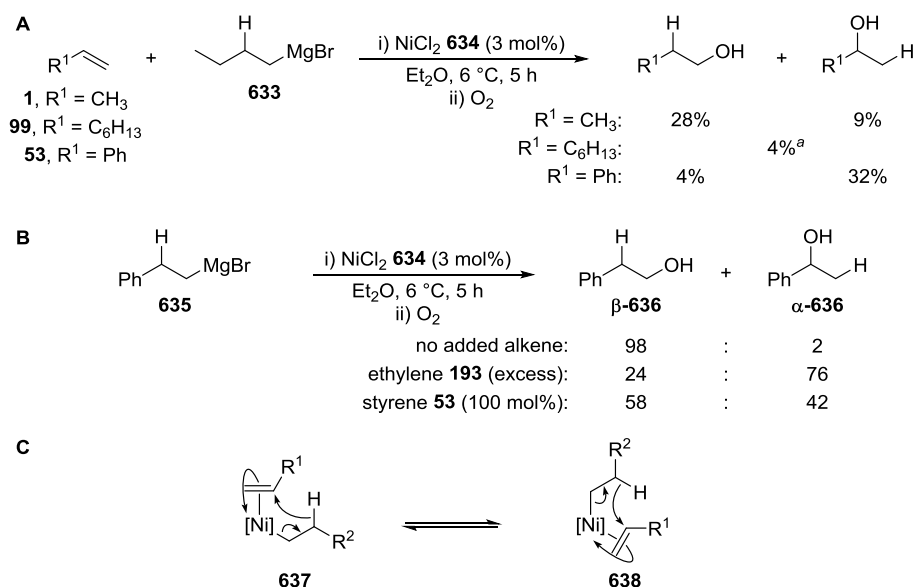
Scheme 4.09. Nickel-catalysed hydromagnesiation. A Hydromagnesiation of terminal alkenes using n -butylmagnesium bromide 633 . B Isomerisation of (2-phenylethyl)magnesium bromide 635 using nickel chloride 634 in the absence and presence of alkenes. C Proposed direct \beta -hydride transfer between alkyl and alkene ligands on nickel. a Regioselectivity not reported.
