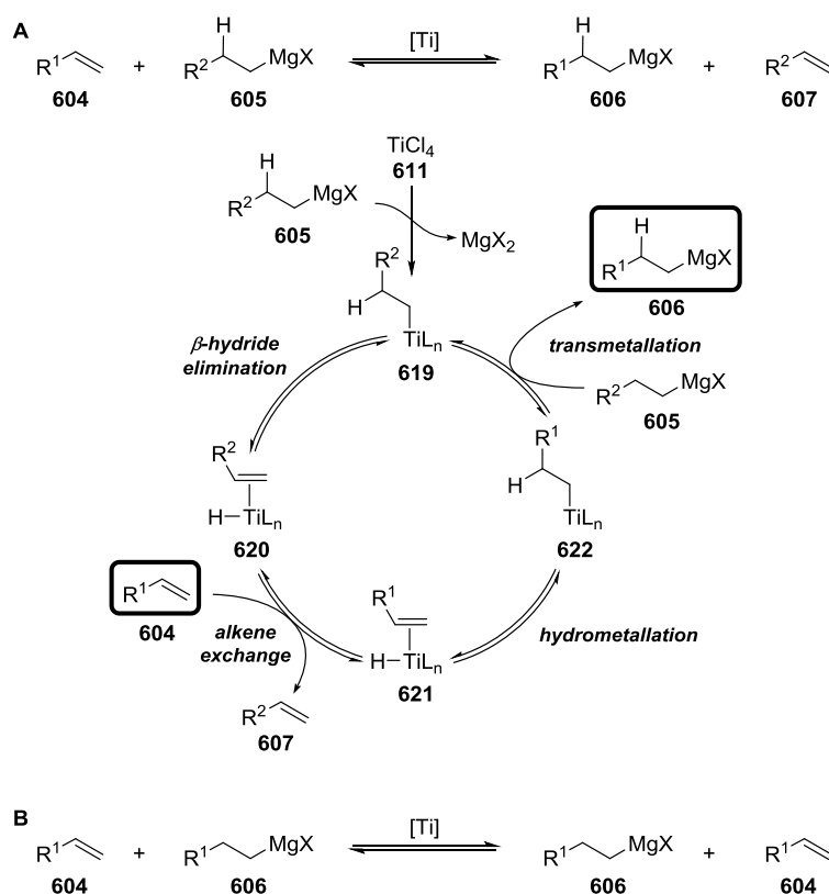
Scheme 4.06. A Proposed mechanism for titanium-catalysed hydromagnesiation of alkenes 604 using alkyl Grignard reagents bearing \beta -hydrogen atoms 605 . B ‘Unproductive’ hydromagnesiation reaction between an alkene 604 and a Grignard reagent bearing \beta -hydrogen atoms 606 .
