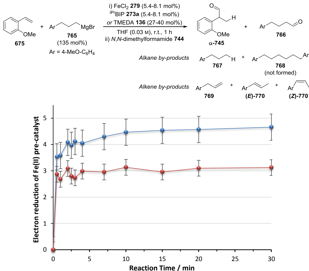
Figure 4.17. Quantification of the reduction of iron(II) pre-catalysts using alkyl Grignard reagent 765 ● = i PrBIPFeCl 2 734 ; ● = FeCl 2 279 + TMEDA 136 (5 equiv. w.r.t. Fe)
