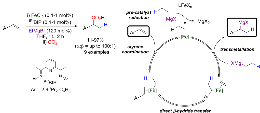
Scheme A2. Iron-catalysed hydromagnesiation of styrene derivatives
