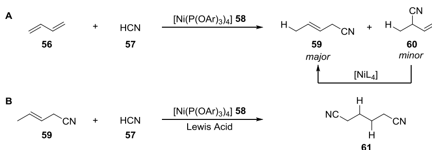
Scheme 1.11. Nickel-catalysed hydrocyanation of 1,3-butadiene 56 to give adiponitrile 61 .
