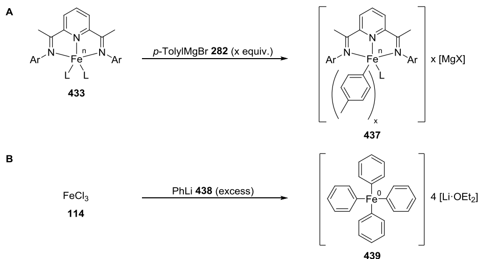
Scheme 2.33. Exhaustive arylation of iron species by aryl-metal reagents. A Proposed deactivation of iron (pre-)catalyst in the presence of excess p -tolylmagnesium bromide 282 . B Reported reaction of iron(III) chloride 114 with phenyllithium 438 to give iron(0) tetraphenylferrate 439 . [123]
