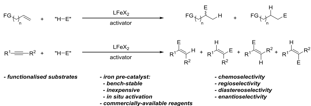
Scheme 1.29. Project Aims: Development of operationally-simple iron-catalysed hydrofunctionalisation methodologies using commercially-available reagents.
