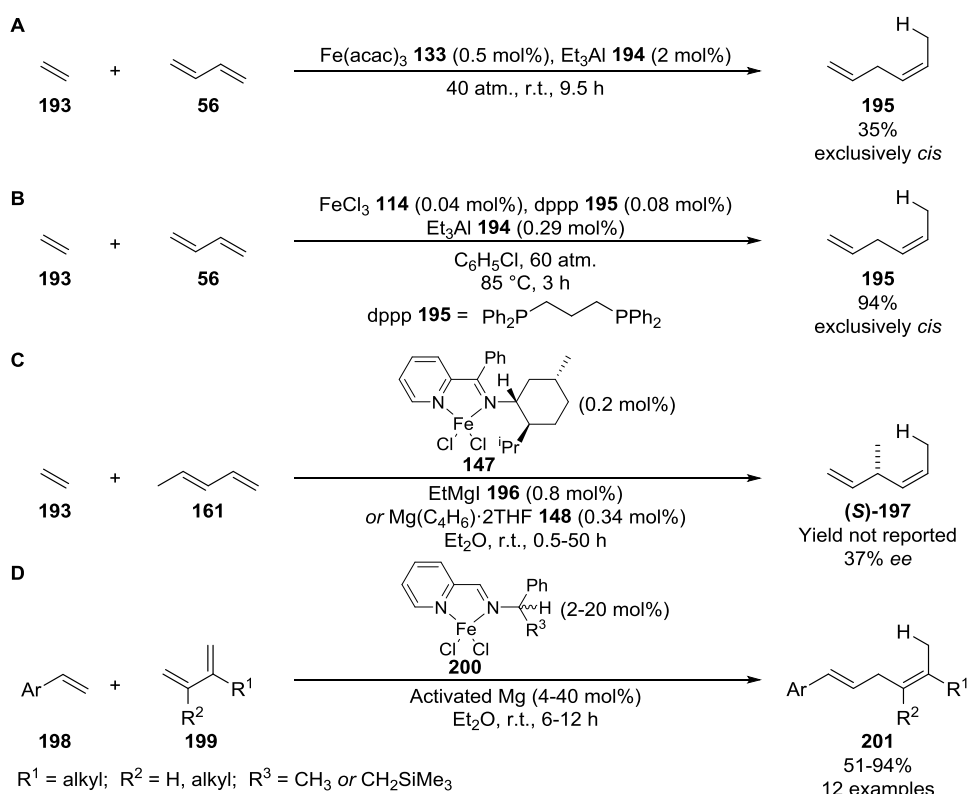
Scheme 1.26. Iron-catalysed 1,4-hydrovinylation of 1,3-dienes. A 1,4-hydrovinylation of 1,3-butadiene 56 with ethylene 193 using an iron pre-catalyst reduced in situ with triethylaluminium 194 ; B Improvement in activity using a bidentate phosphine ligand 195 ; C Enantioselective 1,4-hydrovinylation of 1,3-pentadiene 161 with ethylene 193 using an iminopyridine iron complex 147 reduced in situ with organomagnesium reagents; D Expansion of substrate scope for iron-catalysed 1,4-hydrovinylation of 1,3-dienes.
