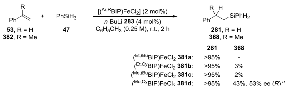
Scheme 2.20. Hydrosilylation of styrene 53 and \alpha -methylstyrene 382 using enantiopure bis(imino)pyridine iron(II) pre-catalysts 381a-d . a Determined by chiral HPLC following conversion to 2-phenylpropanol 383 .
