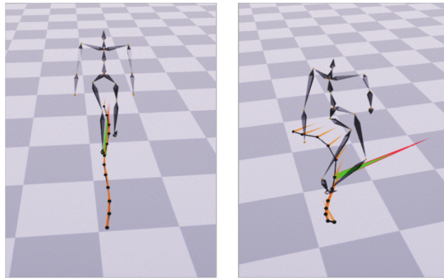
Figure 3.4: Overfitting. When only a small amount of training data is available it is easy to overfit, here a character walks reasonably in a straight line but creates unrealistic poses when following turning trajectories unseen in the training data. To create this visualisation a PFNN was trained on neutral locomotion data and fine-tuned with limited stylised ( bent forward ) data.
