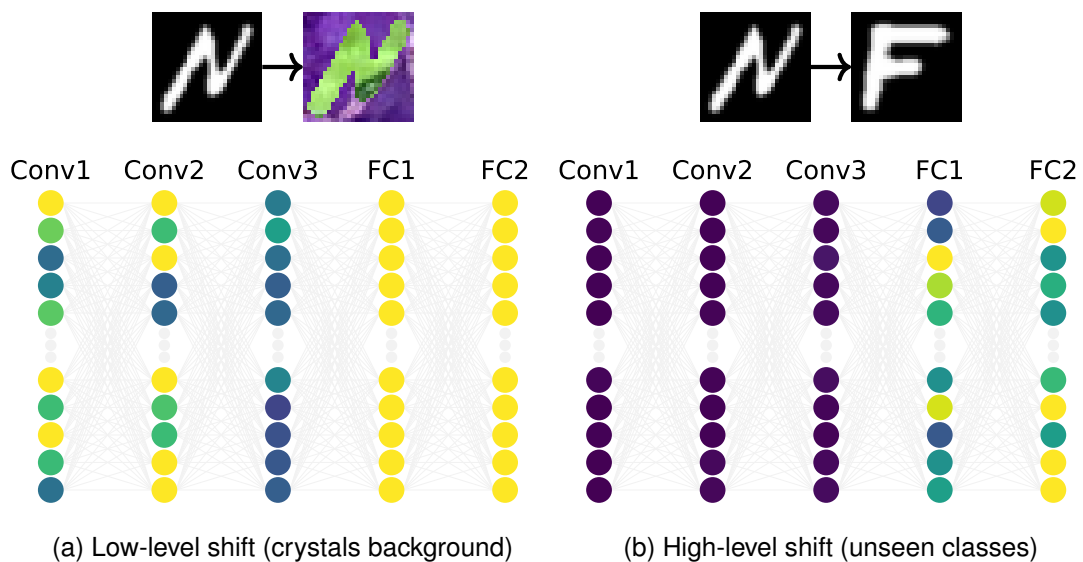
Figure 5.3: Patterns of surprise for different changes in data distribution. Yellow units are highly surprised and dark blue units are unsurprised. (a) For low-level shifts surprise is noticed in the early layers and this effect propagates through the rest of the network. (b) For high-level shifts early layers are unsurprised (similar features) whereas the later fully connected layers show surprise.
