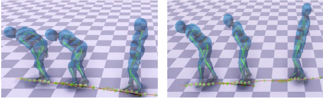
Figure 3.16: Interpolation. Style: Bent Forward to Lean Back . Left: LPN One-hot. Right: LPN FiLM. The one-hot method does not create a smoothly changing transition.
