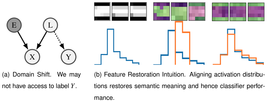
Figure 4.1: The feature restoration approach to resolving domain shift. (a) Data generating assumptions for source-free domain adaptation. (b) Aligning unit activation distributions to restore semantic meaning to features.
