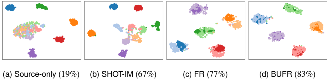
Figure 4.10: t-SNE (Van der Maaten and Hinton, 2008) applied to the feature representations of 5 classes from the EMNIST-DA crystals shift. Dark colours show the source data, light the target. Model accuracies are shown in parentheses.
