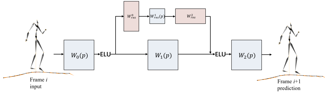
Figure 3.5: System Overview. Style agnostic parameters, shared across all styles, are learned in the animation synthesis PFNN network (bottom row). Style specific parameters are learned in a CP decomposed residual adapter (top row) which can change capacity as the size of the central matrix changes. Phase-functioned weight matrices are shown in blue, non phase-functioned weight matrices are shown in red. We use the exponential linear unit (ELU) as our non-linearity Clevert et al. (2015).
