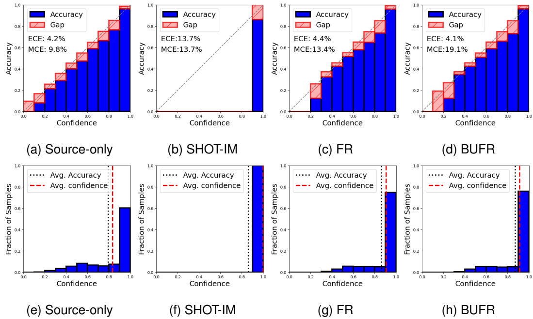
Figure 4.8: Reliability diagrams and confidence histograms for a mild EMNIST-DA shift (shot noise). (a-d): Reliability diagrams. (e-h): Corresponding confidence histograms. Examining the rightmost bin show that when FR and BUFR are confident (c & g, d & h), predictions are more accurate than for SHOT-IM (b & f).
