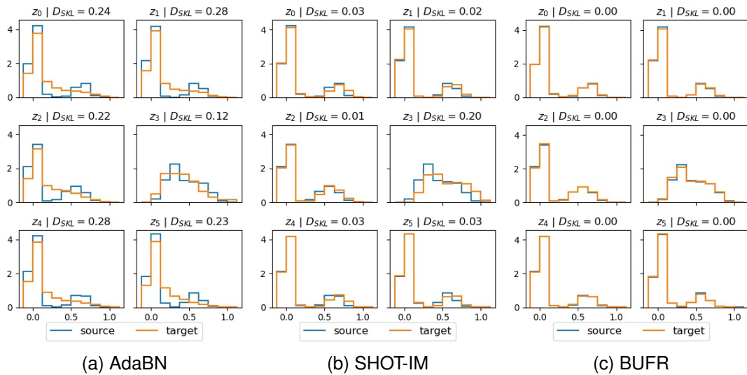
Figure B.7: Histograms showing distribution alignment on the CIFAR-10-C impulse-noise shift. The blue curves are the saved marginal distributions under the source data (identity). The orange curves are the marginal distributions under the target data (impulse-noise) after adaptation . (a) AdaBN only slightly aligns the marginal distributions. (b) SHOT-IM partially aligns the marginal distributions despite not optimising for alignment. (c) BUFR matches the activation distributions very closely.
