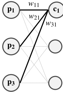
Figure 5.4: Update rule schematic. The thick weight connections update only if the aggregated parent surprise, \bar{p}_1 , is low enough and the child surprise, c_1 , is high enough.
