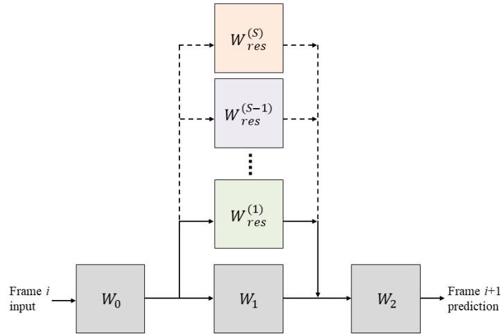
Figure 3.3: Style Modelling with Residual Adaptation. PFNN weights, shared across styles, are shown in grey. Style specific, phase-functioned, residual adapter weights are shown in other colours. Weights ( W_0 , W_1 , W_2 , W_{res}^{(s)} ) are calculated for a given phase value using Equation 3.1. Phase omitted from figure for brevity.
