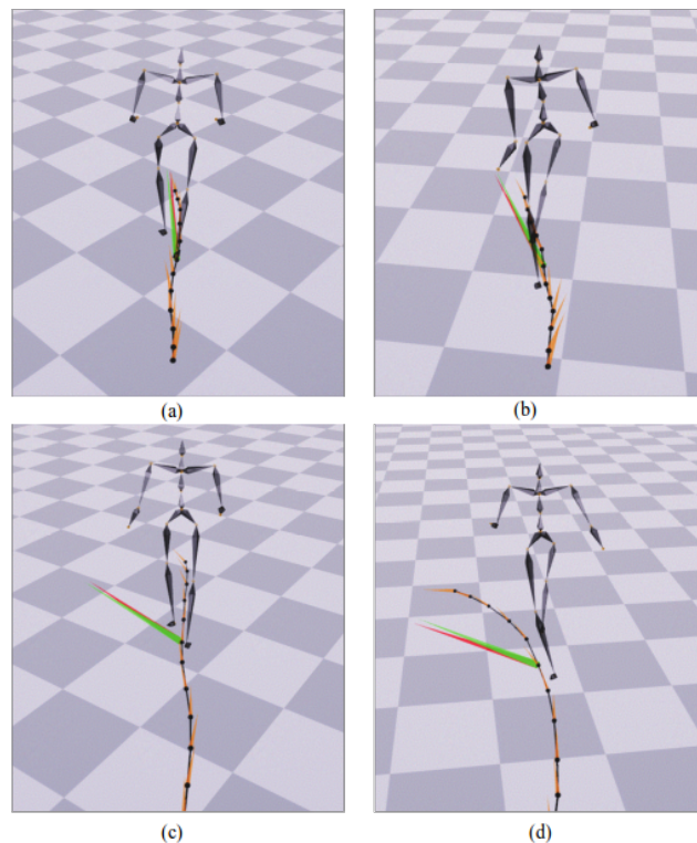
Figure 3.7: Underfitting and overfitting to different styles as residual adapter capacity changes. (a) Dinosaur style, CP decomposed residual adapter, reasonably capturing the style. (b) Dinosaur style, diagonal residual adapter, the style is captured poorly due to underfitting. (c) Elated style, full residual adapter, the style is well modelled but the character struggles to turn left. (d) Elated style, CP decomposed residual adapter, the style is still well modelled but the character can turn more easily.
