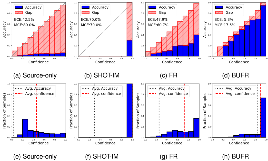
Figure 4.7: Reliability diagrams and confidence histograms for a severe EMNIST-DA shift (sky). (a-d): Reliability diagrams. (e-h): Corresponding confidence histograms. (a & e): The source model on the target data achieves poor accuracy but generally predicts with low confidence. (b & f): SHOT-IM confidently makes incorrect predictions. (d & h): Our BUFR method is more well calibrated.
