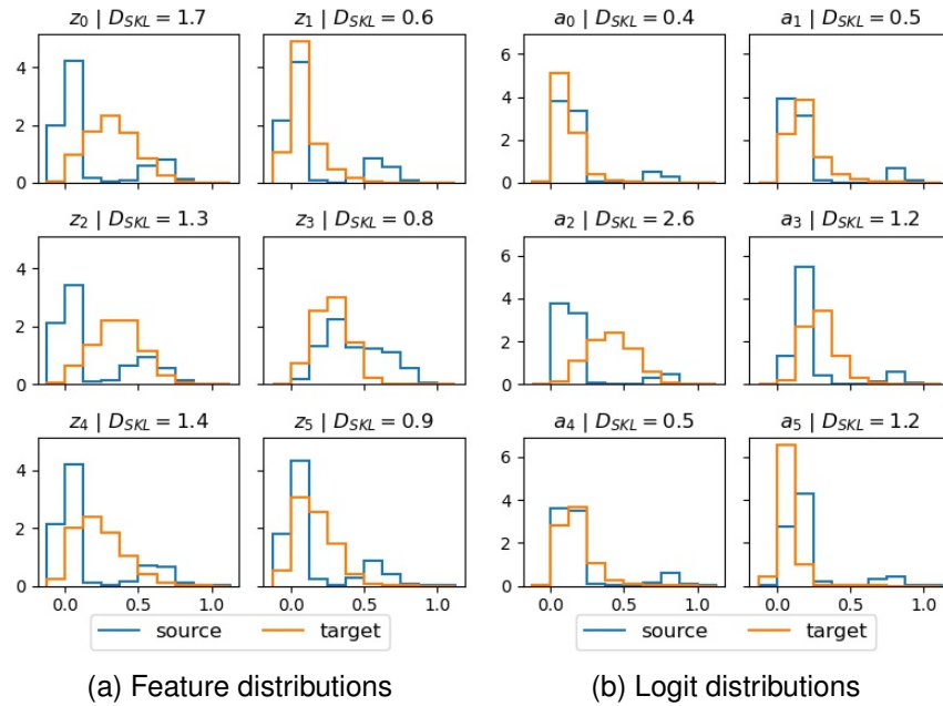
Figure B.6: Histograms of 6 marginal distributions using the CIFAR-10-C impulse-noise shift. The blue curves are the saved marginal distributions under the source data (identity). The orange curves are the marginal distributions under the target data (impulse-noise) before adaptation . (a) Marginal feature activation distributions. (b) Marginal logit activation distributions. D_{SKL} is the symmetric KL divergence.
