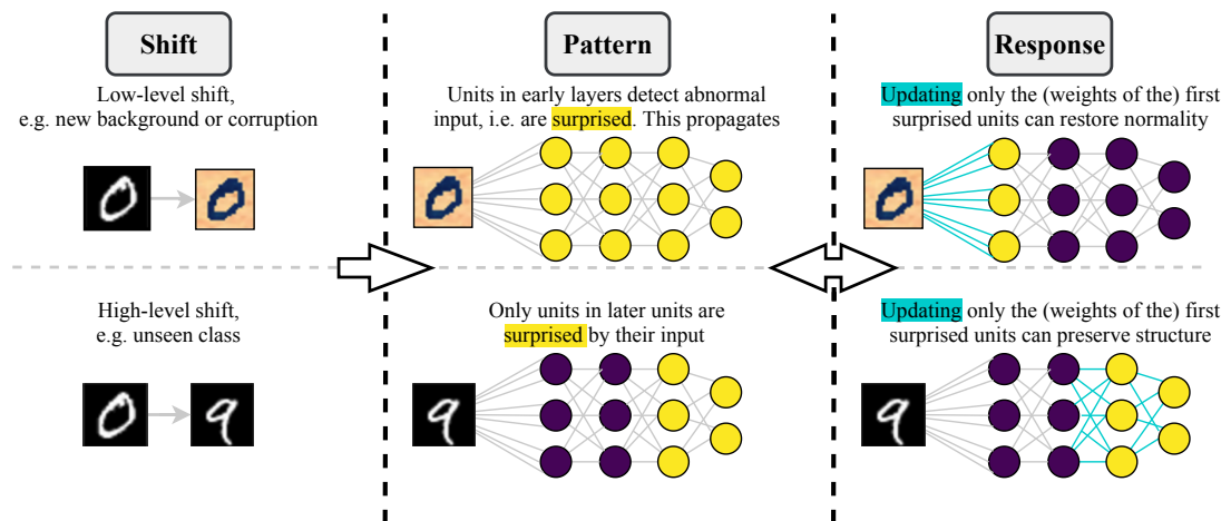
Figure 5.1: Patterns of unit-level surprise can be used to choose which few parameters to update based on a shift in data distribution. The update response may change the pattern which may in turn change the parameters to be updated by the response. Purple units are unsurprised, yellow units surprised, blue indicates the weights to update.
