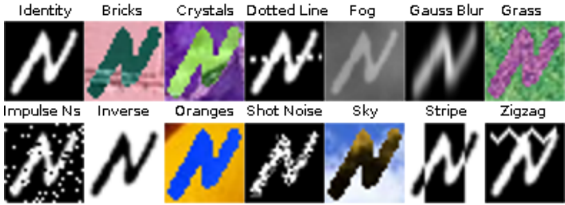
Figure 4.3: EMNIST-DA shifts.
