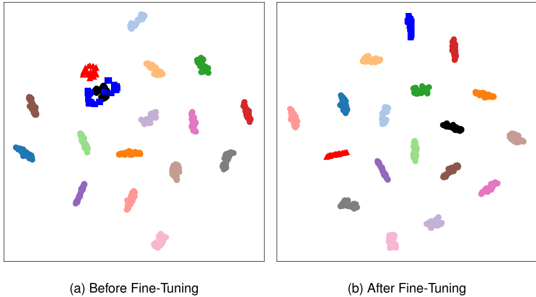
Figure 3.11: t-SNE for FiLM parameters. We show embedding for 50 different stylised motion clips for 15 style that the FiLM generator is pretrained on (pastel colours). We also show 50 embeddings for 3 styles unseen during pretraining (black circles, blue squares, red triangles). (a) Before fine-tuning the style the FiLM generator is trained on are well separated but the unseen styles are not. (b) After fine-tuning all styles are well separated.
