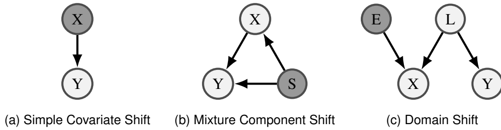
Figure 2.1: Different data generating processes lead to different types of dataset shift as described in Storkey (2009). Darker circles highlight the variables that change under the dataset shift in question.
