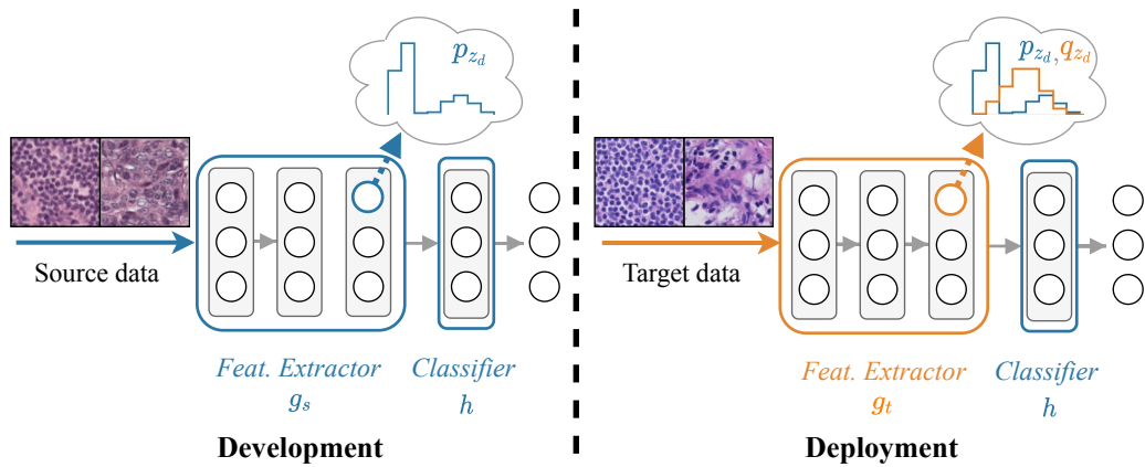
Figure 4.4: Feature Restoration Overview. Left : At development time, approximate marginal feature distributions, \{p_{z_d}\}_{i=1}^D , are saved using the source data. Right : At deployment time, the approximations of the marginal feature distributions under the target data, \{q_{z_d}\}_{i=1}^D , are aligned with those under the source data.
