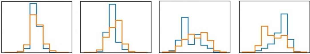
Figure 5.2: Examples of our histogram parameterisations of P(A) , in blue, and Q(A) , in orange. When new data is received, the activation distribution changes, the more different the distributions the higher the surprise. From left to right, the surprise values s(A) are approximately 0.1, 0.2, 0.3, 0.4.
