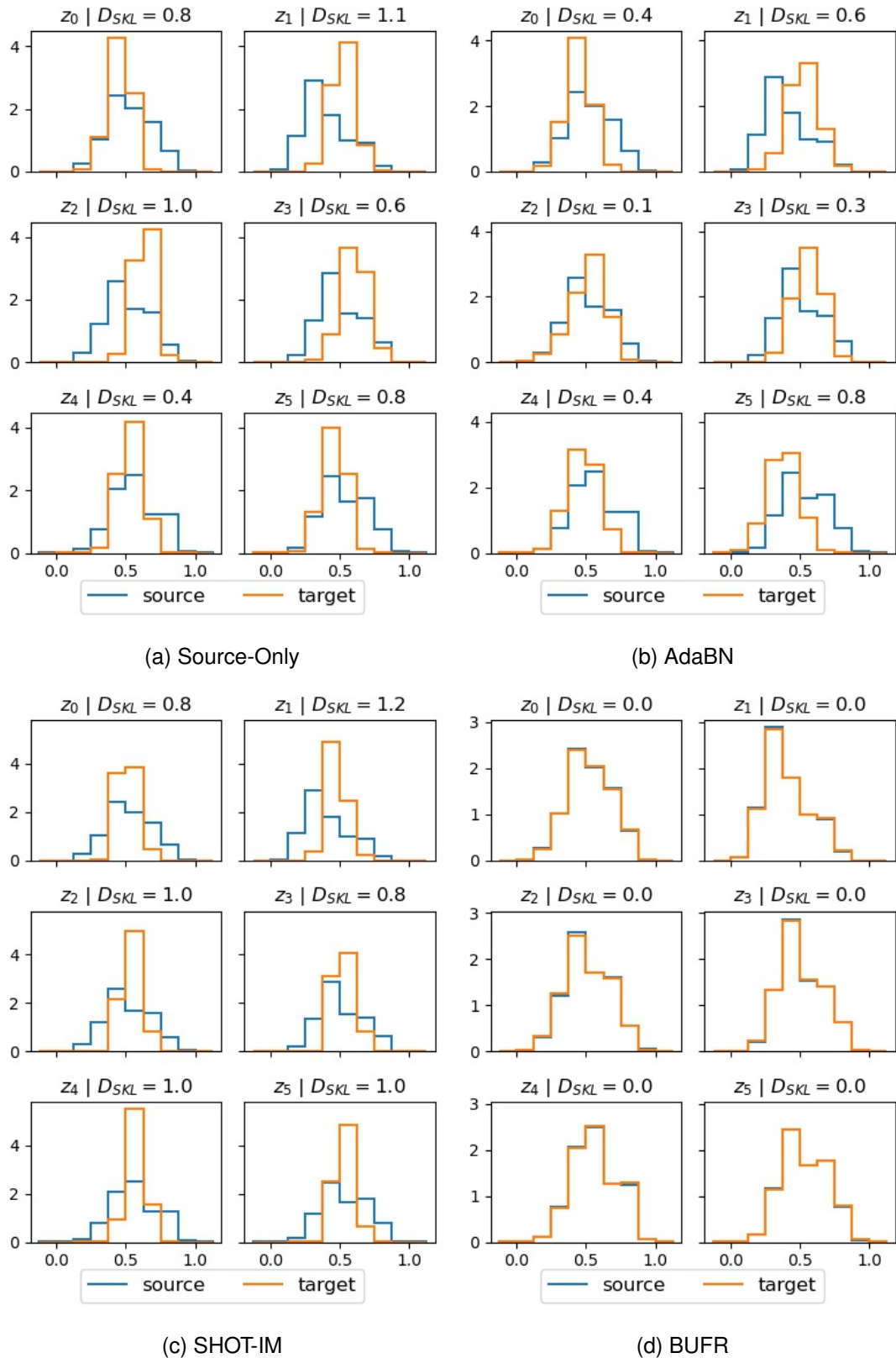
Figure 4.5: Histograms showing distribution alignment on the EMNIST-DA stripe shift. The blue curves are the saved marginal distributions under the source data (identity). The orange curves are the marginal distributions under the target data (stripe). (a): Source-Only, before adaptation distributions are different. (b,c): AdaBN and SHOT-IM, after adapting the marginal distributions are not aligned despite achieving reasonable accuracy. (d) BUFR, after adaptation the activation distributions align very closely, making D_{SKL} very small.
