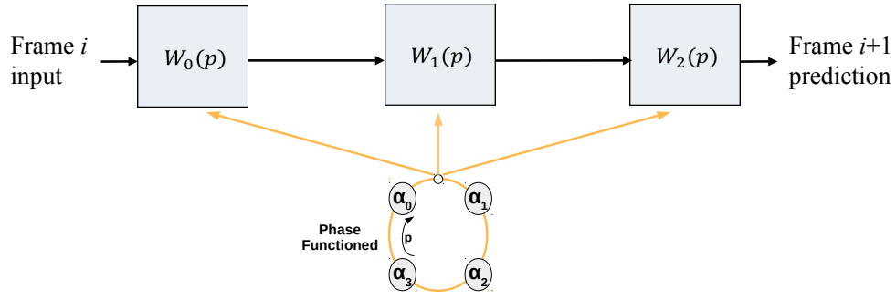
Figure 3.2: A Phase-Functioned Neural Network. The weights used for prediction depend on a phase label and are set by blending parameters using Equation 3.1.
