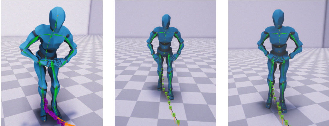
Figure 3.13: No Global Phase. Style: Pendulum Hands . Left to Right: Data, PFNN FiLM, LPN FiLM. The hands do not swing as they should using the PFNN.
