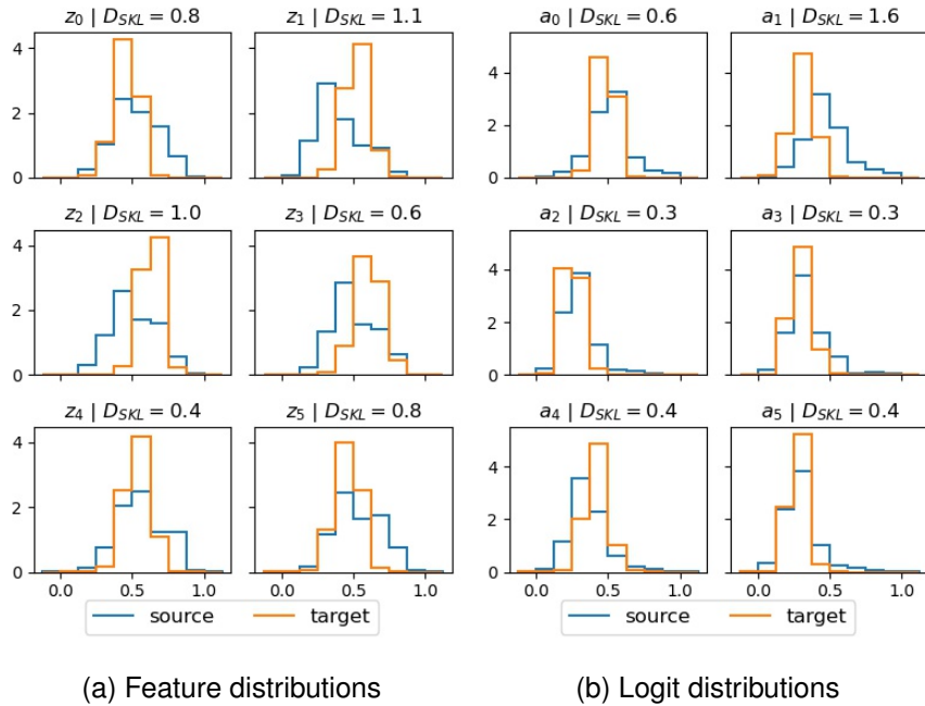
Figure B.5: Histograms of 6 marginal distributions using the EMNIST-DA stripe shift. The blue curves are the saved marginal distributions under the source data (identity). The orange curves are the marginal distributions under the target data (stripe) before adaptation . (a) Marginal feature activation distributions. (b) Marginal logit activation distributions. D_{SKL} is the symmetric KL divergence.
