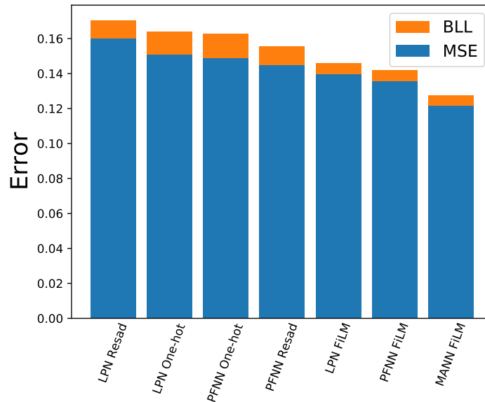
Figure 3.18: Test Error. We compare the error of different models on a held out test set. Each bar is divided into the blue mean squared error (MSE) and the orange bone length loss (BLL).
