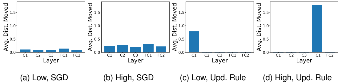
Figure 5.5: Mean Euclidean distances moved by units in each layer. (a) using SGD for a low level shift (crystals background shift), (b) using SGD for a high level shift (H1, 5 unseen classes), (c) our update rule for the same low level shift and (d) our update rule for the same high level shift.
