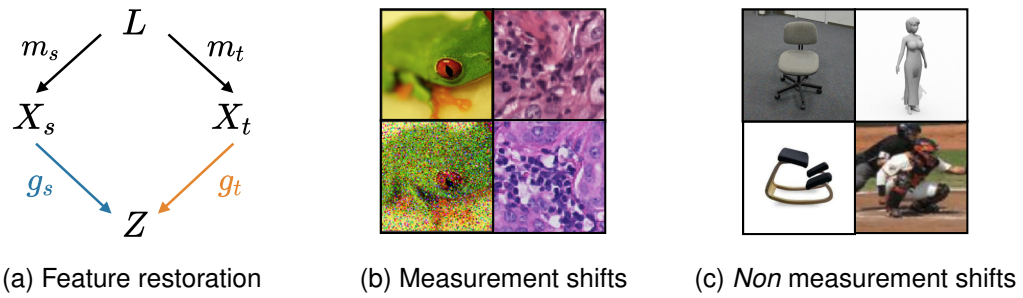
Figure 4.2: Feature restoration diagram and measurement shift examples. (b,c): top=source, bottom=target. (b): CIFAR-10-C ‘frog’ & CAMELYON17 ‘tumor’. (c): OFFICE-31 ‘desk chair’ & VISDA-C ‘person’.
