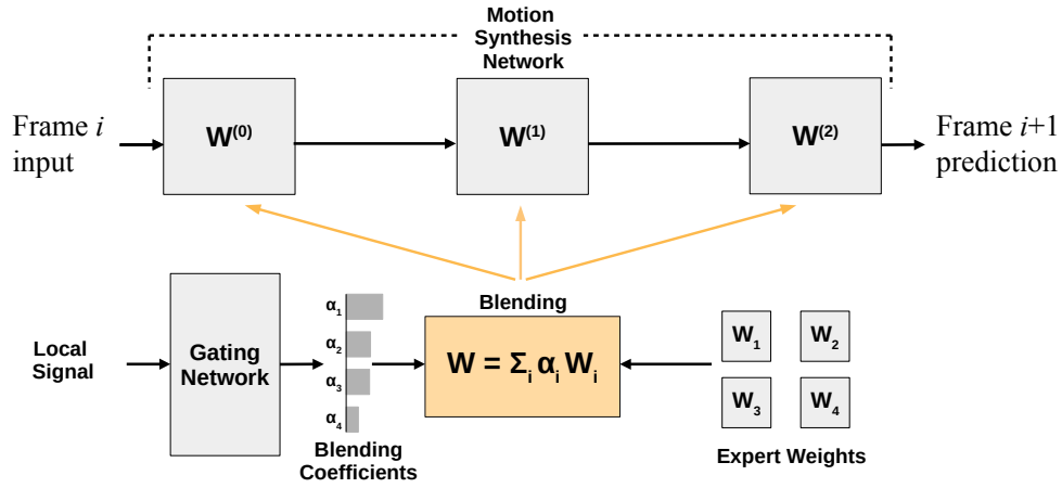
Figure 3.9: A Gated Experts System. As with the PFNN, weights used for prediction are set by blending parameters. Rather than being manually defined, the blending is learned dependent on some local signal.
