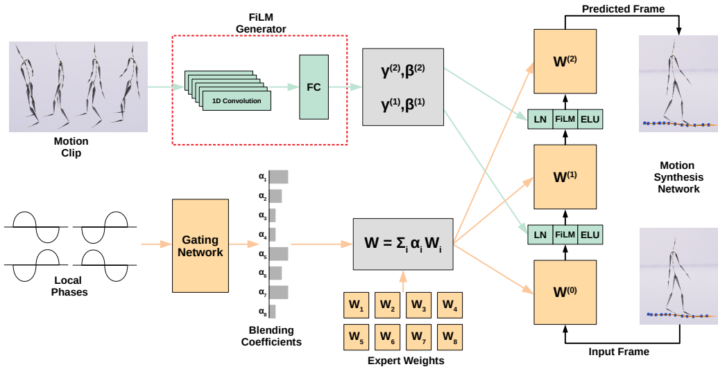
Figure 3.12: 100STYLE Style Modelling System. Animation synthesis (peach) is performed using a local phase network that uses a gating network to blend expert weights to create the parameters of a motion synthesis network. Style modulation (green) is done using FiLM parameters which modulate the hidden units of the motion synthesis network. LN is layer normalisation (Ba et al., 2016).
