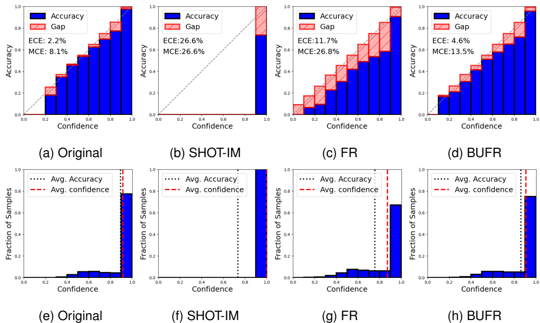
Figure 4.6: Reliability diagrams and confidence histograms over all EMNIST-DA corruptions. (a-d): Reliability diagrams. (e-h): Corresponding confidence histograms. (a & e): The ‘Original’ source model is well-calibrated on the source data . (b & f): Minimising prediction entropy leads to overconfidence. (c & g, d & h): Our methods, FR and BUFR, which do not make use of entropy minimisation, are more well calibrated.
