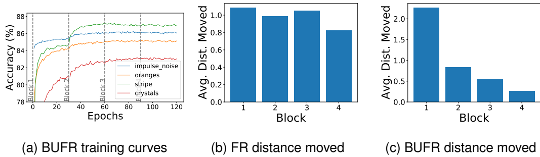
Figure 4.9: Bottom-Up Training Analysis. (a) BUFR accuracy during training on selected EMNIST-DA corruptions. Dashed-grey lines indicate when the next block is unfrozen. (b, c) Average Euclidean distance moved by parameters in each block when adapting g_s to g_t using the same constant learning rate. (b) FR moves all parameters a similar amount. (c) BUFR changes primarily the early layers.
