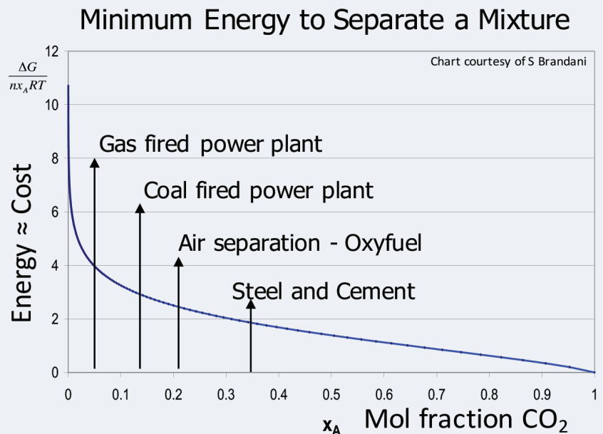
Figure 8: Having a range of different technology developments is important to address varied industry requirements. For example, not all capture is the same, and this chart shows that more energy is needed for capture from more dilute CO 2 emissions. It also illustrates that CO 2 capture from steel and cement production is cheaper than from gas power plant. Source: Stefano Brandani
