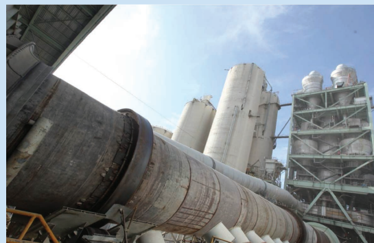
One third of CO 2 emissions from a cement plant derive from fuel combustion and two thirds from the calcination process itself. Photo: LafargeHolcim 2015
