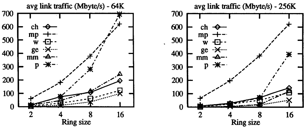
Figure 4.10: Traffic per link, for cache sizes of 64KK (left) and 256Kbytes (right). ‘ch’ stands for chol() , ‘mp’ for mp3d() , ‘w’ for water() , ‘ge’ for ge() , ‘mm’ for mmult() , ‘p’ for paths() .
