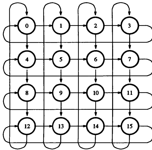
Figure 6.1: A four-by-four SCI mesh.
