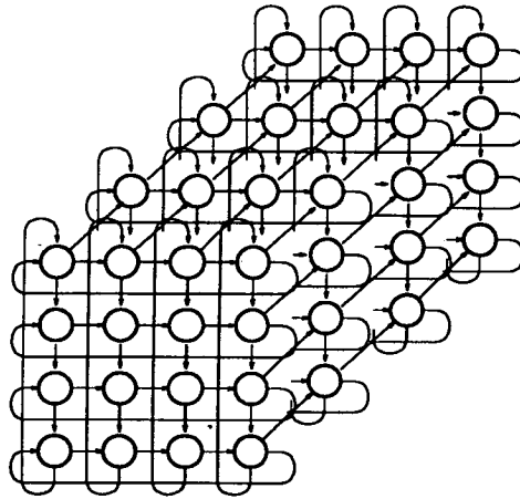
Figure 6.12: A four-by-four-by-four SCI cube. Wrap-around connections in the Z dimension not shown.
