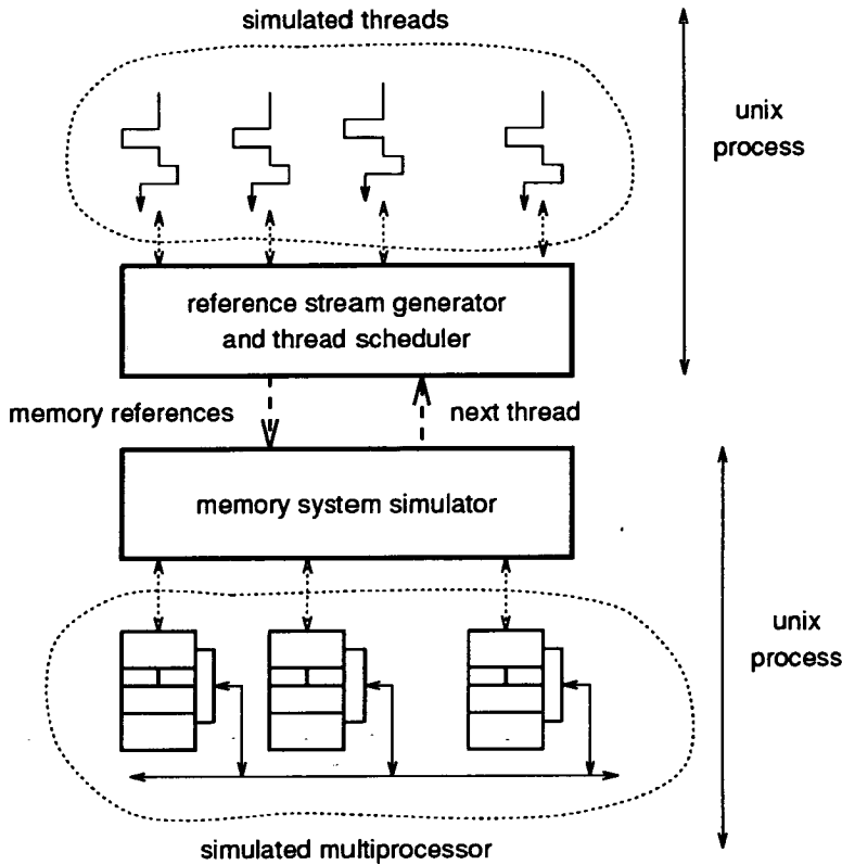
Figure 3.1: Simulation environment.
