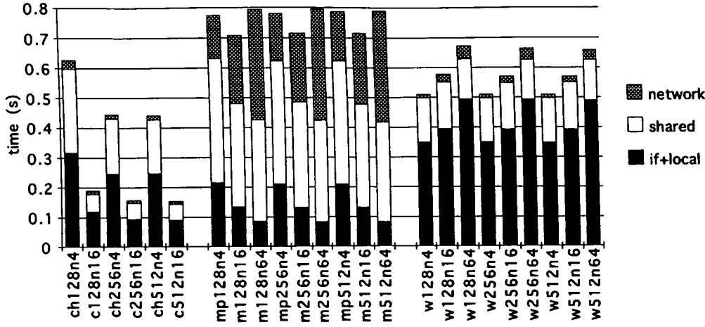
Figure 6.3: Execution time plots for chol() (left), mp3d() and water() (right). The segments show the time spent on shared-data references and network latency. Data sets are scaled up with machine size.
