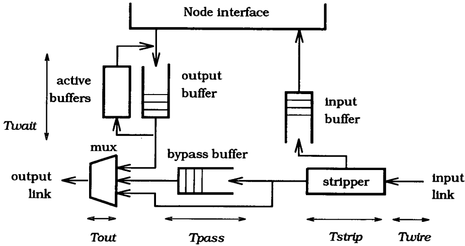
Figure 2.2: SCI link interface.
