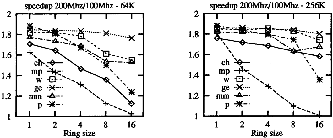
Figure 4.6: Speedup achieved by doubling processor clock frequency, with cache sizes of 64K (left) and 256Kbytes (right). ‘ch’ stands for chol() , ‘mp’ for mp3d() , ‘w’ for water() , ‘ge’ for ge() , ‘mm’ for mmult() , ‘p’ for paths() .
