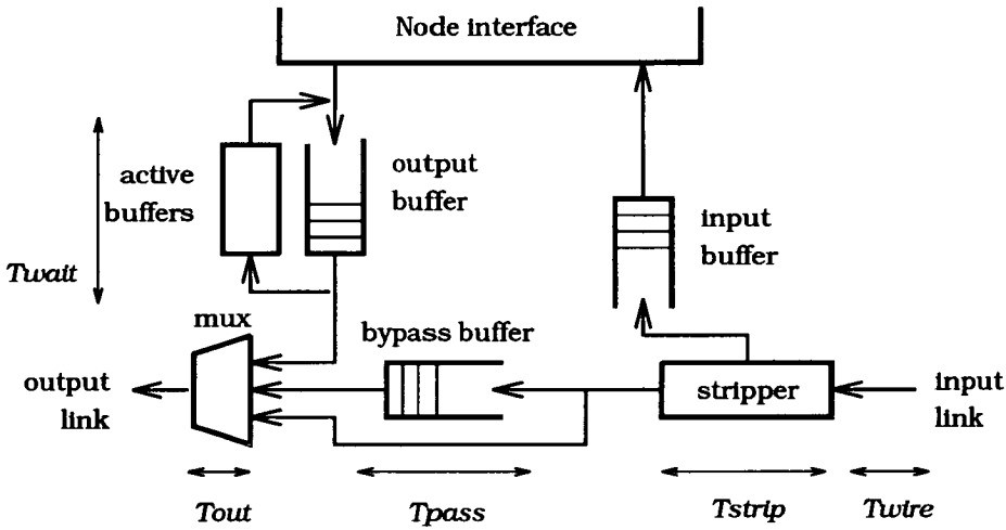
Figure 3.3: SCI link interface.
