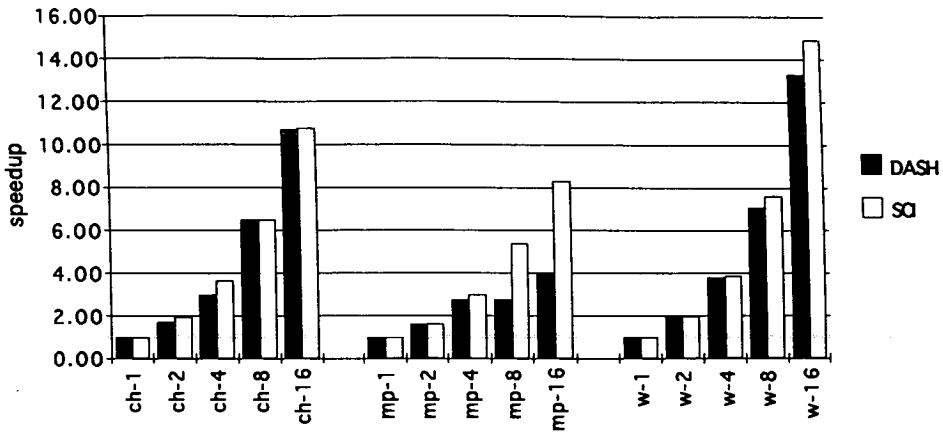
Figure 4.13: Speedup plots for chol() (left), mp3d() (mid) and water() (right).
