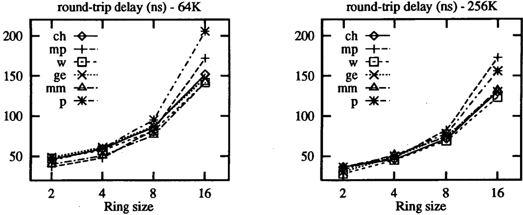
Figure 4.8: Average round-trip delay, with cache sizes of 64K (left) and 256Kbytes (right). ‘ch’ stands for chol() , ‘mp’ for mp3d() , ‘w’ for water() , ‘ge’ for ge() , ‘mm’ for mmult() , ‘p’ for paths() .
