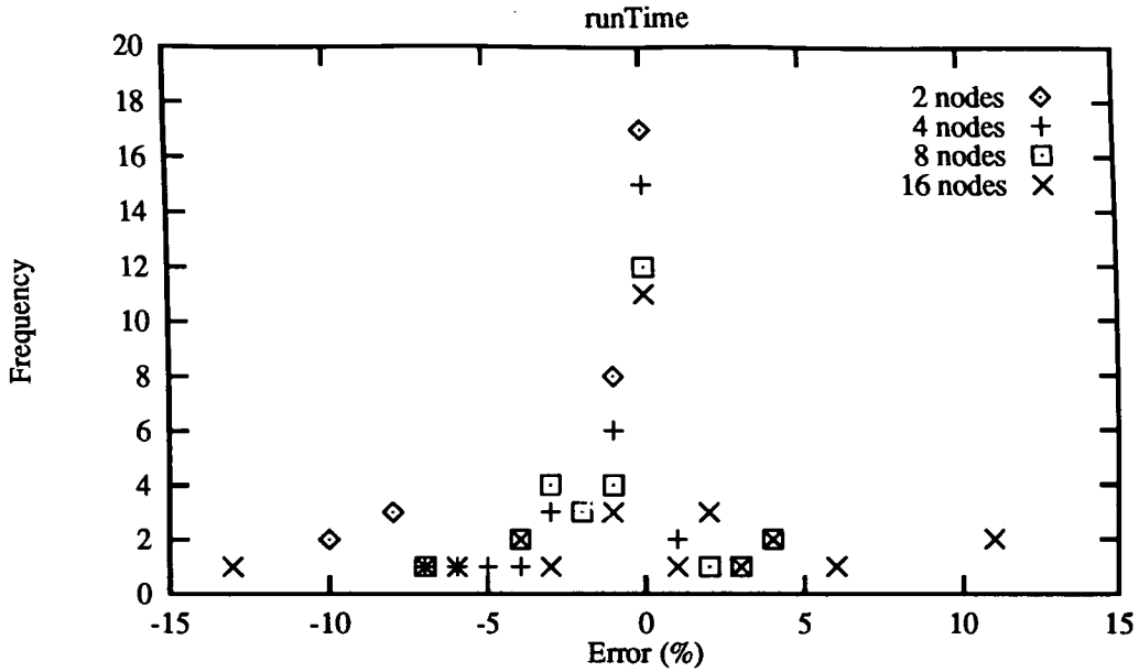
Figure 5.1: Distribution of error in the model predictions when compared to the simulation result. A negative error means that the model underestimates the execution time.
