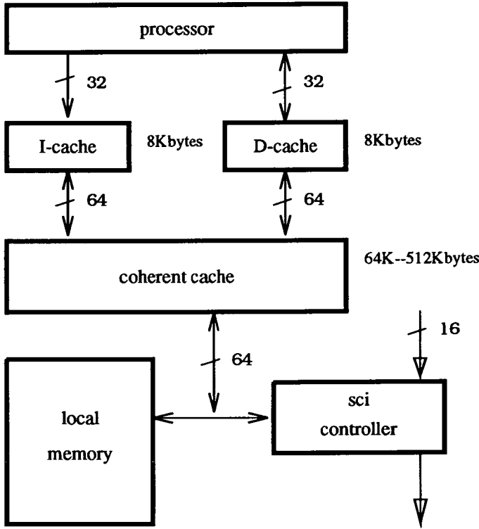
Figure 3.2: Architecture of the processing nodes.
