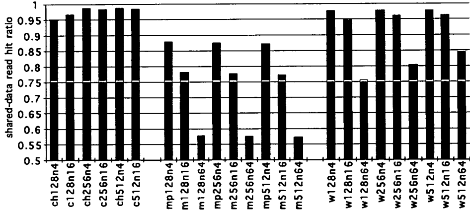
Figure 6.4: Coherent cache shared-data read hit ratio plots for chol() (left), mp3d() (center) and water() (right).
