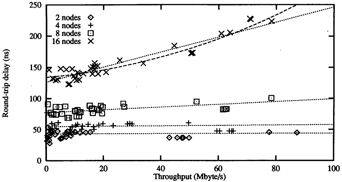
Figure 4.9: Latency versus throughput on 2-, 4-, 8- and 16-node rings.
