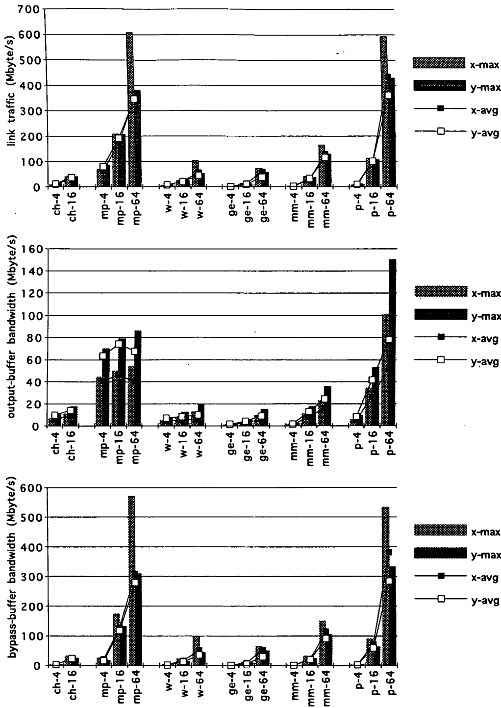
Figure 6.11: Link traffic per dimension (top), output buffer traffic per dimension (mid) and bypass buffer traffic per dimension (bottom), for 256Kbytes caches. From left to right: chol(), mp3d(), water(), ge(), mmult() and paths().
