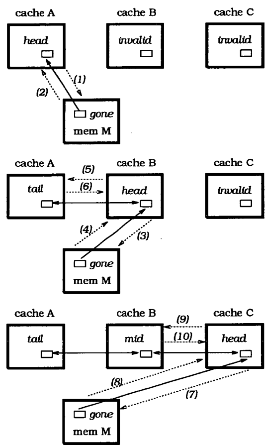
Figure 2.3: Sharing-list setup. Solid lines represent sharing-list links, dotted lines represent messages.
