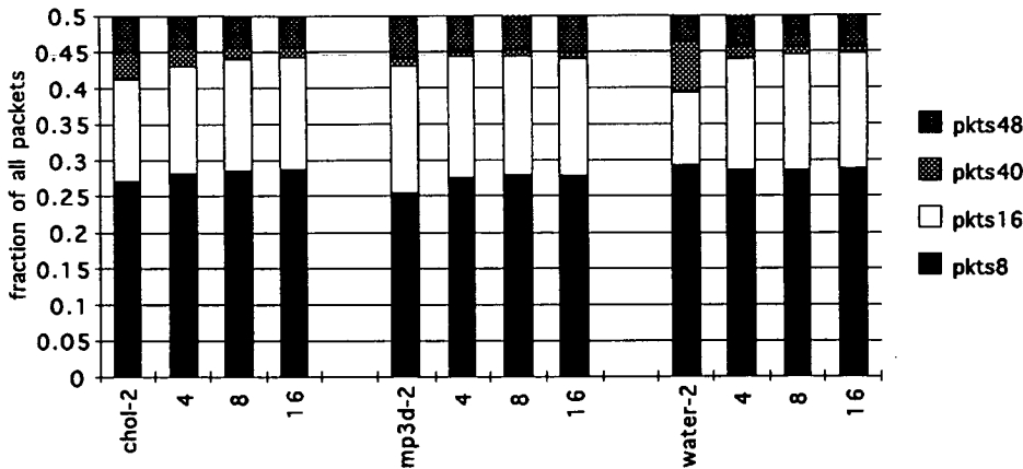
Figure 4.11: Distribution of packet sizes for 256Kbytes caches.
