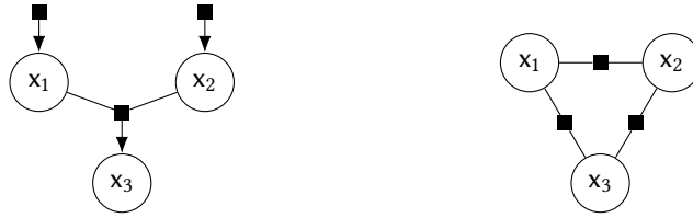
(a) Example directed factor graph. (b) Example undirected factor graph.
