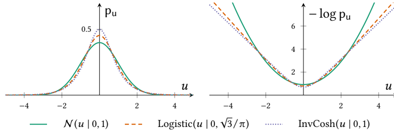
Figure D.1: Unit variance densities with unbounded support.
