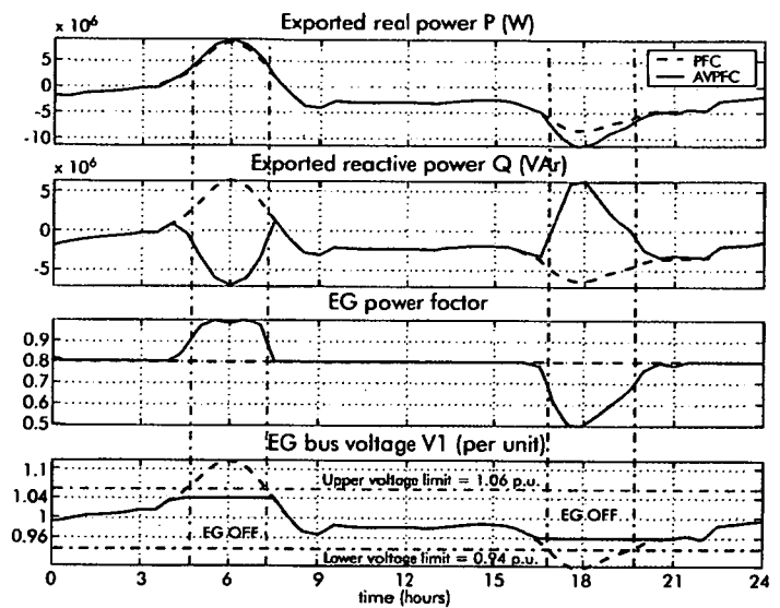
Figure 6: DG operation with power factor control and hybrid voltage/power factor control
