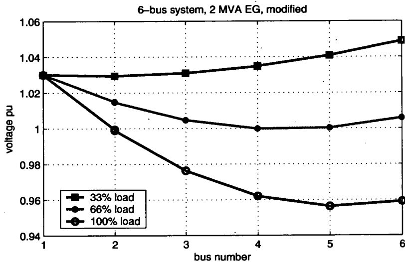
Figure 2.13: Voltage profile of the six-bus system of Figure 2.1 modified to accommodate 2 MVA of embedded generation on bus 6 (transformer 1:1)
