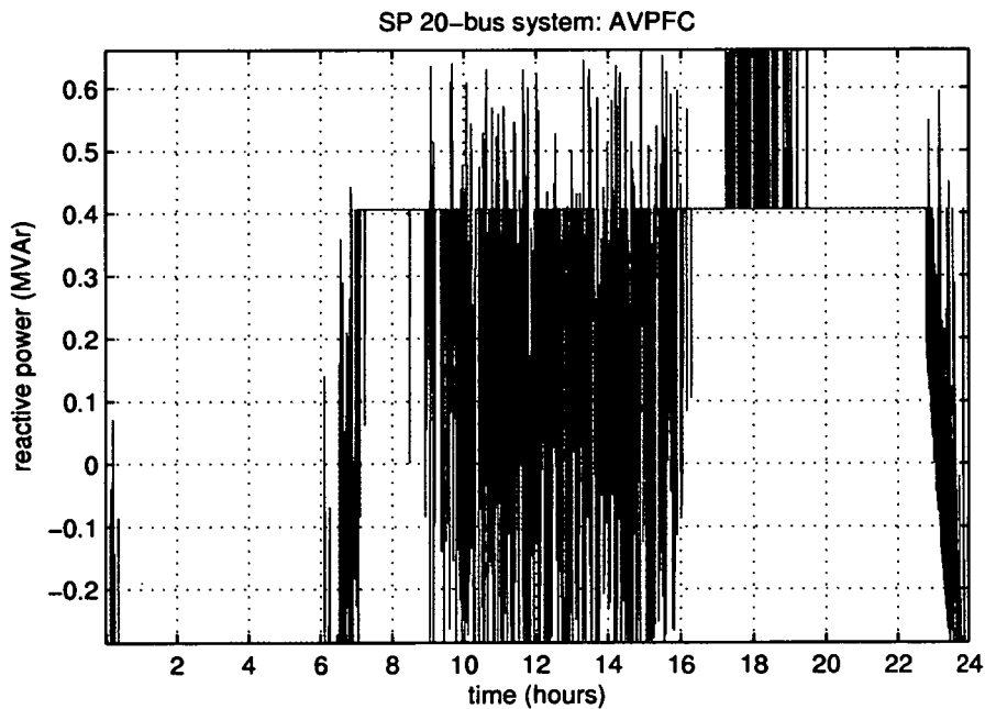
Figure 6.23: Reactive power exchange of the wind turbine operating under AVPFC control
