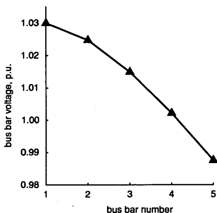
Fig. 2 Voltage profile of the radially tapered network
