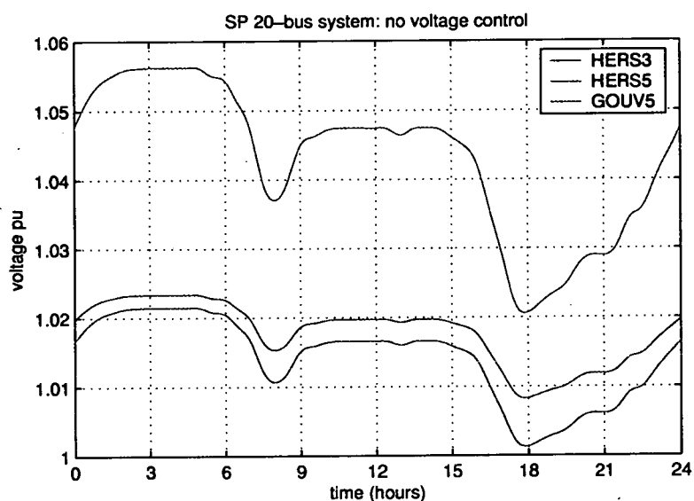
Figure 6.3: Voltage profiles of buses HERS3, HERS5 and GOUV5 after the connection of a 2MW generator at GOUV5 operating in power factor control mode
