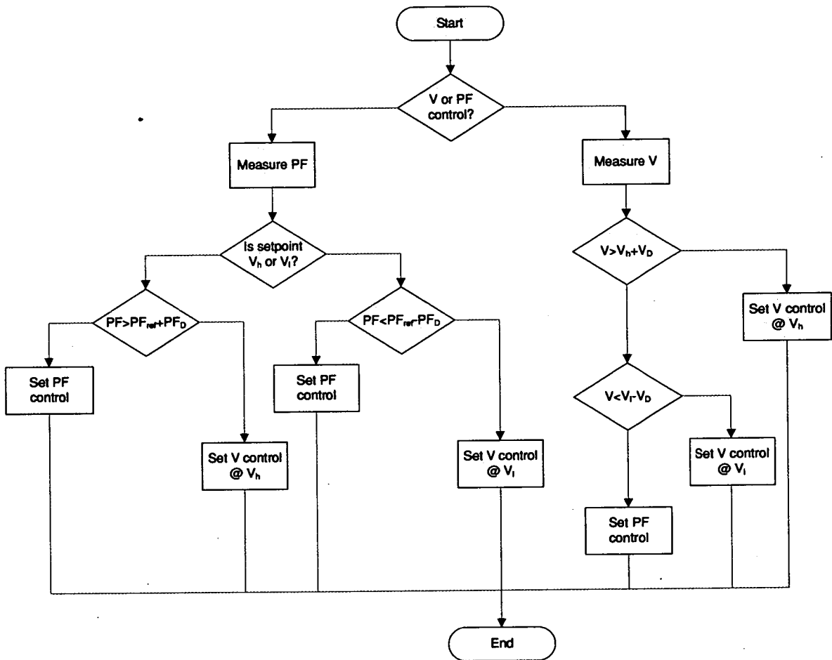
Figure 5.8: The flow chart of the automatic voltage/power factor control algorithm
