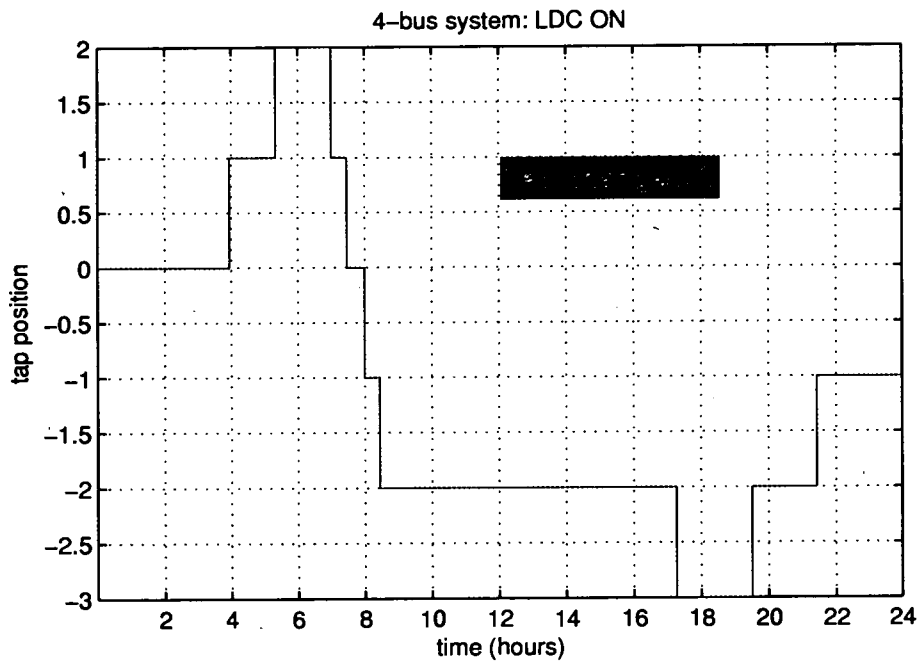
Figure 5.28: OLTC tap position during the 24-hour simulation with the AVPFC controlled WECS
