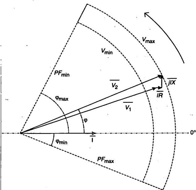
Fig. 4 Voltage vector diagram for the two-busbar system of Fig. 3
