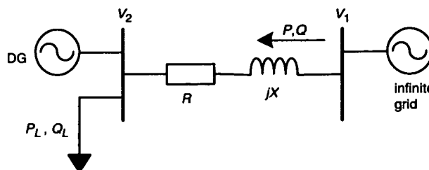
Fig. 3 Basic 2 busbar system
