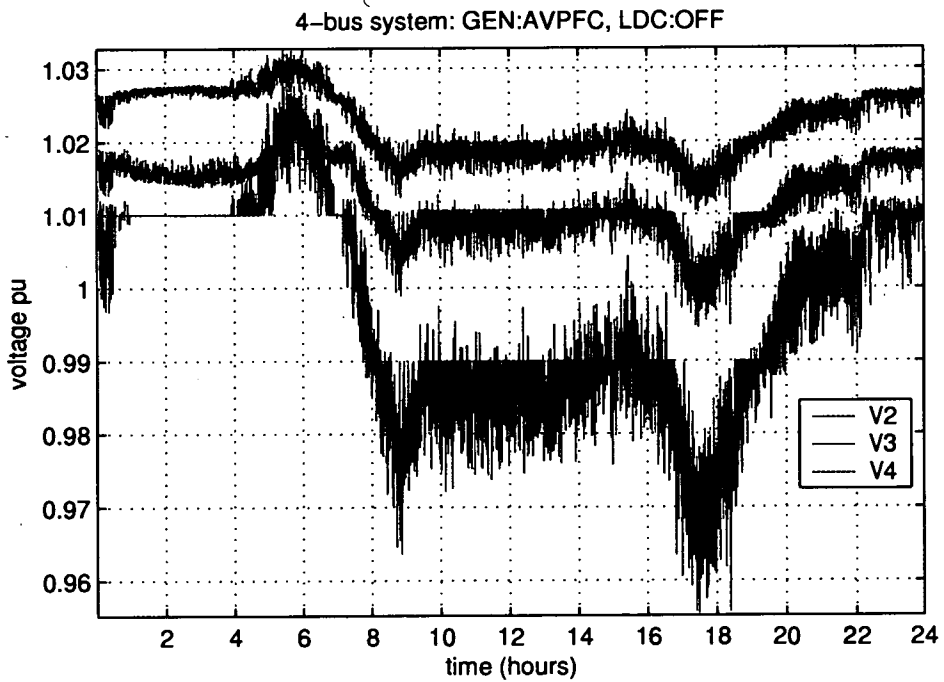
Figure 5.22: Voltage profile for the AVPFC controlled WECS
