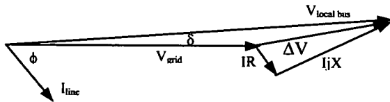
Figure 2 – Voltage Phasor Diagram
