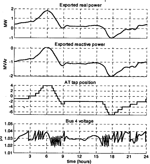
Figure 9 – LRC operation
