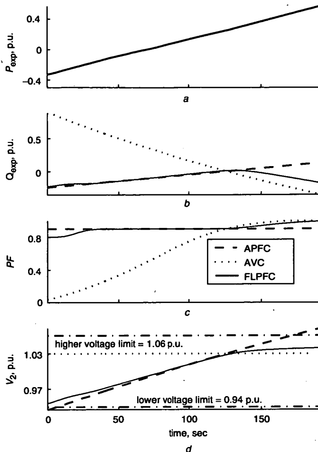
Fig. 9 DG loading-up under AVC, APFC and FLPFC control
