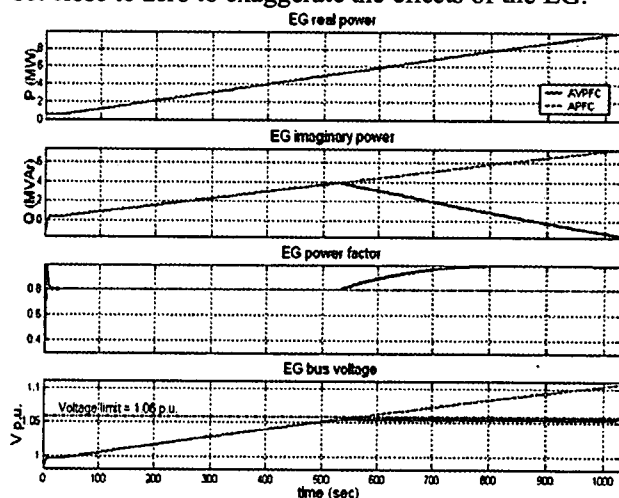
Figure 8 – Machine loading results
