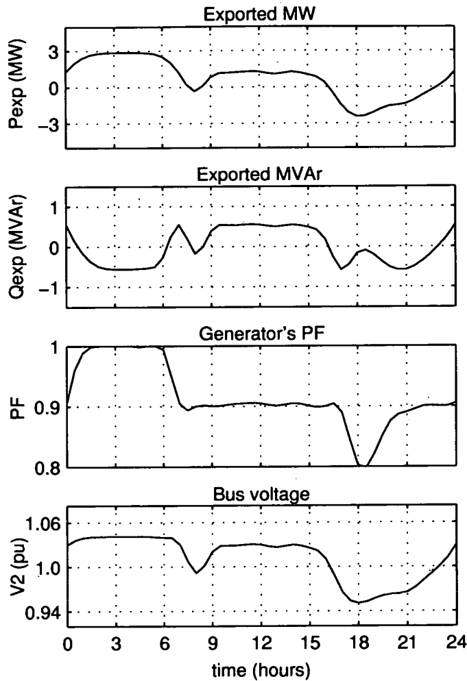
Figure 5.17: FLPFC response to 24-hour varying load
