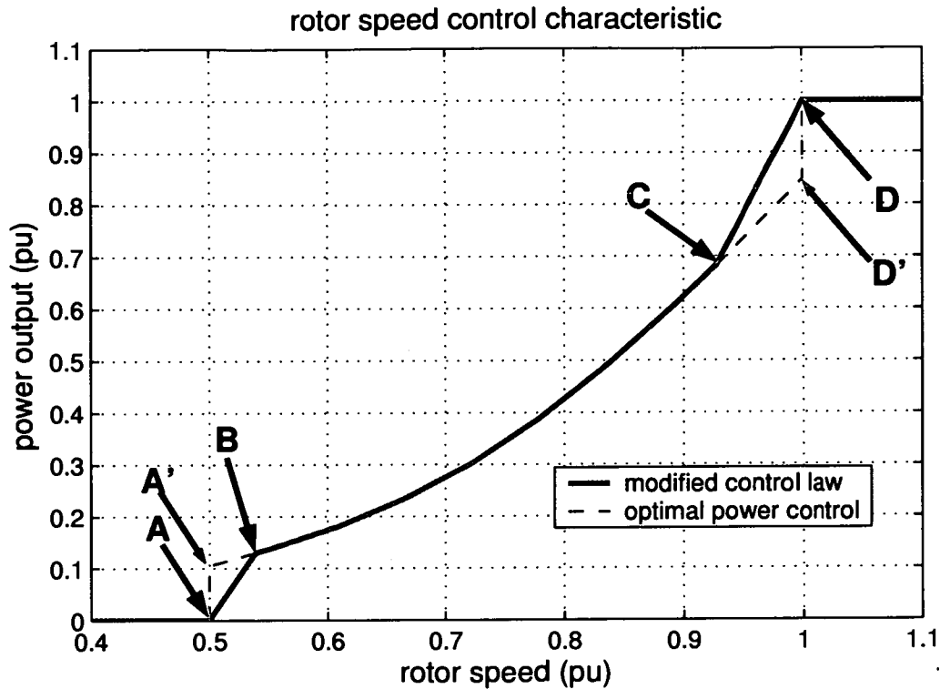
Figure 4.10: Speed control characteristic for the DFIG
