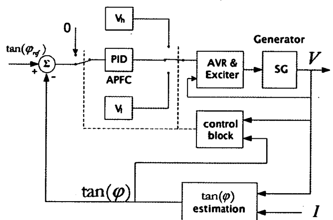
Figure 4 – AVPFC block diagram
