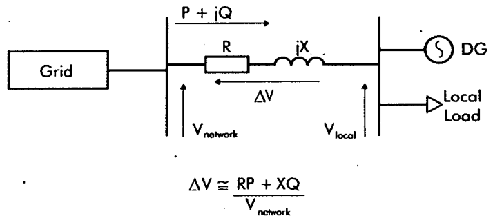
Figure 3: Voltage drop in feeder
