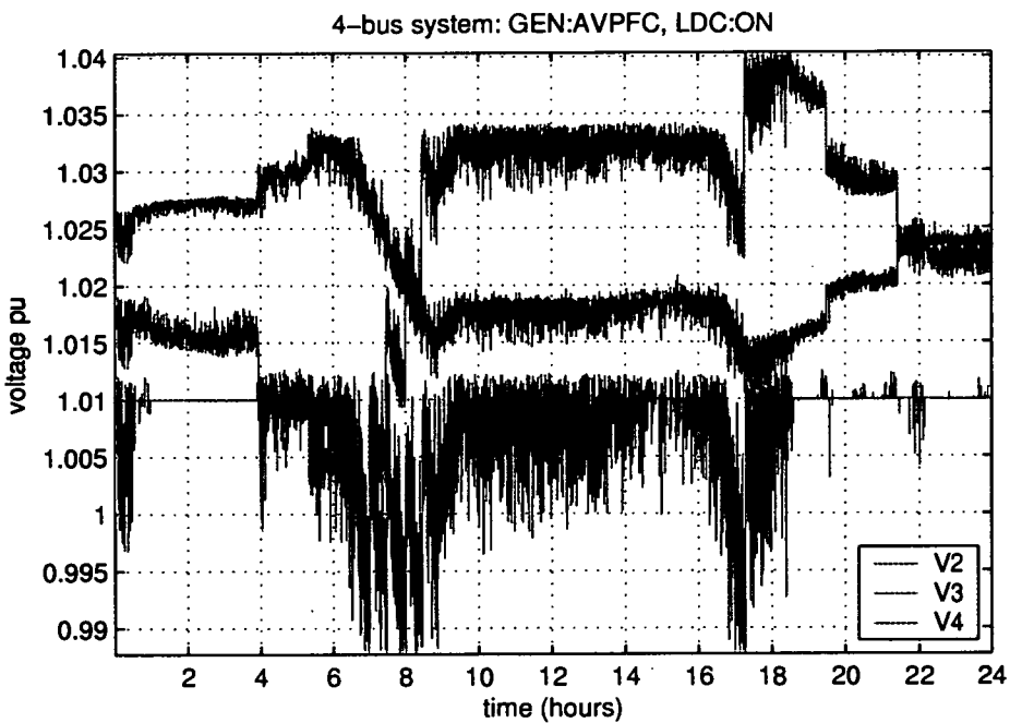
Figure 5.24: Voltage profile for the AVPFC controlled WECS with line drop / rise compensation
