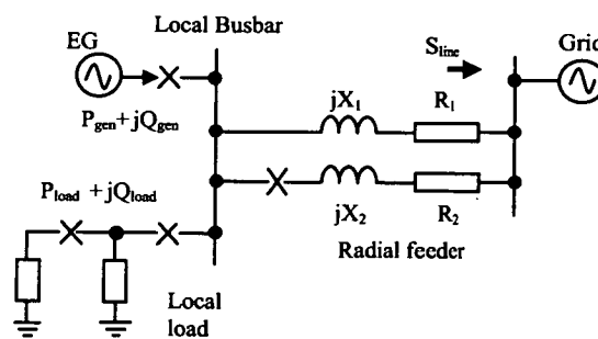
Figure 5 – Test Network
