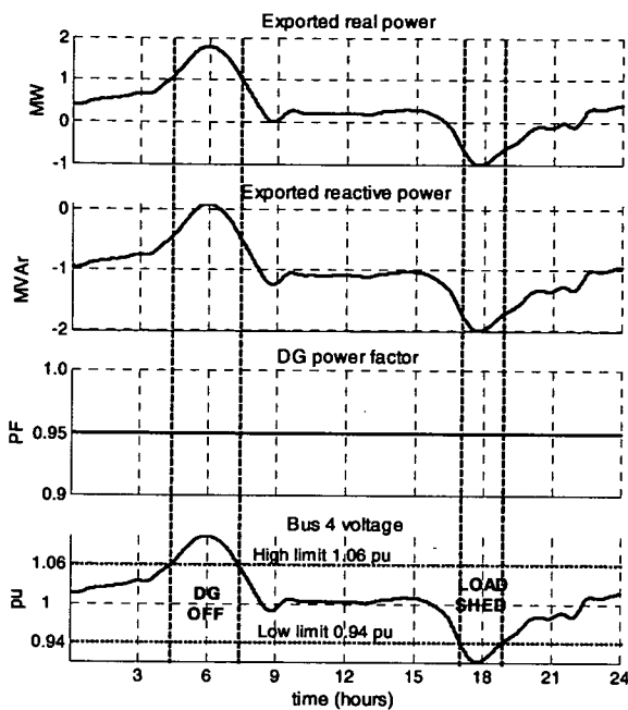
Figure 7 – APFC operation
