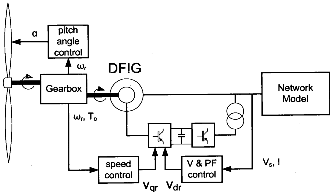
Figure 4.2: Functional diagram and power transfer in a Wind Energy Conversion System
