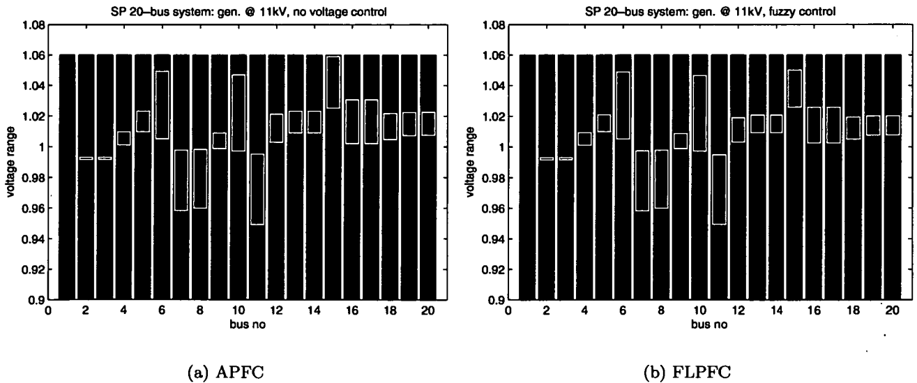
Figure 7: Network voltage ranges with APFC (a) and FLPFC (b) controlled generator on bus 15
