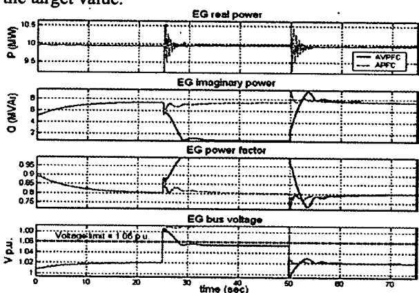
Figure 9 – Load switching results
