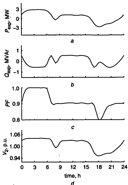
Fig. 13 FLPFC response to 24 h varying load
