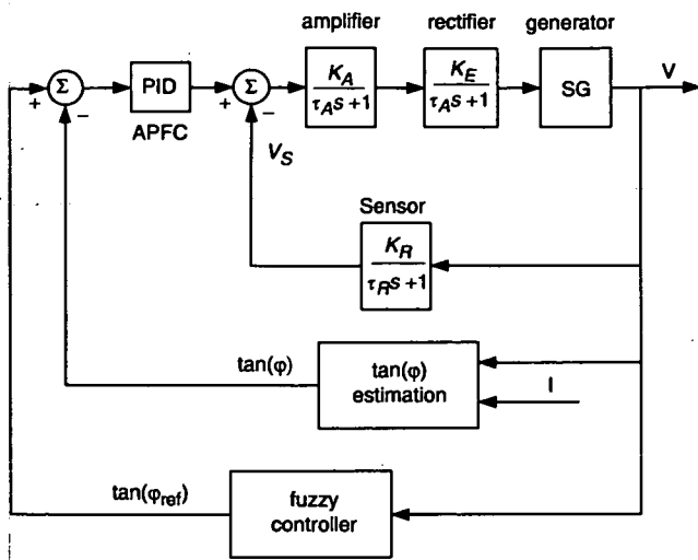
Fig. 7 Block diagram of a DG with a fuzzy logic power-factor controller
