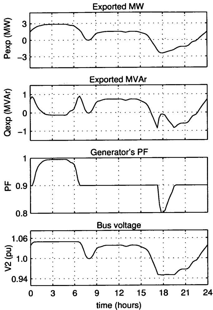
Figure 5.16: AVPFC response to 24-hour varying load
