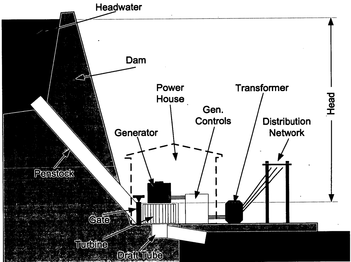
Figure 3.2: Diagram of a Small Hydro Generator Installation.
