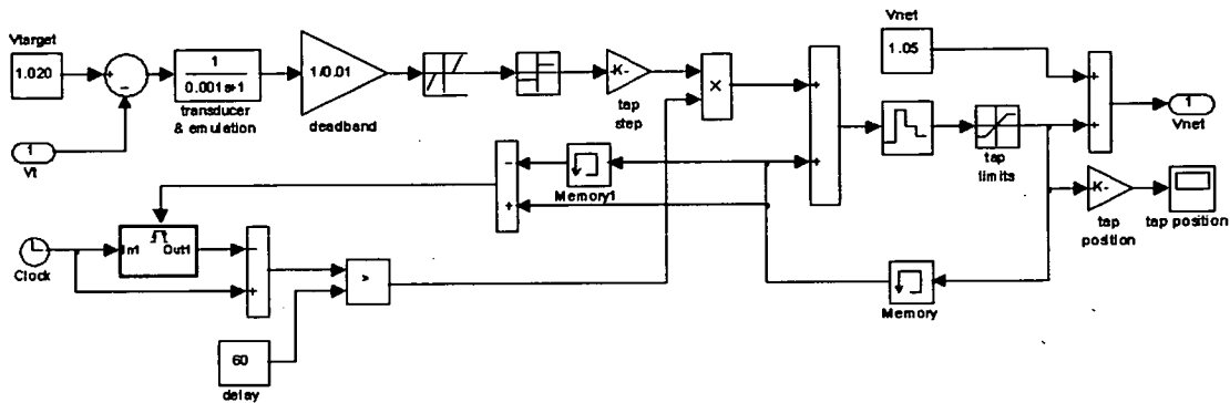
Figure 3.11: Simulink block diagram of the OLTC mechanism
