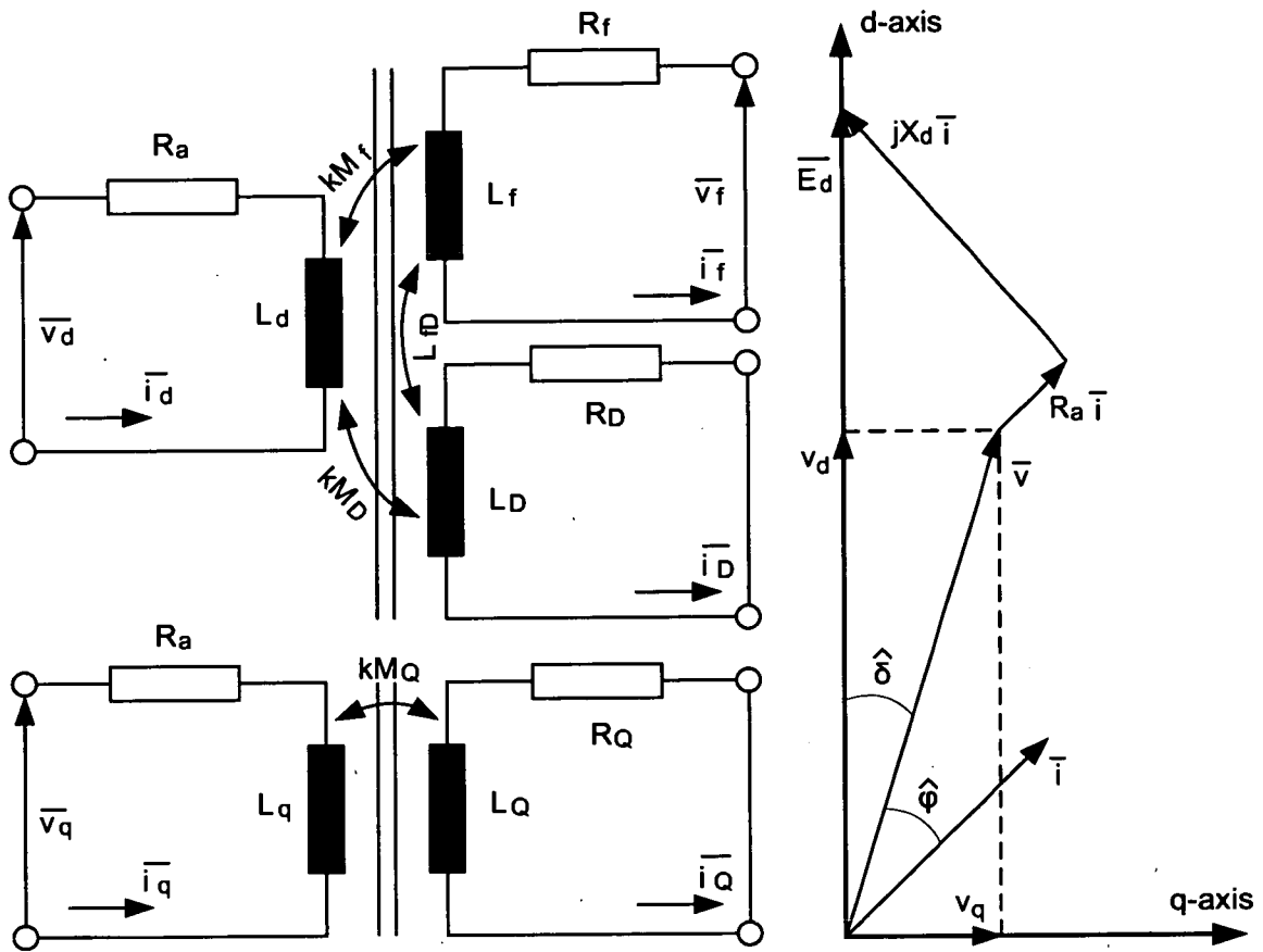
Figure 3.5: Steady state equivalent circuit of the synchronous generator (left) and terminal voltage/current vector diagram
