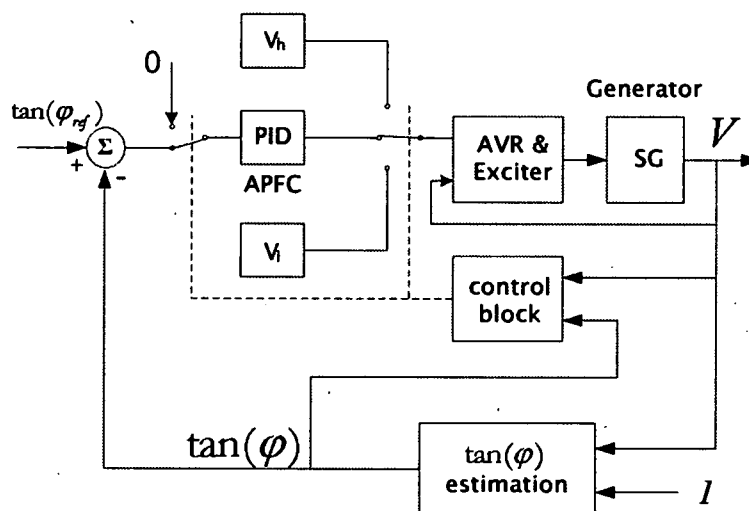
Figure 3: AVPFC block diagram
