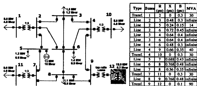
Figure 4. 12-bus 14-line test case and transformer/line characteristics
