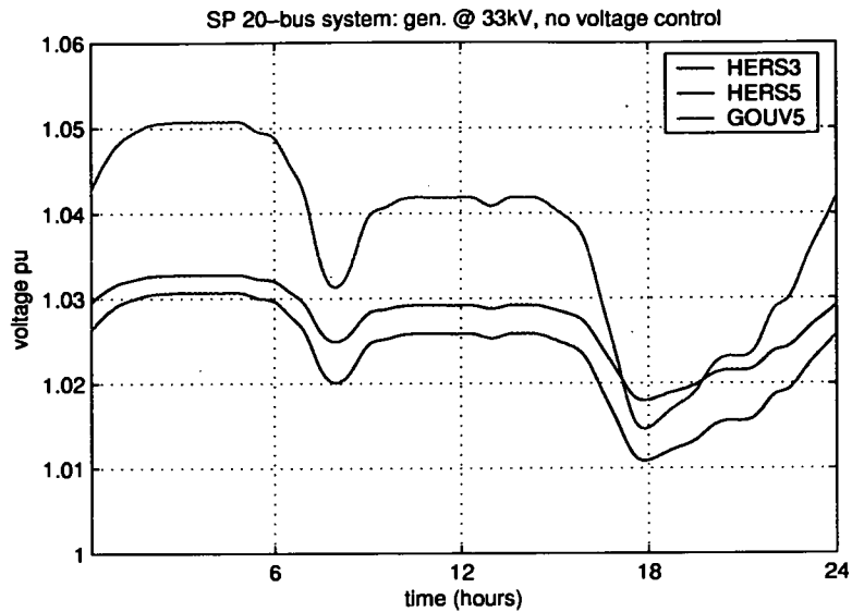
Figure 6.10: Voltage profiles of buses HERS3 , HERS5 and GOUV5 after the connection of a 8MW generator at HERS3 operating in APFC mode
