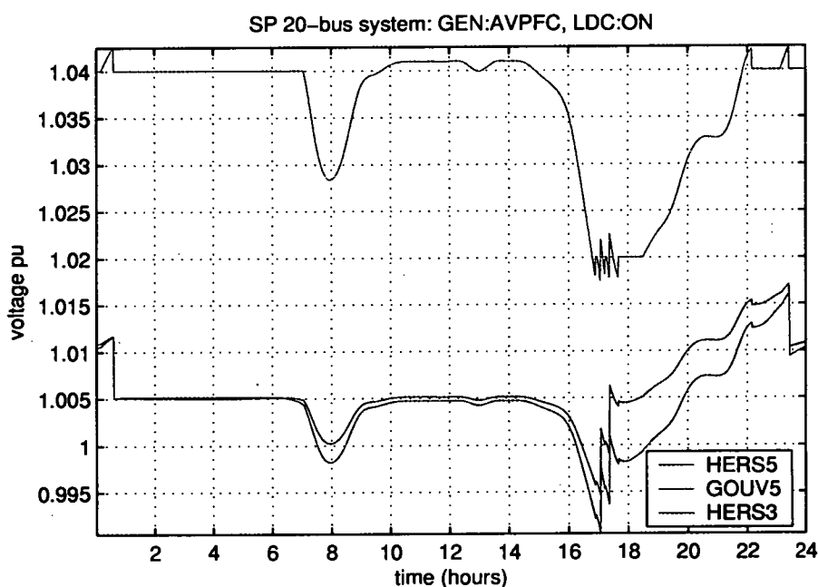
Figure 6.18: Voltage profiles for combined AVPFC and LDRC operation
