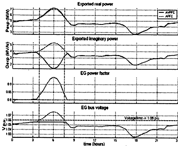
Figure 12 – Variable load results
