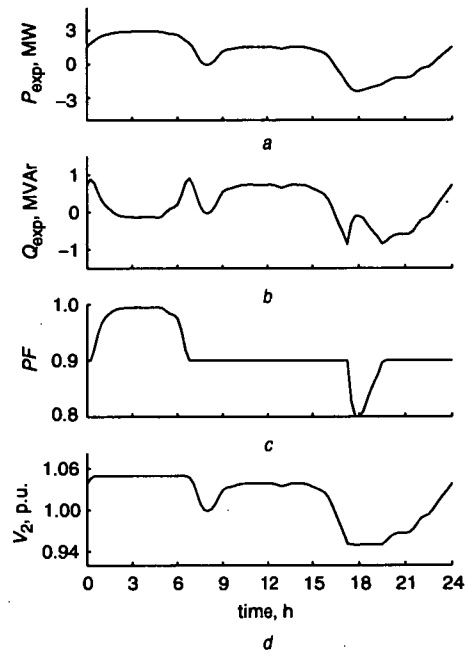
Fig. 12 AVPFC response to 24 h varying load (a) Exported MW (b) Exported MVA r (c) Generator's PF (d) Busbar voltage
