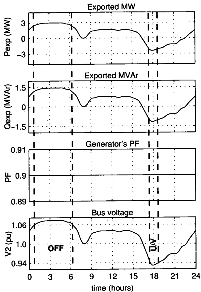
Figure 5.15: Response of APFC to a varying load
