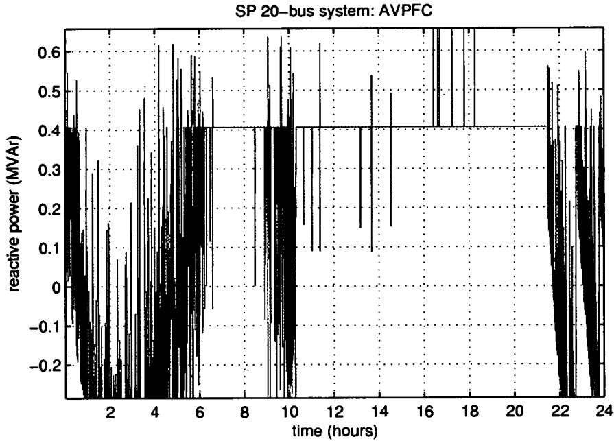
Figure 6.27: Reactive power exchange of the wind turbine operating under AVPFC control combined with LDRC
