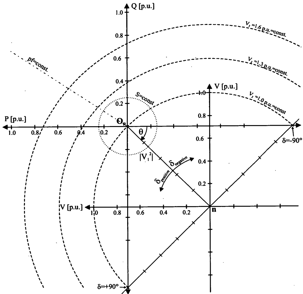
Figure 5.3: Composite universal power circle diagram
