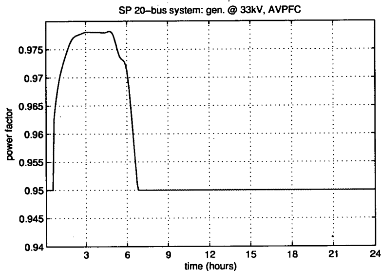
Figure 6.12: Power factor of generator at HERS3 operating in AVPFC mode
