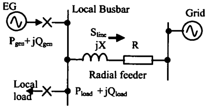
Figure 1 – Radial feeder with connected EG
