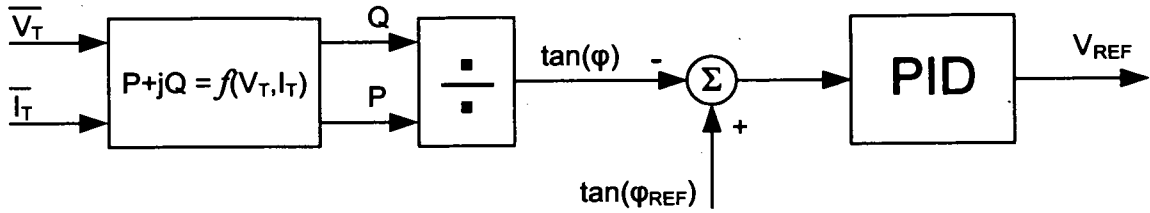
Figure 3.9: Automatic power factor controller block diagram
