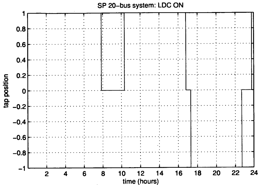
Figure 6.28: Tap changes throughout the 24-hour period with the generator in AVPFC mode
