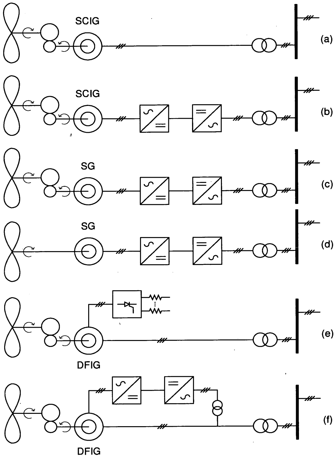
Figure 4.8: Most common generator topologies of wind energy conversion systems
