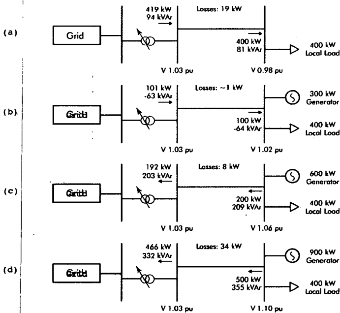
Figure 2: Changes in power flows, losses and voltages with connection of distributed generators
