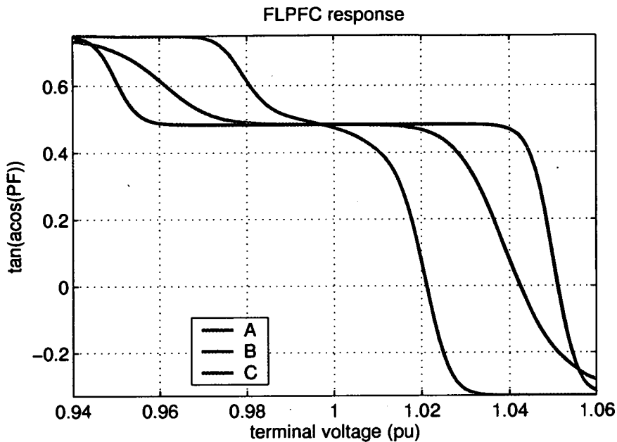
Figure 5.18: A set of three V - Q curves for the FLPFC
