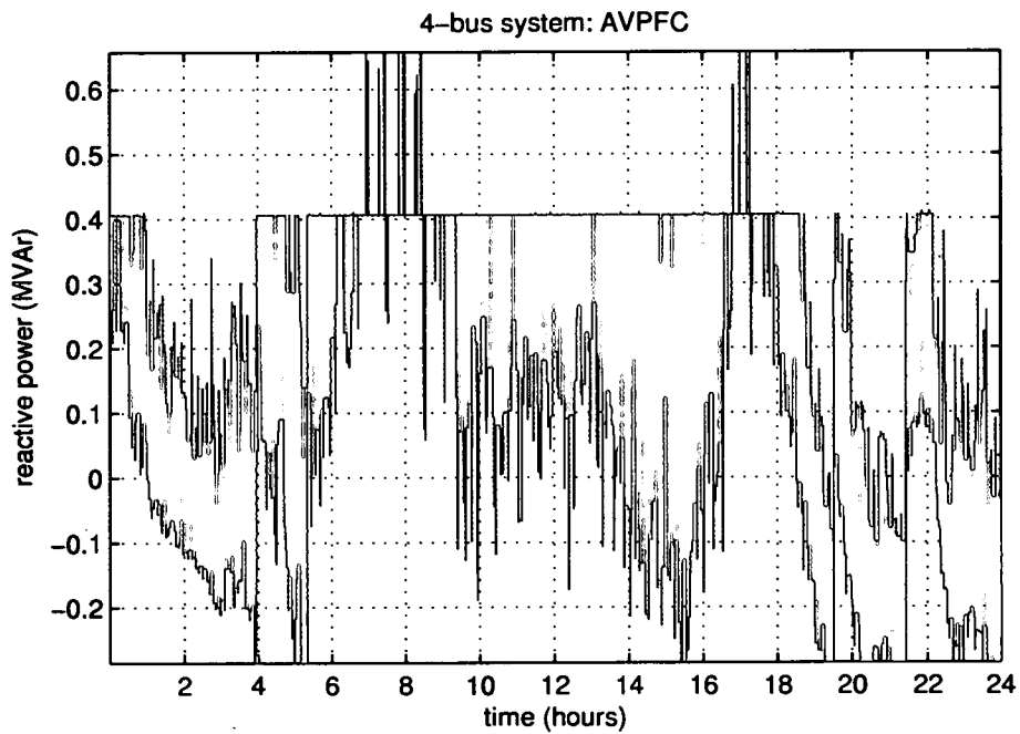
Figure 5.26: Reactive power exchange from one AVPFC controlled WECS with line drop / rise compensation
