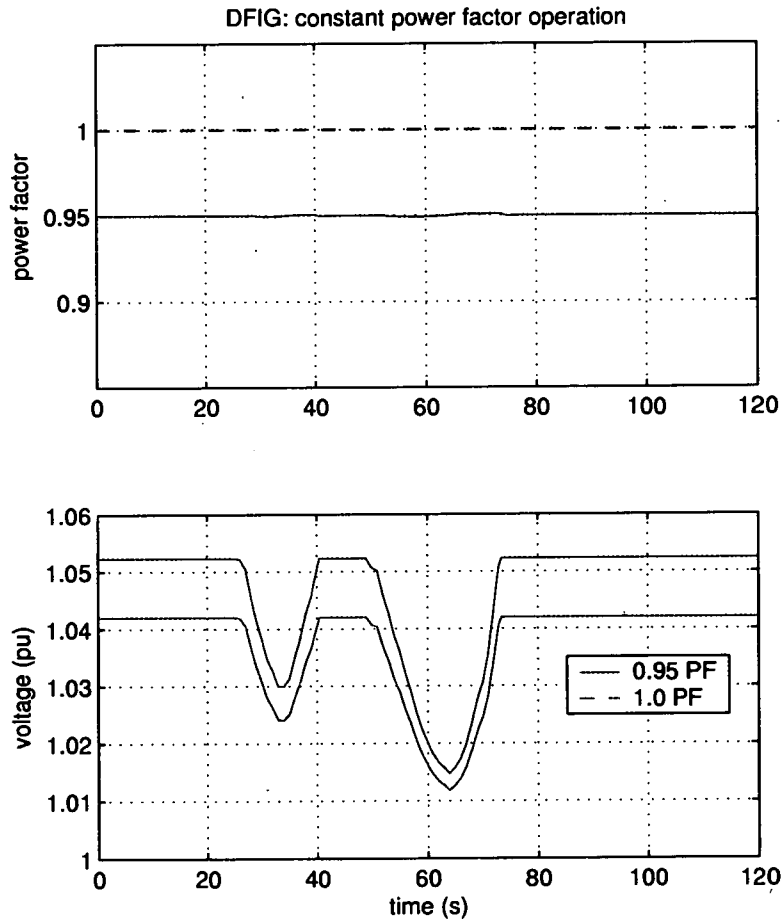
Figure 4.16: Power factor and terminal voltage for the DFIG in constant power factor mode
