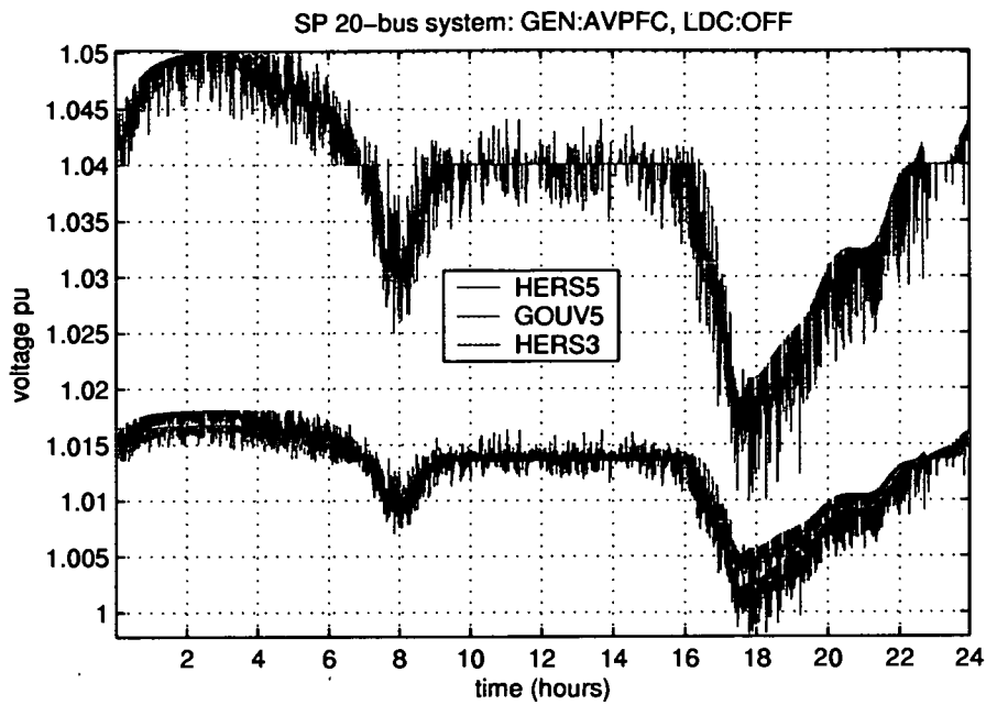
Figure 6.22: 24-hour voltage profile with the wind turbine operating under AVPFC control
