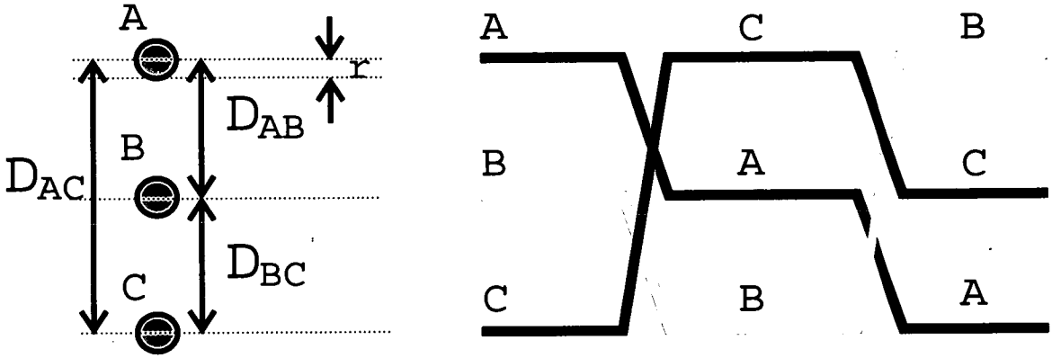
Figure 2.3: In-line configuration of conductors of a three-phase line (left) and conductor transposition (right)
