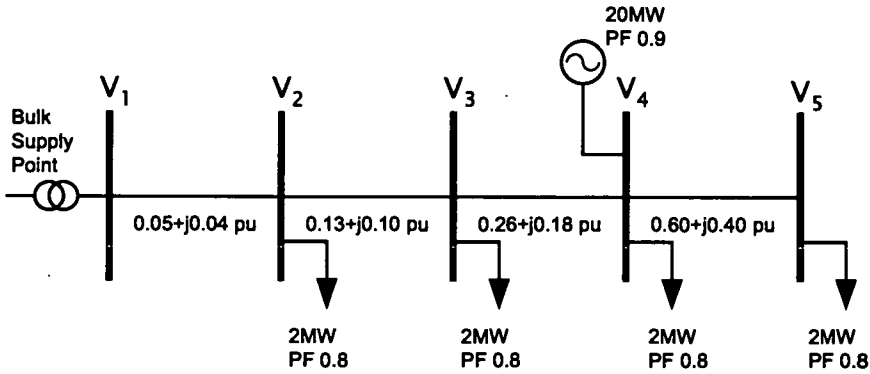
Figure 1: Radially tapered network
