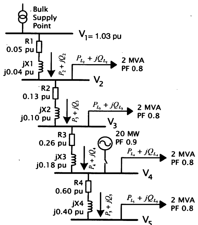
Figure 1 – Radially tapered network
