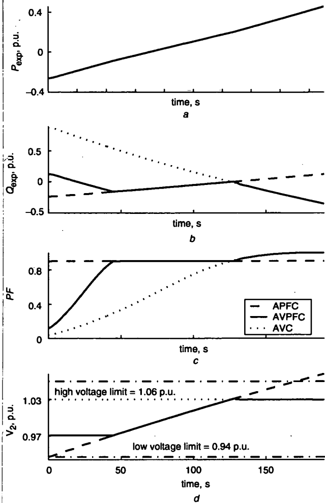
Fig. 6 DG loading-up under AVC, APFC and AVPFC control (a) Exported real power (b) Exported reactive power (c) SG power factor (d) Terminal voltage
