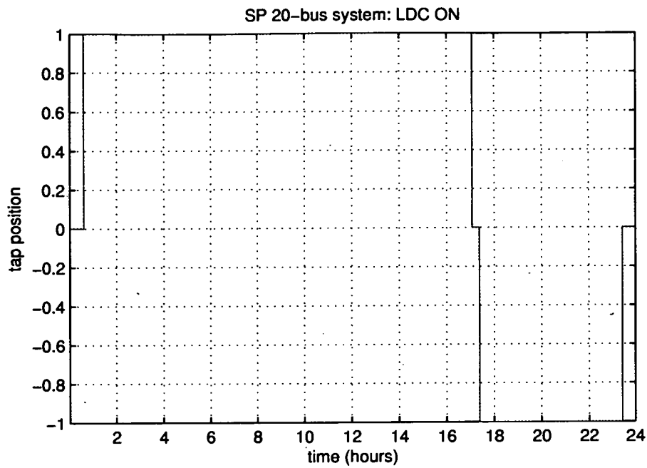
Figure 6.19: Tap transitions of the OLTC transformer with the generator under AVPFC control
