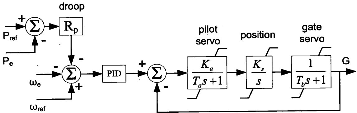
Figure 3.4: Block diagram of the hydraulic governor
