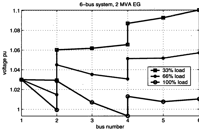
Figure 2.12: Voltage profile of the six-bus system of Figure 2.1 with 2 MVA of embedded generation on bus 6
