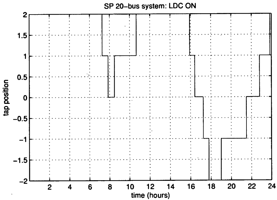
Figure 6.25: Tap changes throughout the 24-hour period with the generator in APFC mode
