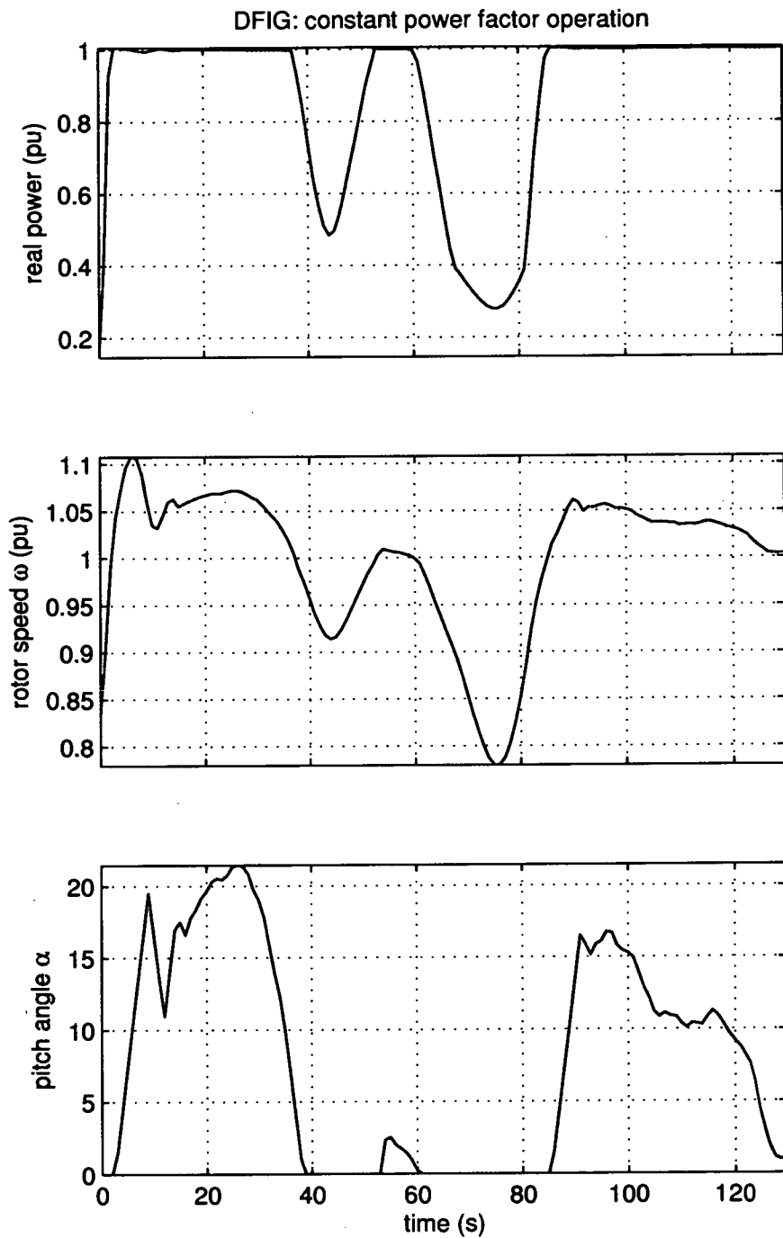
Figure 4.15: Real power export, rotor speed and blade pitch angle for the DFIG in constant power factor operation
