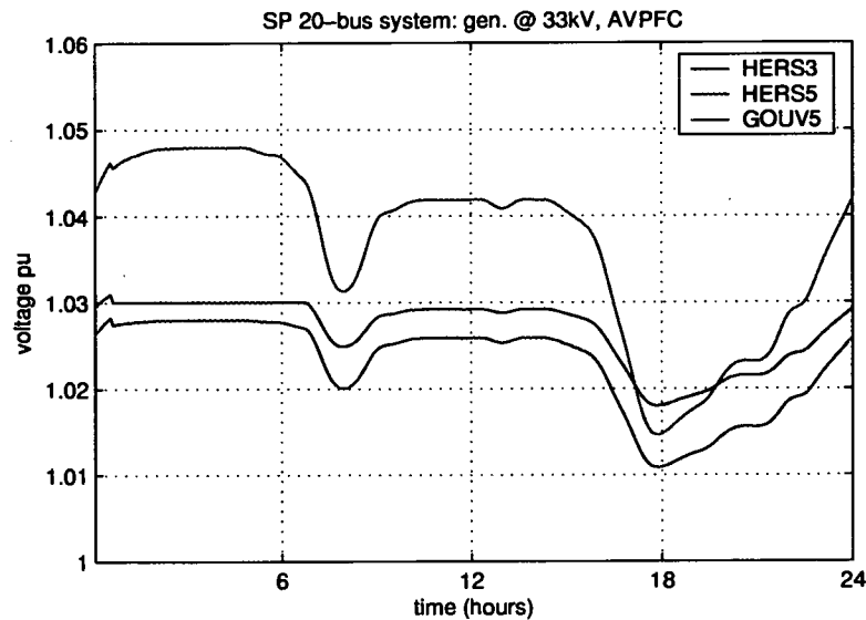
Figure 6.11: Effect of operating the generator at HERS3 in AVPFC mode on the voltage profiles of buses HERS3 , HERS5 and GOUV5
