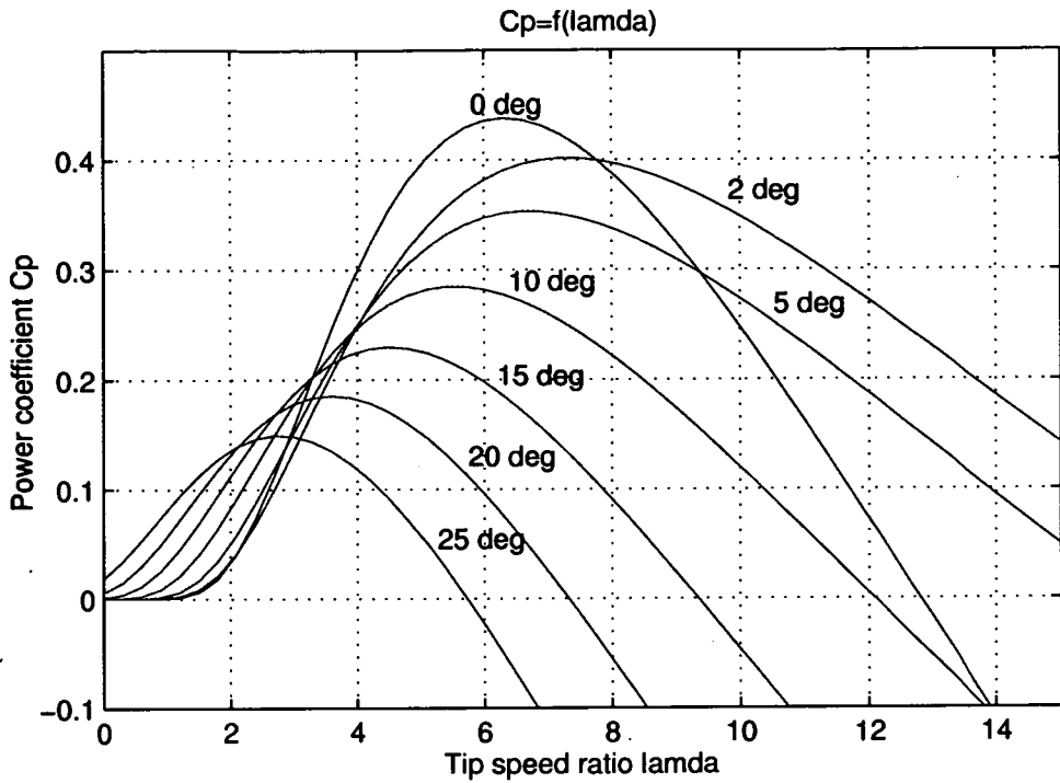
Figure 4.6: Power coefficient versus tip speed ratio for various values of blade pitch angle. Regenerated after Slotweg et al., 2001
