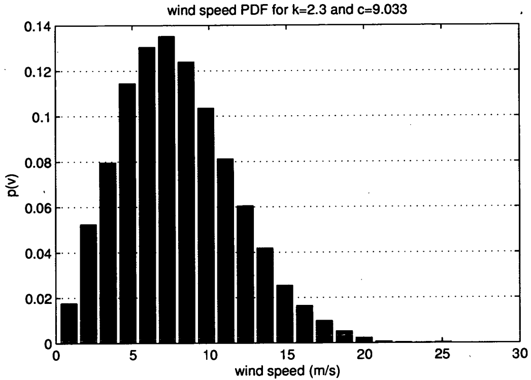
Figure 4.3: Probability density function for a wind speed time series with k=2.3 and c=9.033 .
