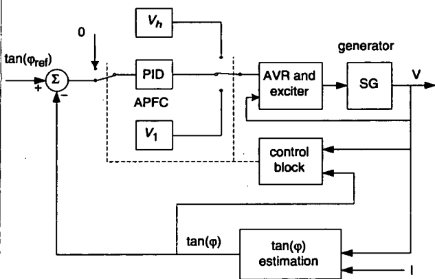
Fig. 5 AVPFC-controlled synchronous generator block diagram
