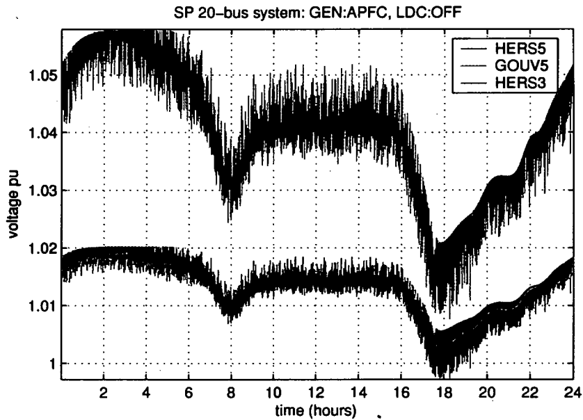
Figure 6.21: 24-hour voltage profile with the wind turbine operating in APFC
