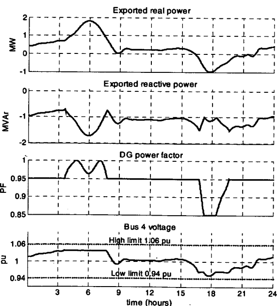
Figure 8 – AVPFC operation
