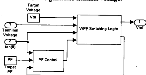
Figure 7 – Auto Voltage/Power Factor Controller
