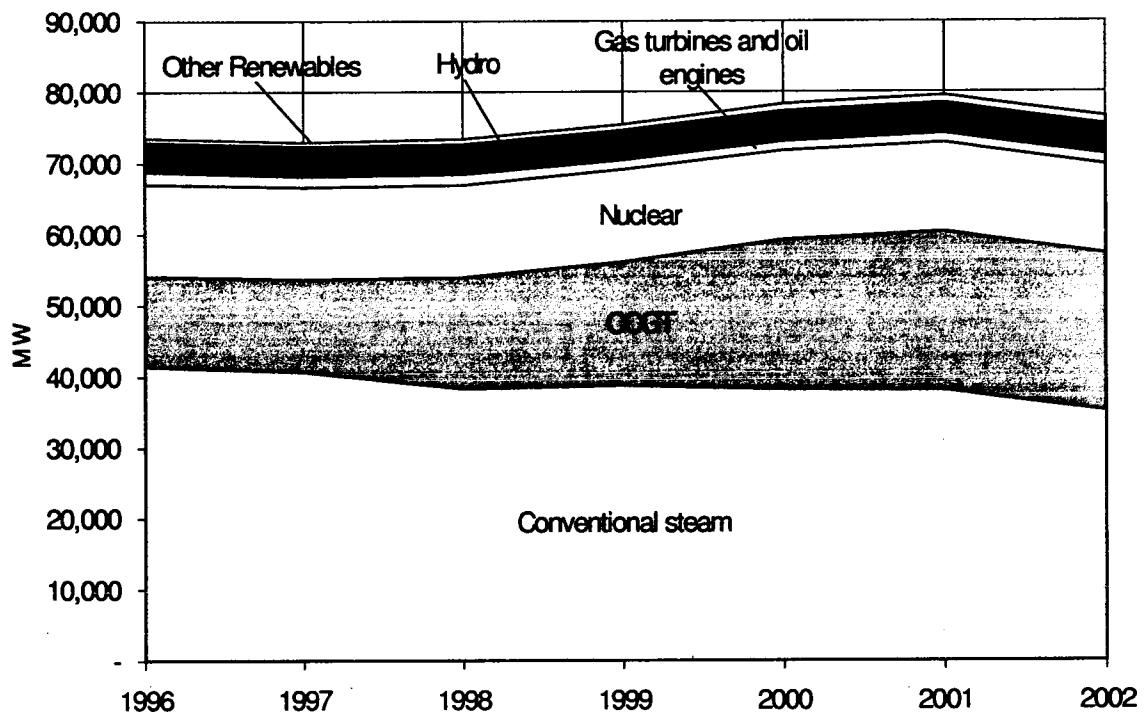
Figure 1.2: Capacity per plant type in the UK from 1996 to 2002, DUKES 2002
