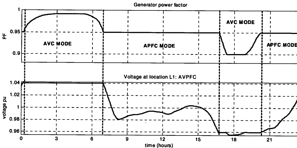
Figure 7: Generated power factor and voltage at location L1 (AVPFC mode)
