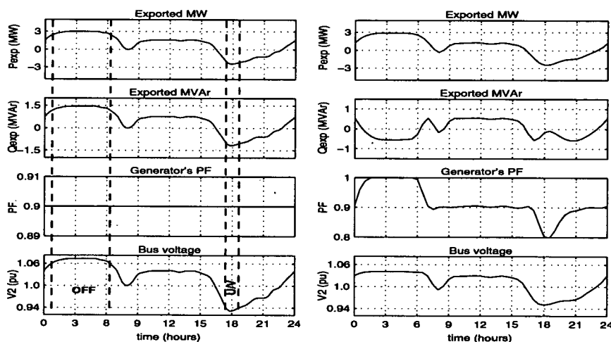
(a) APFC response
