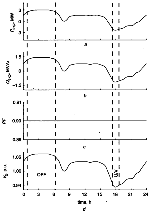
Fig. 11 Response of APFC to varying load (a) Exported MW (b) Exported MVA r (c) Generator's PF (d) Busbar voltage
