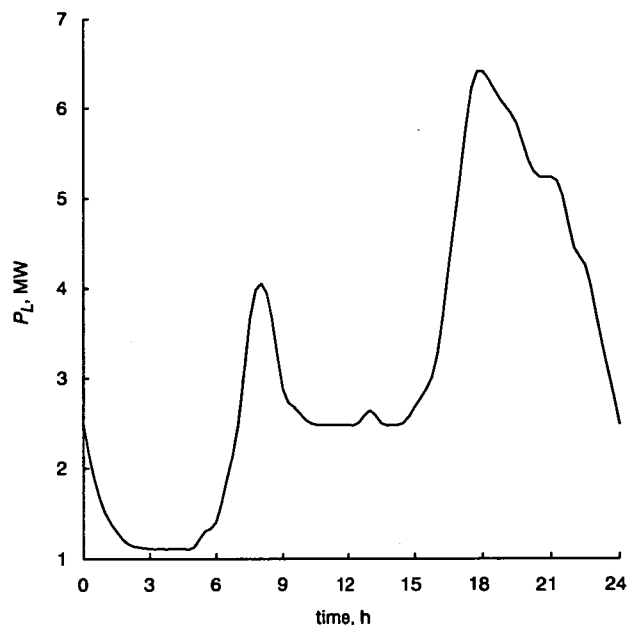
Fig. 10 24 h, 80% domestic 20% industrial load profile (0.9 PF)
