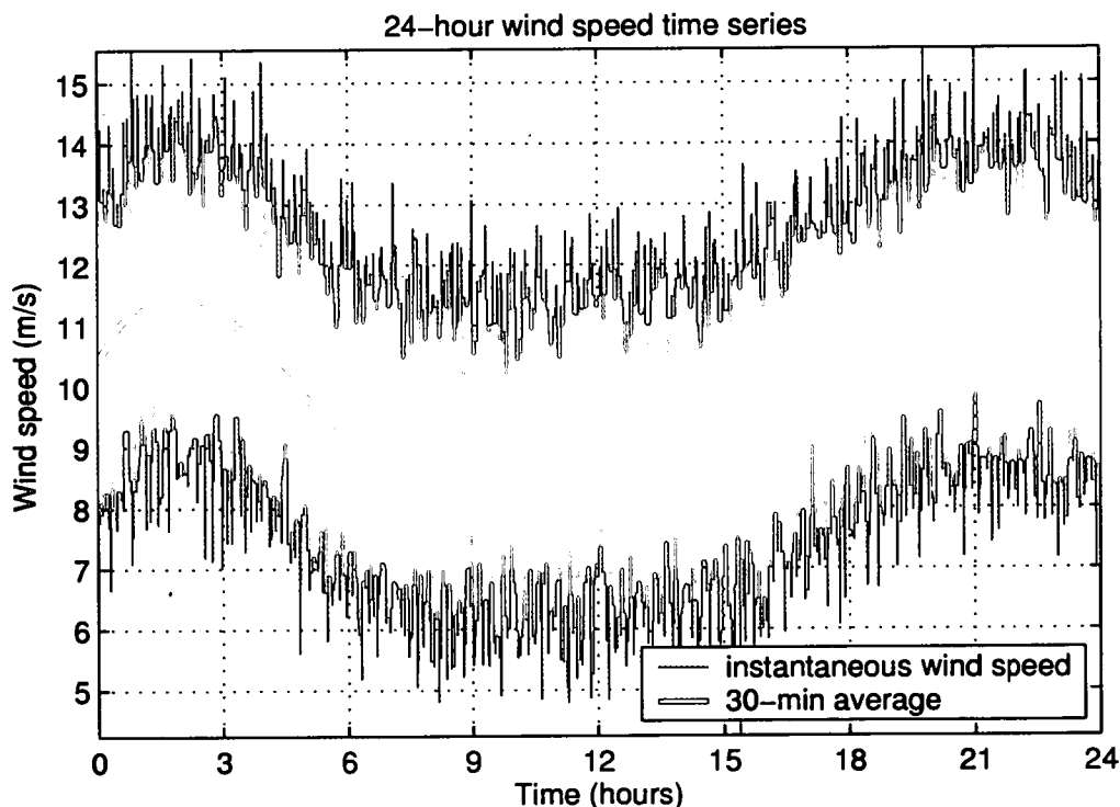
Figure 4.4: Wind speed time series sampled at 1 Hz (blue) and 30 min. average (red)
