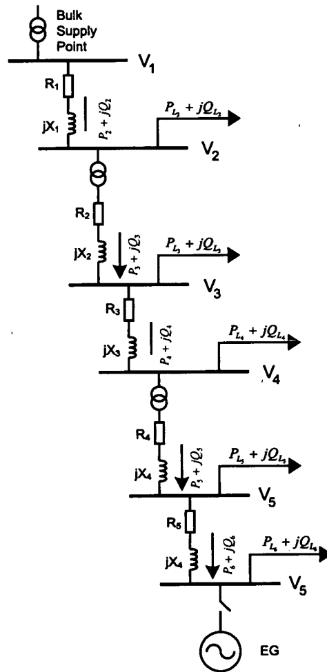
Figure 2.1: A section of a common distribution network consisting of a tapered radial feeder with loads
