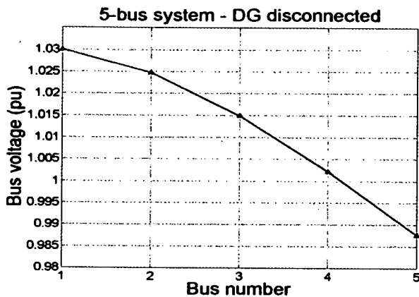
Figure 2 – Voltage profile with the DG disconnected
