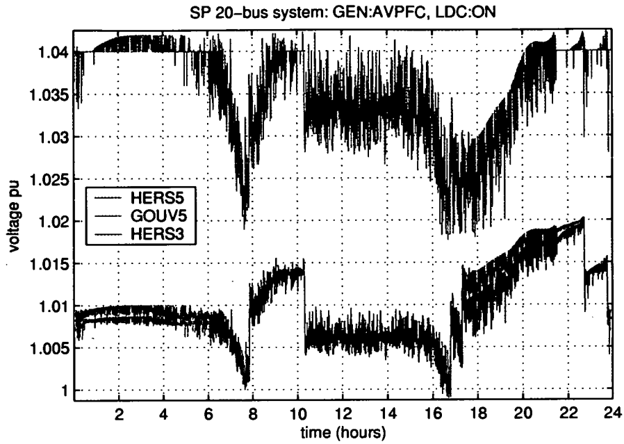
Figure 6.26: 24-hour voltage profile with the wind turbine operating under AVPFC control combined with LDRC
