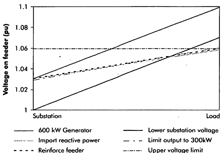
Figure 4: Feeder voltage profile and mitigation measures
