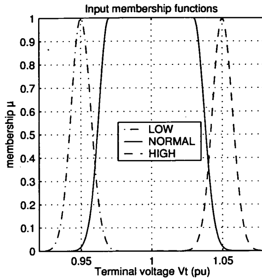
Figure 5.11: Input membership functions of the Fuzzy Power Factor Controller
