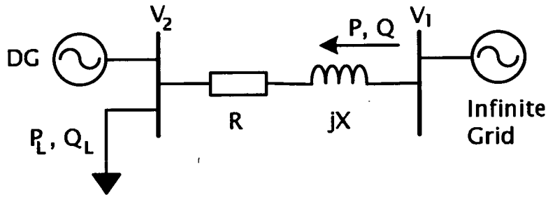
Figure 5.1: Basic 2 bus system
