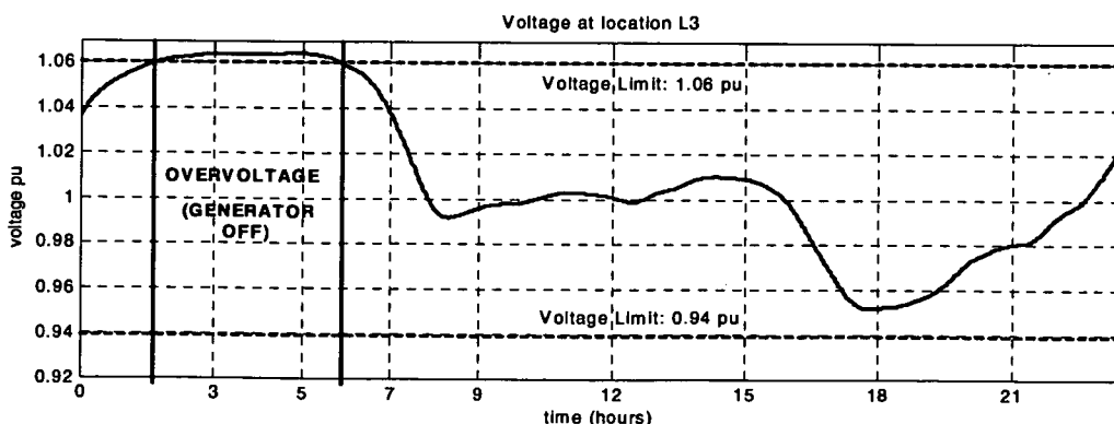
Figure 8: Voltage at location L3 (APFC mode)
