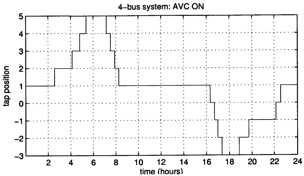
Figure 3.17: OLTC tap position for the 24-hour simulation (AVC)
