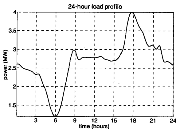
Figure 6 – Profile of load on bus 4
