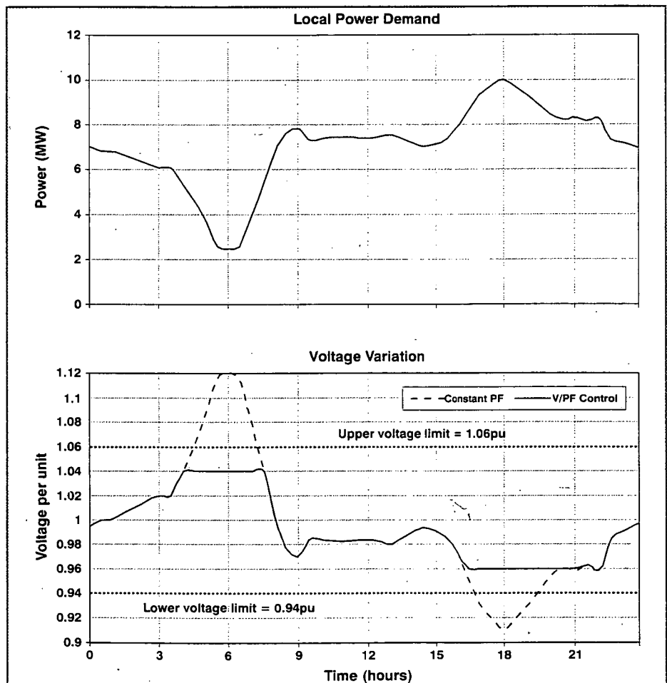
Figure 2: 24-h voltage profile due to load variations with and without hybrid control
