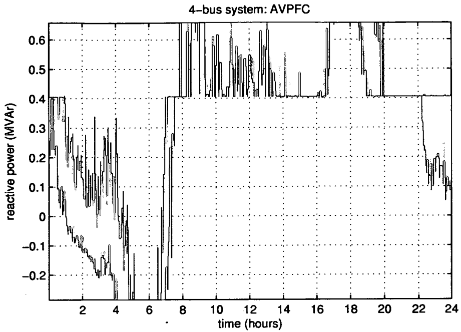
Figure 5.25: Reactive power exchange from one AVPFC controlled WECS
