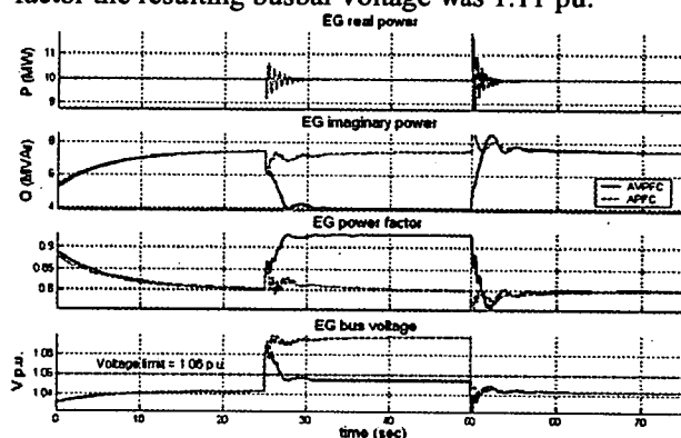
Figure 10 – Line switching results
