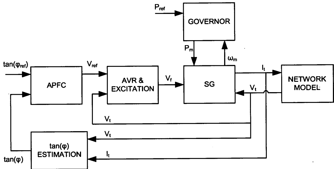
Figure 3.3: Top-level block diagram of the developed model for the small-hydro plant
