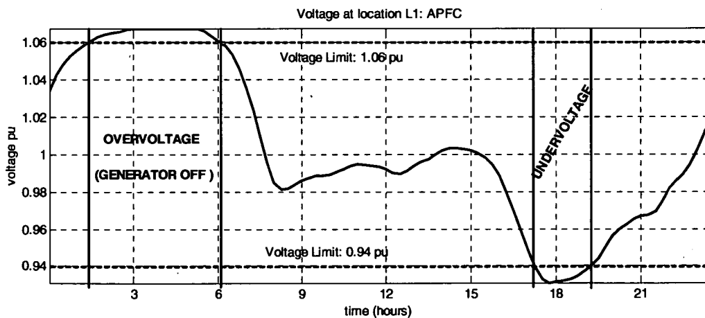
Figure 6: Voltage at location L1 (APFC mode)
