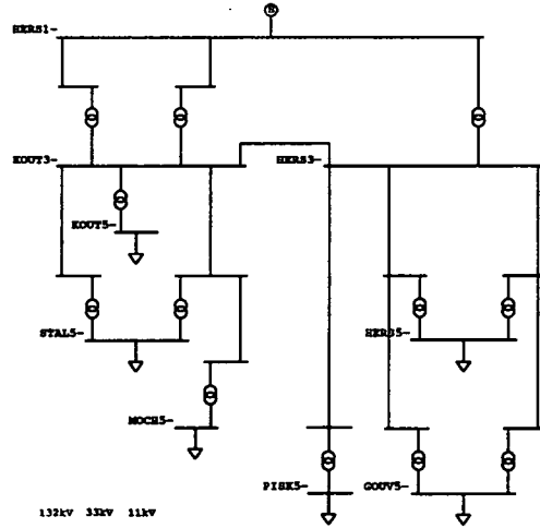
Figure 6: The section of the scottish distribution network used as a test system
