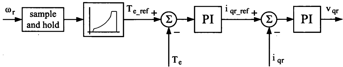
Figure 4.11: Speed controller for the wind turbine
