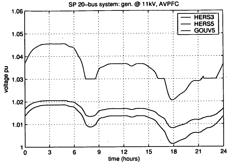
Figure 6.4: Effect of operating the generator at GOUV5 in AVPFC mode on the voltage profiles of buses HERS3, HERS5 and GOUV5
