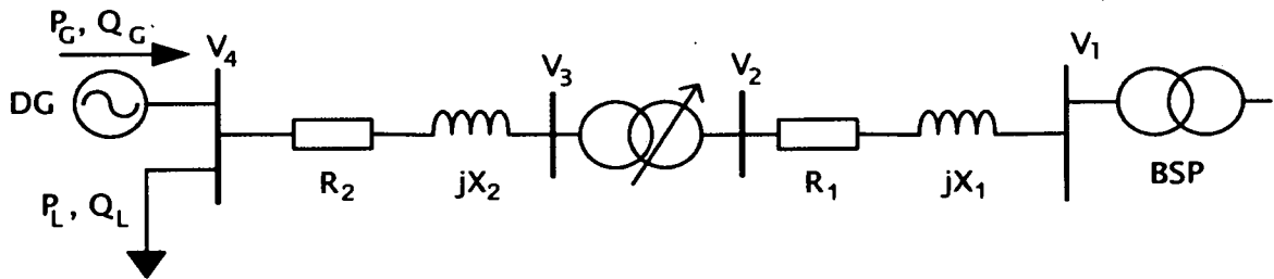
Figure 3.15: The simulated 4-bus system with the OLTC
