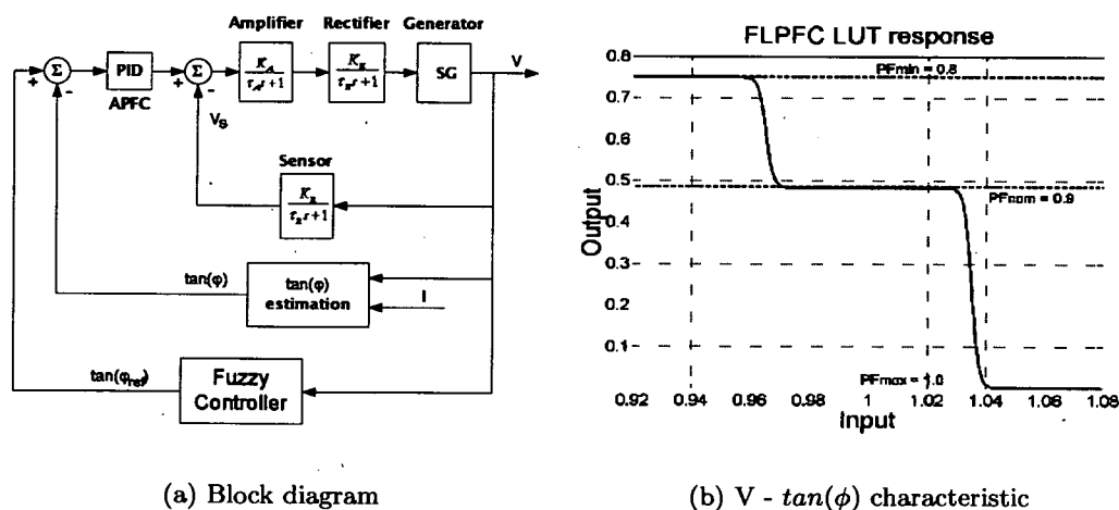
Figure 4: Block diagram of a DG with an FLPFC and its response to voltage changes
