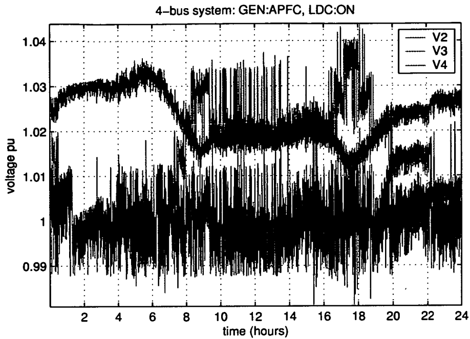
Figure 5.23: Voltage profile for the APFC controlled WECS with line drop / rise compensation
