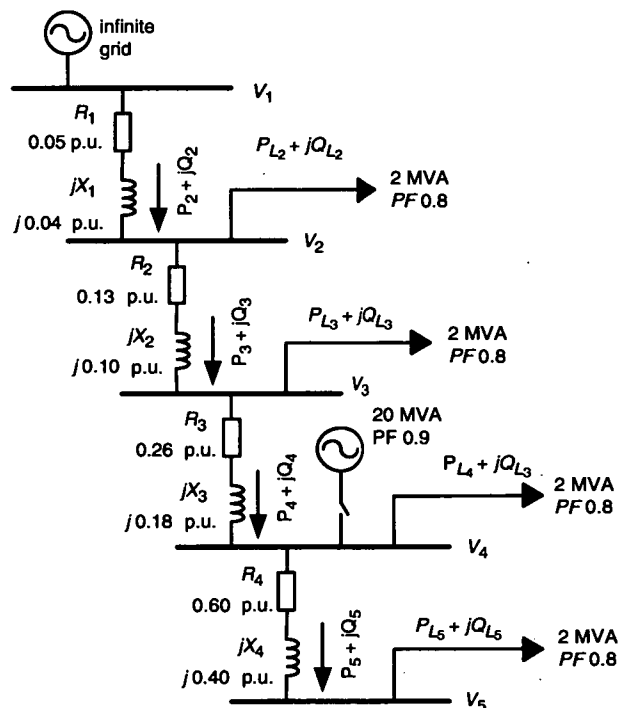
Fig. 1 Radially tapered network
