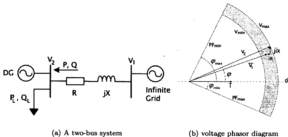
Figure 3: Basic power network
