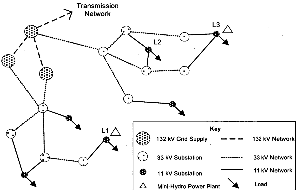
Figure 5: The test network
