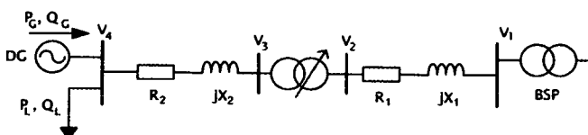
Figure 5 – AT with OLTC in the DN
