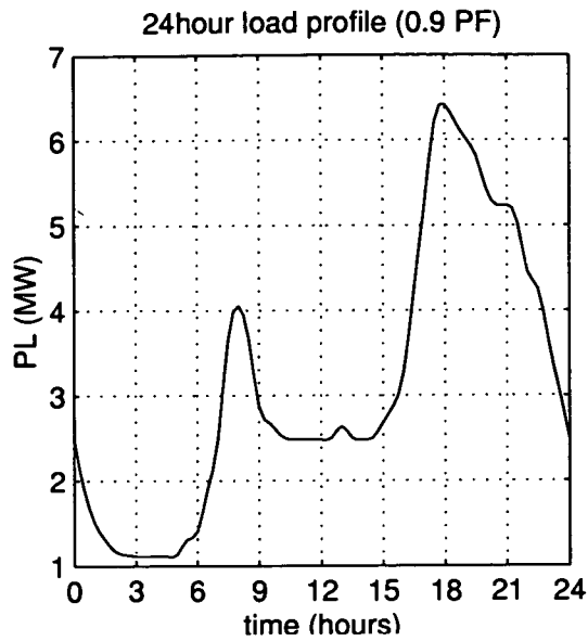
Figure 5.14: 24-hour, 80% domestic 20% industrial load profile
