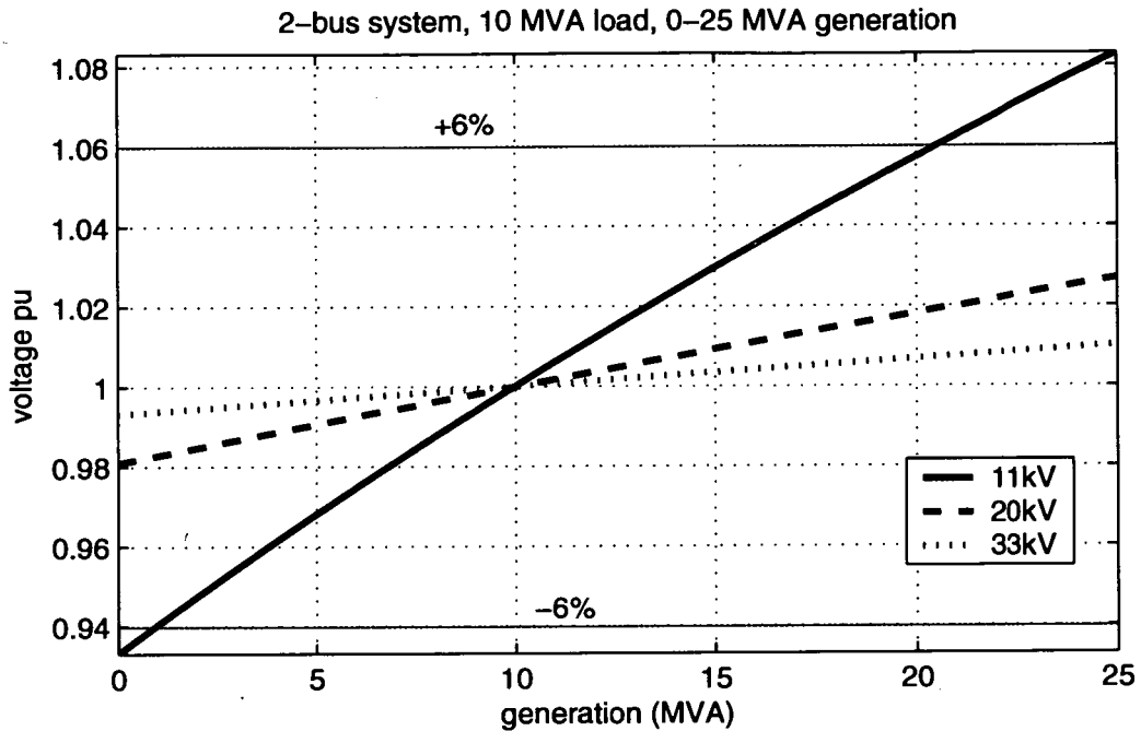
Figure 2.9: Voltage variation at the load bus of the two-bus system for type ACSR54/9 conductor and for three operating voltage levels
