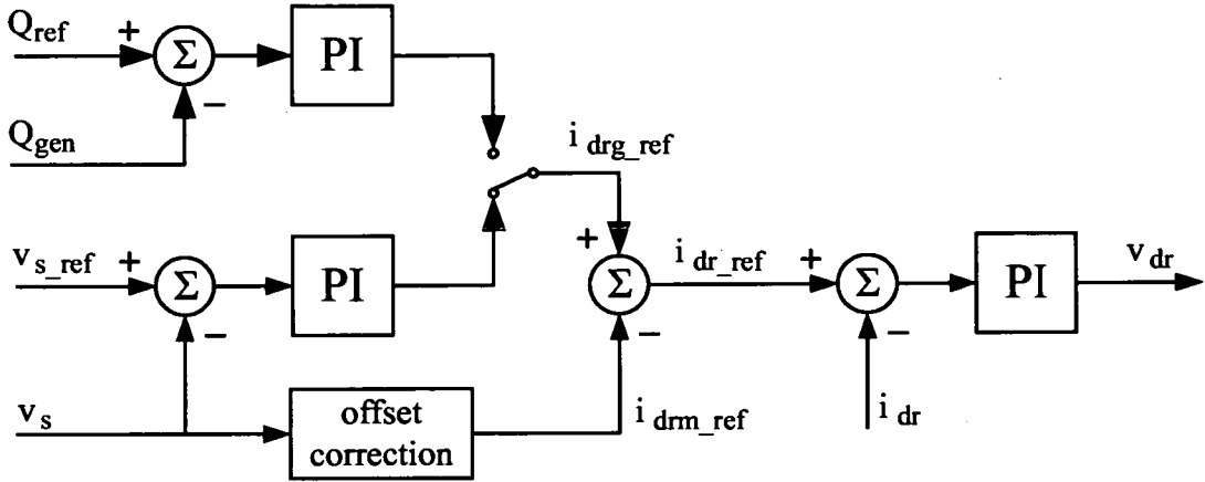
Figure 4.12: Voltage / reactive power controller for the DFIG
