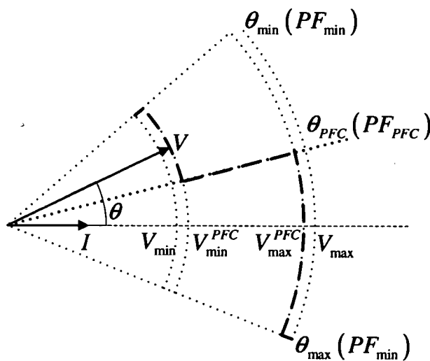
Figure 1 Hybrid AVPFC voltage control.
