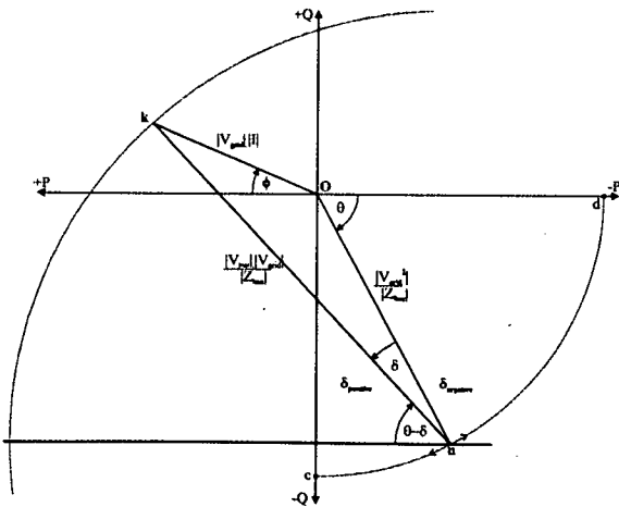
Figure 3 – UPCD for short distribution line
