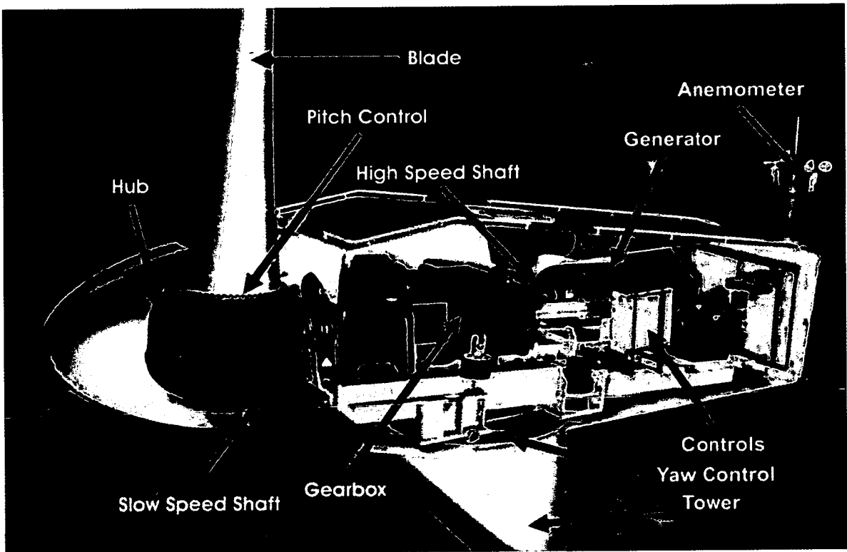
Figure 4.1: Diagram of a 3-blade, horizontal axis wind turbine, image courtesy of Vestas
