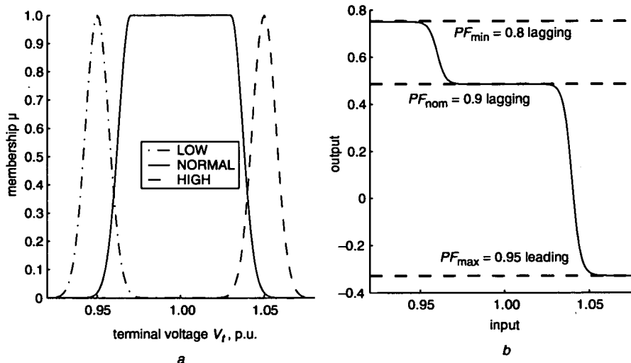
Fig. 8 Input membership functions
