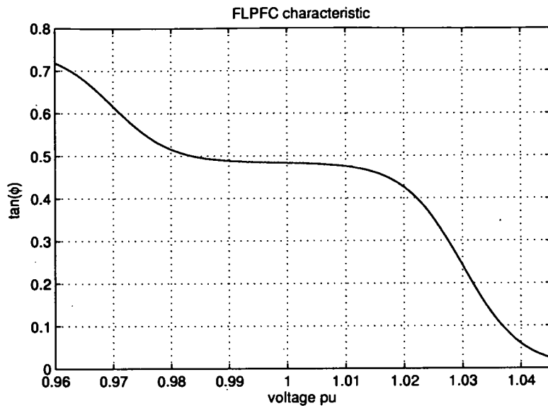
Figure 6.8: Volt- \tan(\phi) characteristic of the FLPFC
