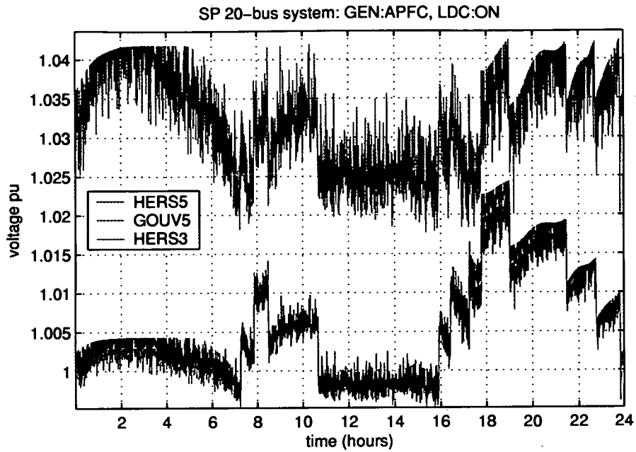
Figure 6.24: 24-hour voltage profile with the wind turbine in APFC mode assisted by line drop/rise compensation
