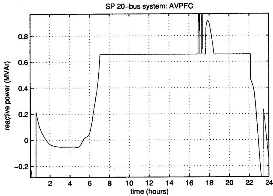
Figure 6.20: Reactive power exchange of the generator under AVPFC control
