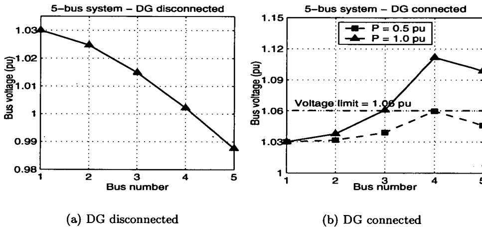
Figure 2: Voltage profile of the radially tapered network
