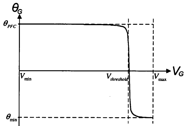
Figure 3. Smoothing of control strategy transition for Intelli-Gens.
