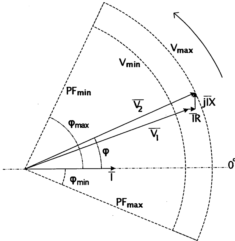
Figure 5.6: Voltage vector diagram for the two-bus system of Figure 5.1
