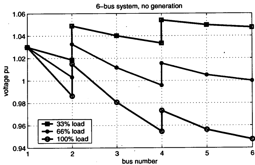
Figure 2.11: Voltage profile of the six-bus system of Figure 2.1 with no embedded generation
