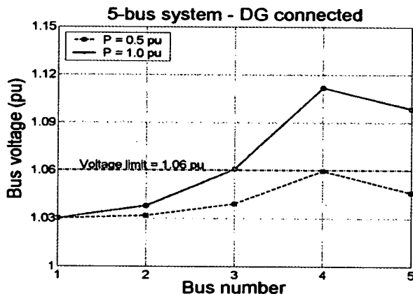
Figure 3 – Voltage profile with the DG connected
