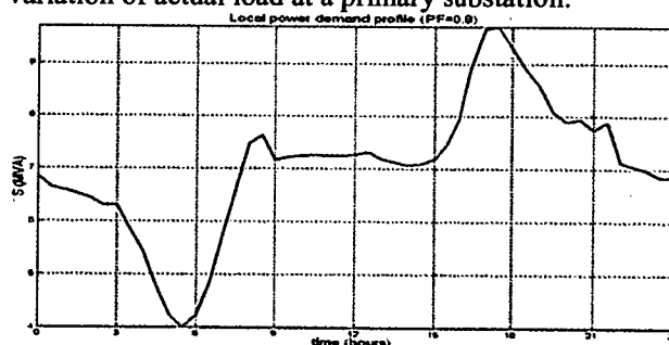
Figure 11 – Local load profile
