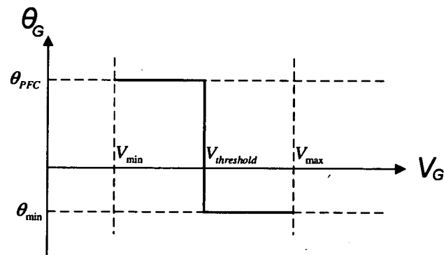
Figure 2. Voltage control strategy of Intelli-Gens.
