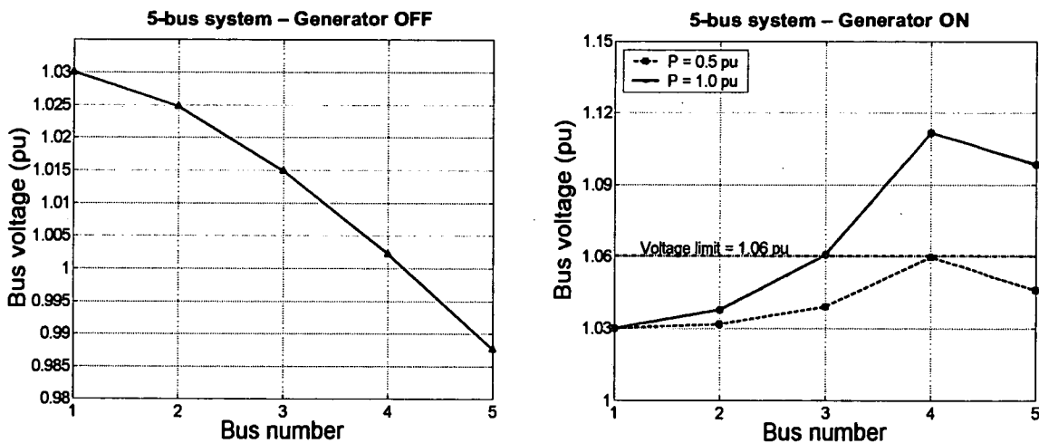
Figure 2: Voltage profile of the 5-bus system with the generator off (a) and on (b)
