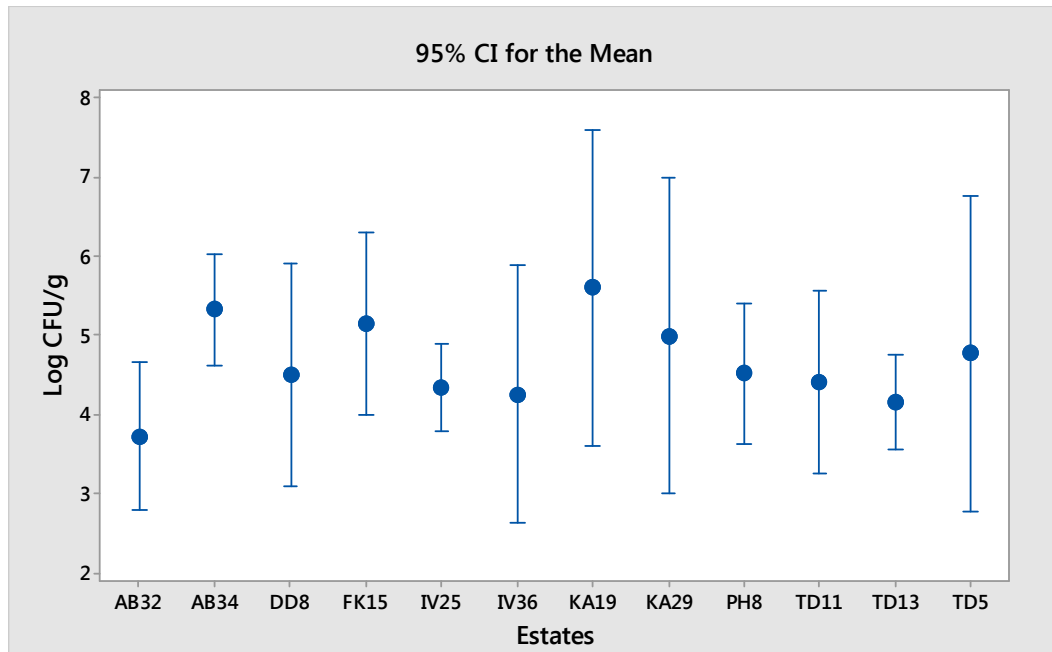
Figure 3.7: Means of Campylobacter load and 95% Confidence Interval (CI) of positive samples by estate expressed as log CFU/g.
