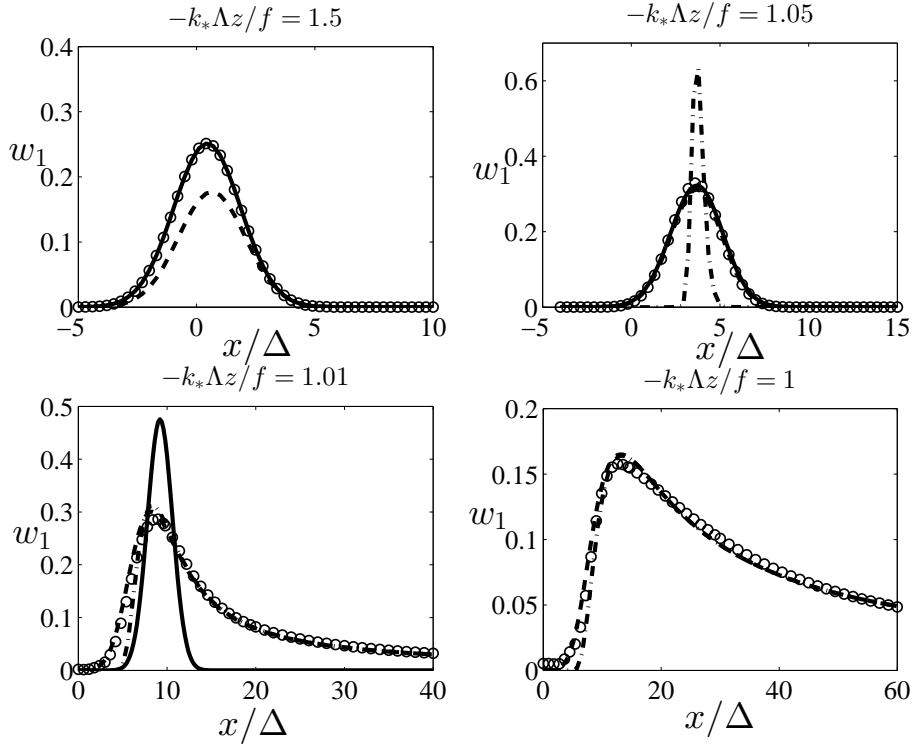
Figure 5.3: (a)–(d) show the amplitude of w normalized by U_b h k_* \Delta / (\sqrt{2\pi} \epsilon) at -k_* \Lambda z / f = 1.5, 1.05, 1.01, 1 corresponding to Regime I, II, II B and dominant inertial level. Here the circles, solid line, dashed line and dot-dashed line denote the direct numerical result, Regime I, II and II B approximations respectively.
