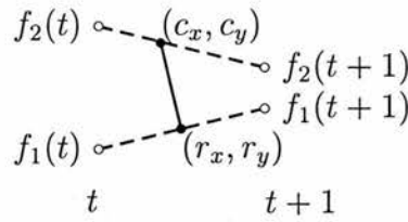
Figure 5.7: Computing the tangential metric
