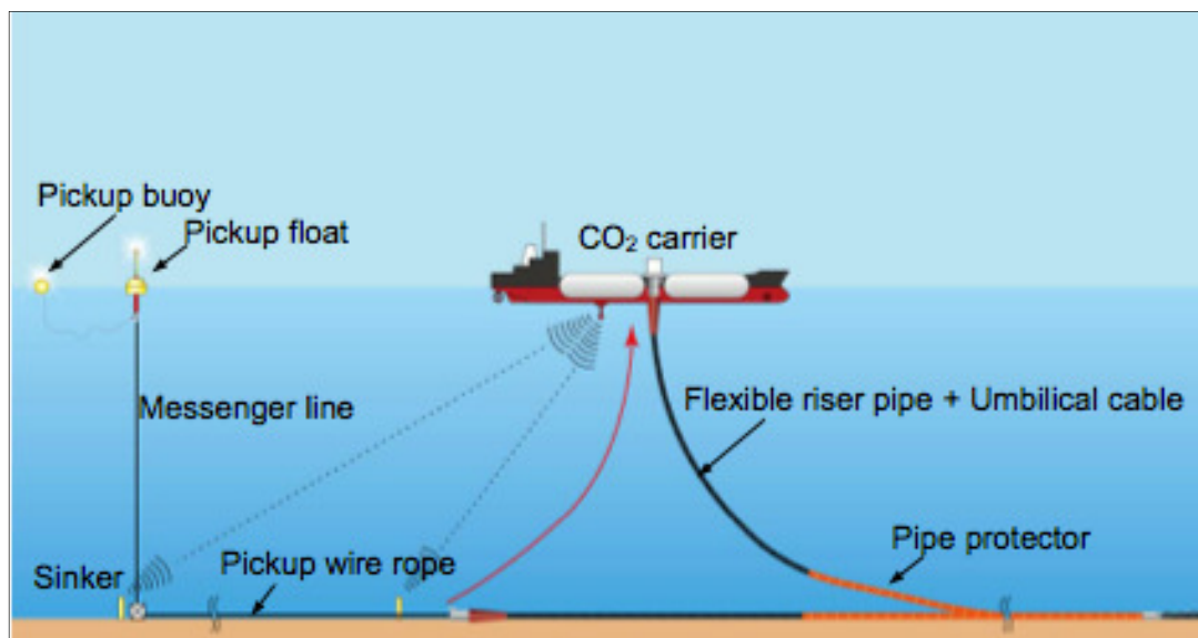
Figure 9. Submerged loading system, subsea injection template not shown (Omata, 2011)
