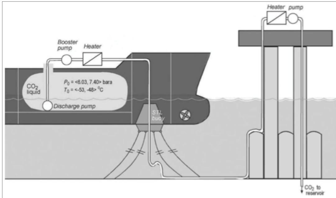
Figure 10. Sketch of submerged turret loading system (Aspelund, Mølnevik and de Koeijer, 2006)
