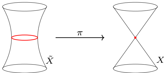
Figure 1.1: The minimal resolution \tilde{X} of the ordinary double point X .
