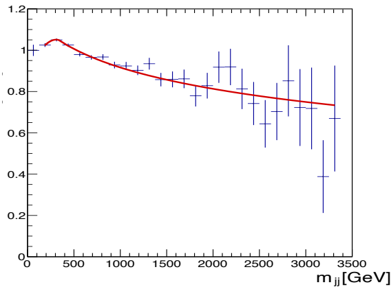
Figure 8.2: Ratio between data and simulation for Z + jet(s) events collected in RR(e \pm e\mp) and RR(\mu \pm \mu\mp) as a function of the dijet invariant mass, with the result of the Novosibirsk fit superimposed. The binning is adjusted to reduce statistical fluctuations.
