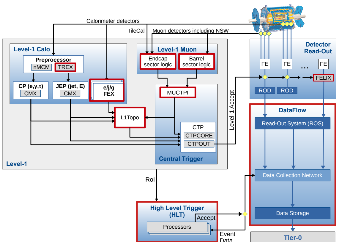
Figure 3.1: Schematic of the ATLAS Trigger and Data Acquisition system with specific focus given to the components of the L1 Trigger system. Run 3 updates (as described in section 2.7) are highlighted in red.
